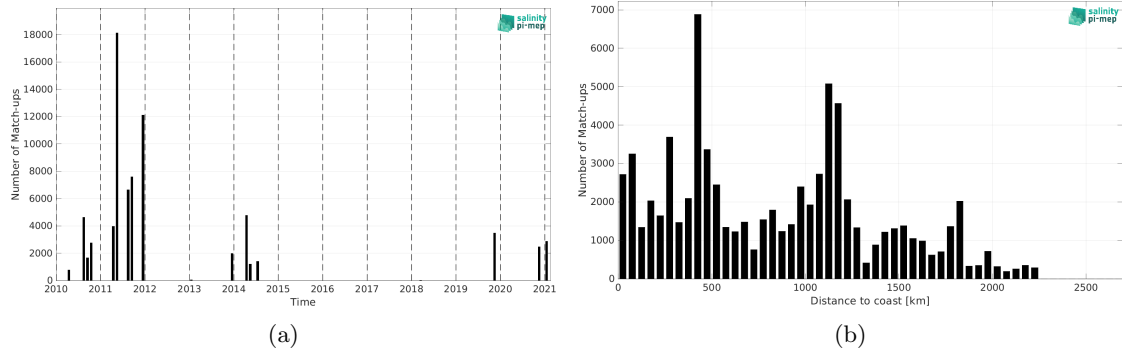
Figure 2: Number of match-ups between TSG (GOSUD-Sailing-ship) and CCI SSS L4 Merged-OI v5.5 - 7-day running (ESA) SSS as a function of time (a) and as function of the distance to coast (b) over the Equatorial Ocean 10N-10S Pi-MEP region and for the full satellite product period.
