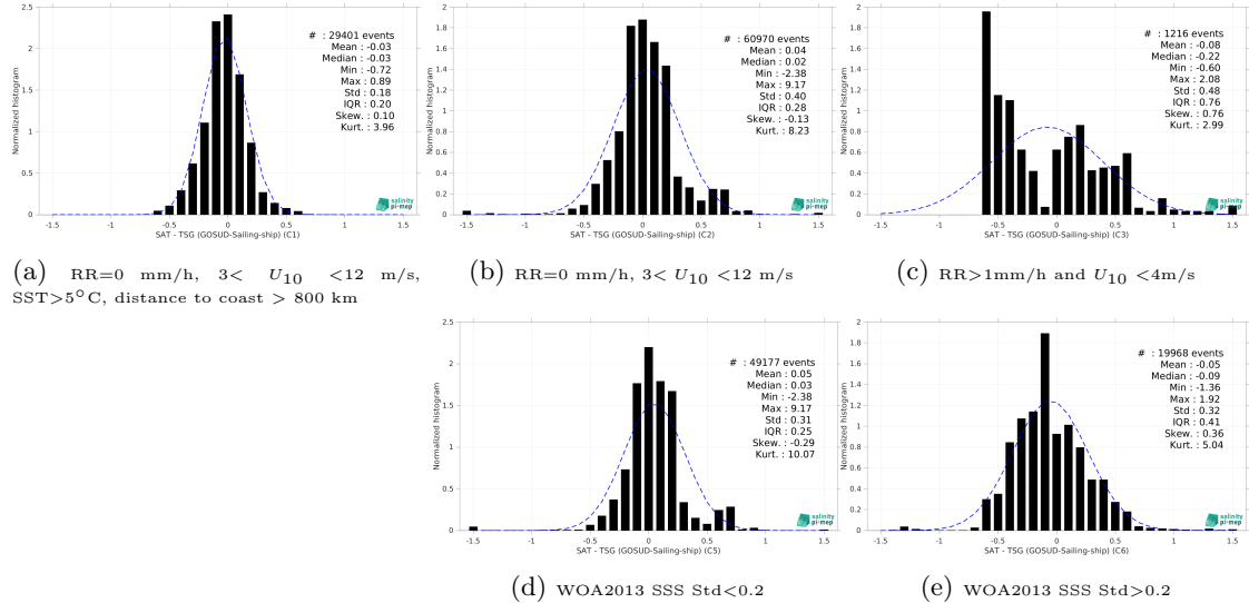
Figure 15: Normalized histogram of \Delta SSS (CCI SSS L4 Merged-OI v5.5 - 7-day running (ESA) - TSG (GOSUD-Sailing-ship)) for 5 different subdatasets corresponding to: RR=0 mm/h, 3 < U_{10} < 12 m/s, SST>5°C, distance to coast > 800 km (a), RR=0 mm/h, 3 < U_{10} < 12 m/s (b), RR>1mm/h and U_{10} < 4 m/s (c), WOA2013 SSS Std<0.2 (d), WOA2013 SSS Std>0.2 (e).
