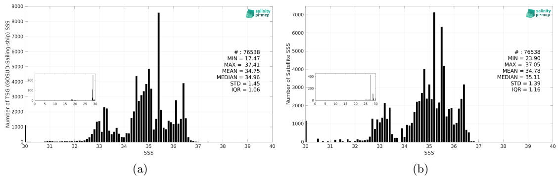
Figure 3: Histograms of SSS from TSG (GOSUD-Sailing-ship) (a) and CCI SSS L4 Merged-OI v5.5 - 7-day running (ESA) (b) considering all match-up pairs per bins of 0.1 over the Equatorial Ocean 10N-10S Pi-MEP region and for the full satellite product period.
