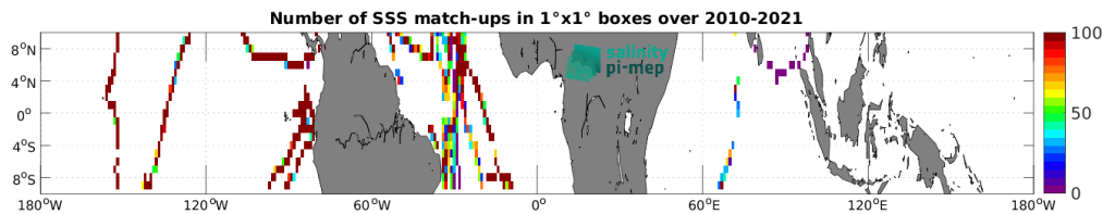
Figure 5: Number of SSS match-ups between TSG (GOSUD-Sailing-ship) SSS and the CCI SSS L4 Merged-OI v5.5 - 7-day running (ESA) SSS product for the Equatorial Ocean 10N-10S Pi-MEP region over 1^\circ \times 1^\circ boxes and for the full satellite product period.
