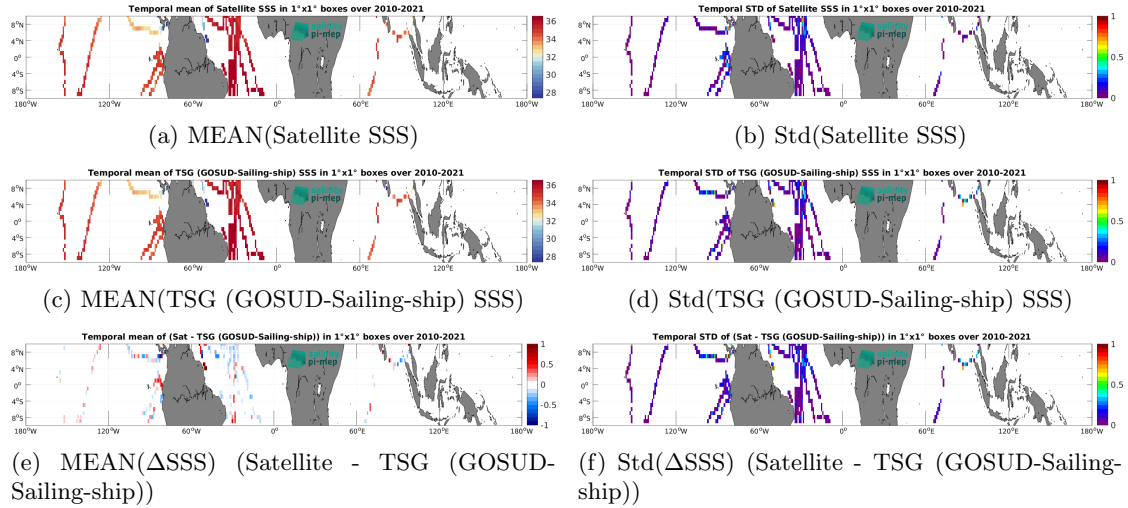
Figure 7: Temporal mean (left) and Std (right) of SSS from CCI SSS L4 Merged-OI v5.5 - 7-day running (ESA) (top), TSG (GOSUD-Sailing-ship) (middle), and of \Delta SSS (Satellite - TSG (GOSUD-Sailing-ship)). Only match-up pairs are used to generate these maps.
