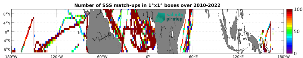
Figure 5: Number of SSS match-ups between TSG (GOSUD-Research-vessel) SSS and the CCI SSS L4 Merged-OI v5.5 - 7-day running (ESA) SSS product for the Equatorial Ocean 10N-10S Pi-MEP region over 1^\circ \times 1^\circ boxes and for the full satellite product period.
