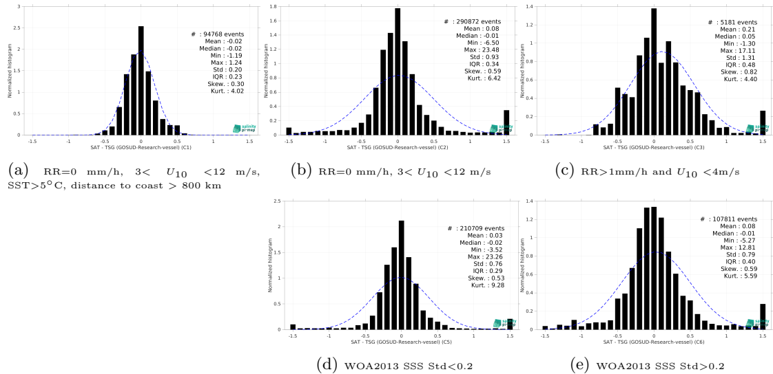
Figure 15: Normalized histogram of \Delta\text{SSS} (CCI SSS L4 Merged-OI v5.5 - 7-day running (ESA) - TSG (GOSUD-Research-vessel)) for 5 different subdatasets corresponding to: RR=0 mm/h, 3 < U_{10} < 12 m/s, SST>5°C, distance to coast > 800 km (a), RR=0 mm/h, 3 < U_{10} < 12 m/s (b), RR>1mm/h and U_{10} < 4 m/s (c), WOA2013 SSS Std<0.2 (d), WOA2013 SSS Std>0.2 (e).
