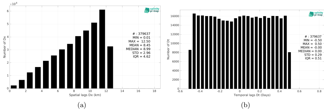
Figure 6: Histograms of the spatial (a) and temporal (b) lags between the location/time of the TSG (GOSUD-Research-vessel) measurement and the date of the corresponding CCI SSS L4 Merged-OI v5.5 - 7-day running (ESA) SSS pixel.
