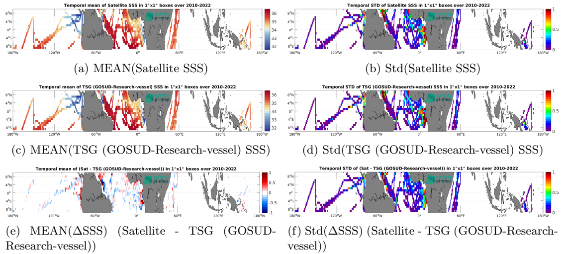
Figure 7: Temporal mean (left) and Std (right) of SSS from CCI SSS L4 Merged-OI v5.5 - 7-day running (ESA) (top), TSG (GOSUD-Research-vessel) (middle), and of \Delta SSS (Satellite - TSG (GOSUD-Research-vessel)). Only match-up pairs are used to generate these maps.
