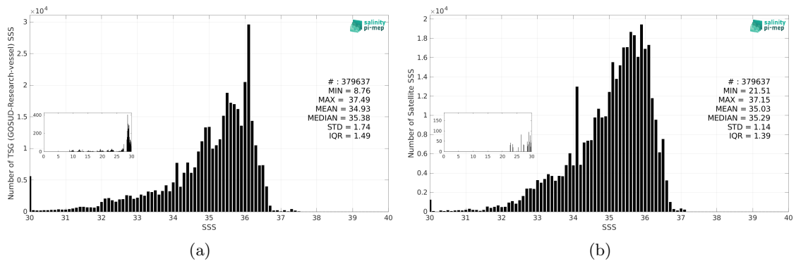
Figure 3: Histograms of SSS from TSG (GOSUD-Research-vessel) (a) and CCI SSS L4 Merged-OI v5.5 - 7-day running (ESA) (b) considering all match-up pairs per bins of 0.1 over the Equatorial Ocean 10N-10S Pi-MEP region and for the full satellite product period.
