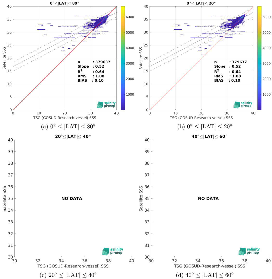
Figure 10: Contour maps of the concentration of CCI SSS L4 Merged-OI v5.5 - 7-day running (ESA) SSS (y-axis) versus TSG (GOSUD-Research-vessel) SSS (x-axis) at match-up pairs for different latitude bands. For each plot, the red line shows x=y . The black thin and dashed lines indicate a linear fit through the data cloud and the \pm 95\% confidence levels, respectively. The number match-up pairs n , the slope and R^2 coefficient of the linear fit, the root mean square (RMS) and the mean bias between satellite and in situ data are indicated for each latitude band in each plots.
