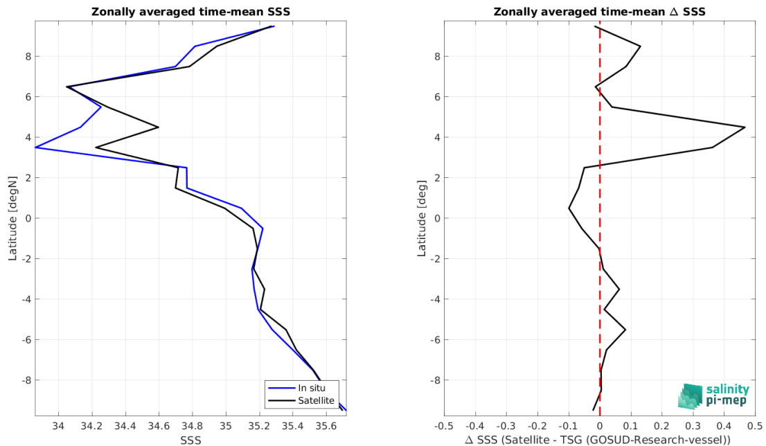
Figure 9: Left panel: Zonal mean SSS from CCI SSS L4 Merged-OI v5.5 - 7-day running (ESA) satellite product (black) and from TSG (GOSUD-Research-vessel) (blue). Right panel: Zonal mean of \Delta SSS (Satellite - TSG (GOSUD-Research-vessel)) for all the collected Pi-MEP match-up pairs estimated over the full satellite product period.
