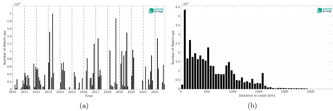
Figure 2: Number of match-ups between TSG (GOSUD-Research-vessel) and CCI SSS L4 Merged-OI v5.5 - 7-day running (ESA) SSS as a function of time (a) and as function of the distance to coast (b) over the Equatorial Ocean 10N-10S Pi-MEP region and for the full satellite product period.
