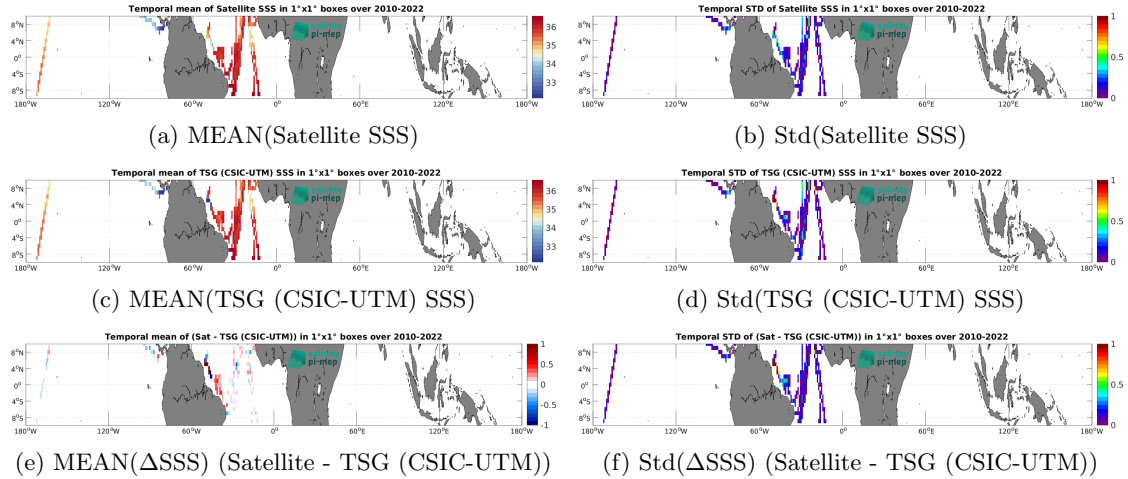
Figure 7: Temporal mean (left) and Std (right) of SSS from CCI SSS L4 Merged-OI v5.5 - 7-day running (ESA) (top), TSG (CSIC-UTM) (middle), and of \Delta SSS (Satellite - TSG (CSIC-UTM)). Only match-up pairs are used to generate these maps.
