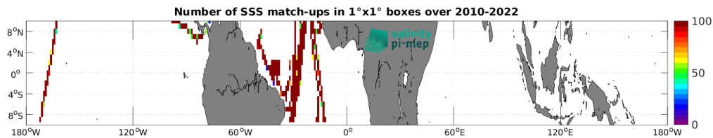
Figure 5: Number of SSS match-ups between TSG (CSIC-UTM) SSS and the CCI SSS L4 Merged-OI v5.5 - 7-day running (ESA) SSS product for the Equatorial Ocean 10N-10S Pi-MEP region over 1^\circ \times 1^\circ boxes and for the full satellite product period.
