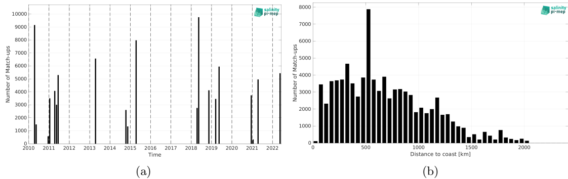
Figure 2: Number of match-ups between TSG (CSIC-UTM) and CCI SSS L4 Merged-OI v5.5 - 7-day running (ESA) SSS as a function of time (a) and as function of the distance to coast (b) over the Equatorial Ocean 10N-10S Pi-MEP region and for the full satellite product period.
