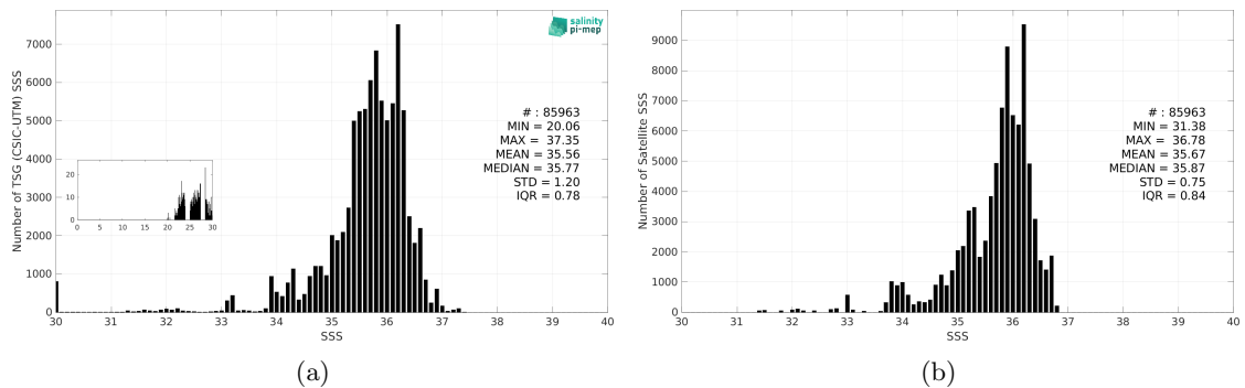
Figure 3: Histograms of SSS from TSG (CSIC-UTM) (a) and CCI SSS L4 Merged-OI v5.5 - 7-day running (ESA) (b) considering all match-up pairs per bins of 0.1 over the Equatorial Ocean 10N-10S Pi-MEP region and for the full satellite product period.
