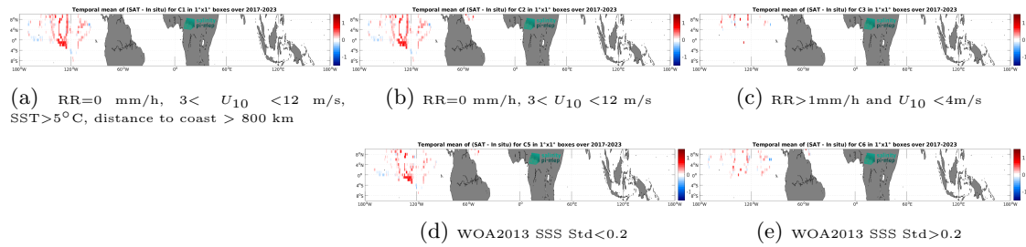
Figure 14: Temporal mean gridded over spatial boxes of size 1^\circ \times 1^\circ of \Delta SSS (CCI SSS L4 Merged-OI v5.5 - 7-day running (ESA) - Sailydrone) for 5 different subdatasets corresponding to:RR=0 mm/h, 3 < U_{10} < 12 m/s, SST>5°C, distance to coast > 800 km (a), RR=0 mm/h, 3 < U_{10} < 12 m/s (b), RR>1mm/h and U_{10} < 4 m/s (c), WOA2013 SSS Std<0.2 (d), WOA2013 SSS Std>0.2 (e).
