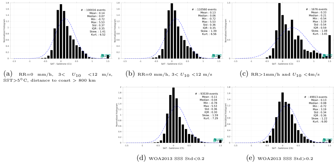
Figure 15: Normalized histogram of \Delta SSS (CCI SSS L4 Merged-OI v5.5 - 7-day running (ESA) - Sailydrone) for 5 different subdatasets corresponding to: RR=0 mm/h, 3 < U_{10} < 12 m/s, SST>5°C, distance to coast > 800 km (a), RR=0 mm/h, 3 < U_{10} < 12 m/s (b), RR>1mm/h and U_{10} < 4 m/s (c), WOA2013 SSS Std<0.2 (d), WOA2013 SSS Std>0.2 (e).
