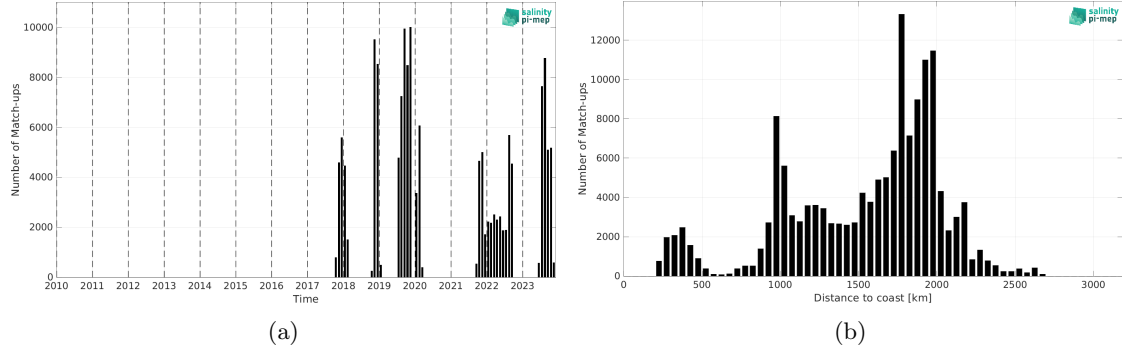
Figure 2: Number of match-ups between Saildrone and CCI SSS L4 Merged-OI v5.5 - 7-day running (ESA) SSS as a function of time (a) and as function of the distance to coast (b) over the Equatorial Ocean 10N-10S Pi-MEP region and for the full satellite product period.
