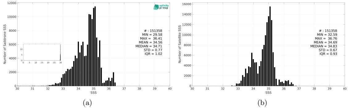
Figure 3: Histograms of SSS from Saildrone (a) and CCI SSS L4 Merged-OI v5.5 - 7-day running (ESA) (b) considering all match-up pairs per bins of 0.1 over the Equatorial Ocean 10N-10S Pi-MEP region and for the full satellite product period.
