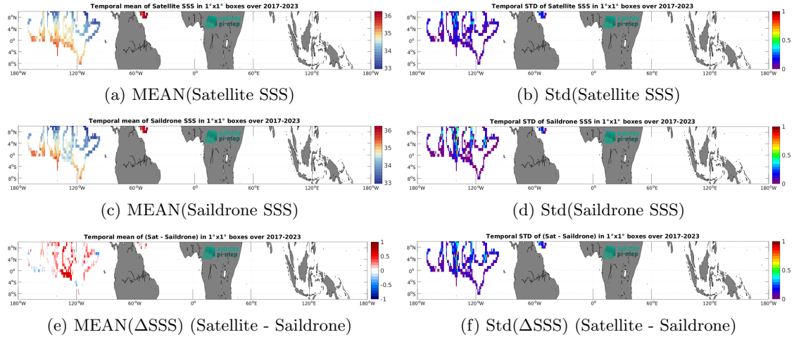
Figure 7: Temporal mean (left) and Std (right) of SSS from CCI SSS L4 Merged-OI v5.5 - 7-day running (ESA) (top), Saildrone (middle), and of \Delta SSS (Satellite - Saildrone). Only match-up pairs are used to generate these maps.
