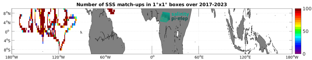
Figure 5: Number of SSS match-ups between Saildrone SSS and the CCI SSS L4 Merged-OI v5.5 - 7-day running (ESA) SSS product for the Equatorial Ocean 10N-10S Pi-MEP region over 1^\circ \times 1^\circ boxes and for the full satellite product period.
