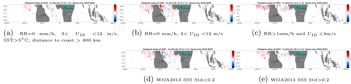
Figure 13: Temporal mean gridded over spatial boxes of size 1^\circ \times 1^\circ of \Delta SSS (CCI SSS L4 Merged-OI v5.5 - 7-day running (ESA) - Surface drifters) for 5 different subdatasets corresponding to:RR=0 mm/h, 3 < U_{10} < 12 m/s, SST >5^\circ\text{C} , distance to coast > 800 km (a), RR=0 mm/h, 3 < U_{10} < 12 m/s (b), RR >1 mm/h and U_{10} < 4 m/s (c), WOA2013 SSS Std <0.2 (d), WOA2013 SSS Std >0.2 (e).
