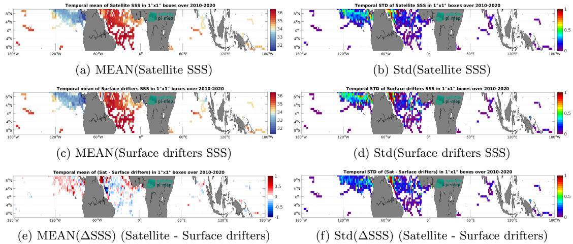
Figure 6: Temporal mean (left) and Std (right) of SSS from CCI SSS L4 Merged-OI v5.5 - 7-day running (ESA) (top), Surface drifters (middle), and of \Delta SSS (Satellite - Surface drifters). Only match-up pairs are used to generate these maps.
