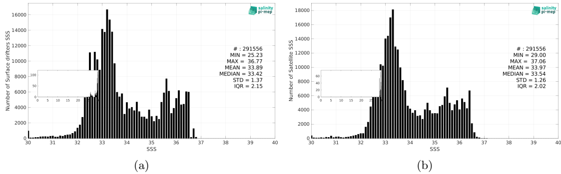
Figure 3: Histograms of SSS from Surface drifters (a) and CCI SSS L4 Merged-OI v5.5 - 7-day running (ESA) (b) considering all match-up pairs per bins of 0.1 over the Equatorial Ocean 10N-10S Pi-MEP region and for the full satellite product period.
