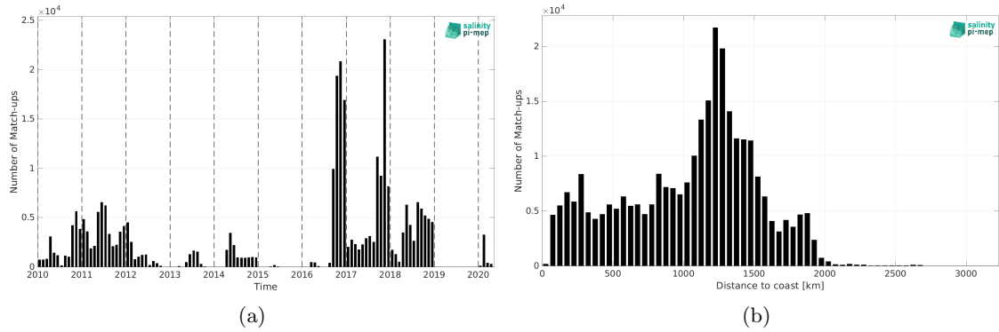
Figure 2: Number of match-ups between Surface drifters and CCI SSS L4 Merged-OI v5.5 - 7-day running (ESA) SSS as a function of time (a) and as function of the distance to coast (b) over the Equatorial Ocean 10N-10S Pi-MEP region and for the full satellite product period.
