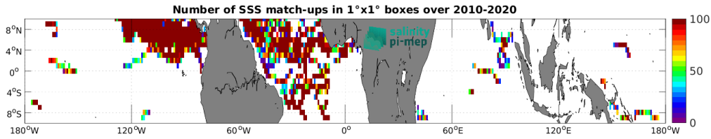
Figure 4: Number of SSS match-ups between Surface drifters SSS and the CCI SSS L4 Merged-OI v5.5 - 7-day running (ESA) SSS product for the Equatorial Ocean 10N-10S Pi-MEP region over 1^\circ \times 1^\circ boxes and for the full satellite product period.
