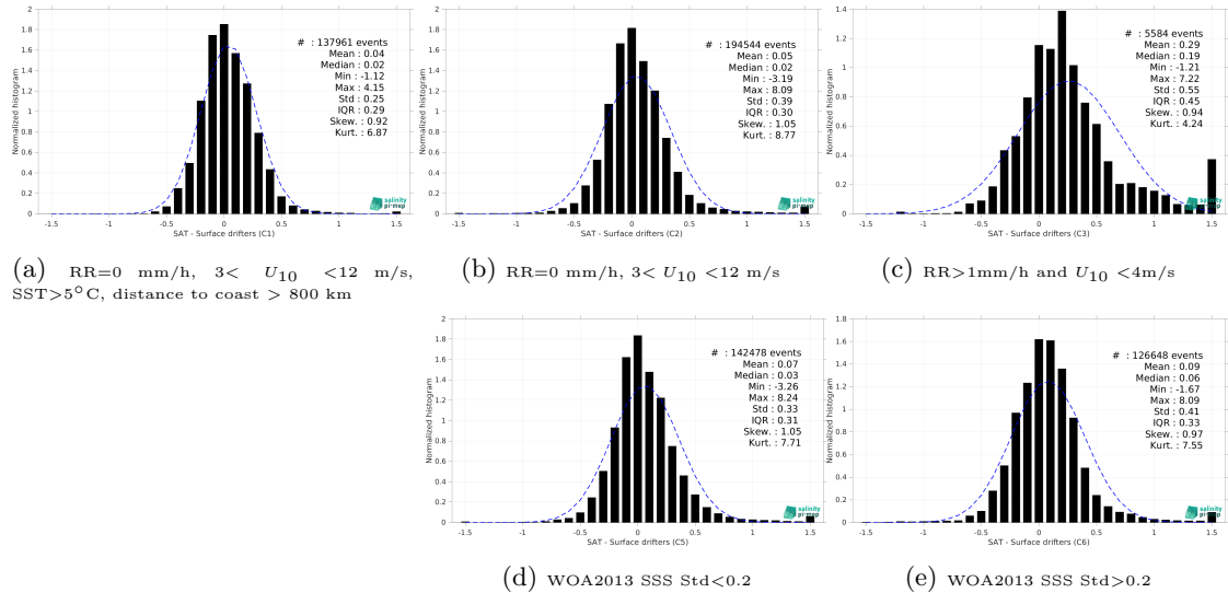
Figure 14: Normalized histogram of \Delta SSS (CCI SSS L4 Merged-OI v5.5 - 7-day running (ESA) - Surface drifters) for 5 different subdatasets corresponding to: RR=0 mm/h, 3 < U_{10} < 12 m/s, SST >5^\circ\text{C} , distance to coast > 800 km (a), RR=0 mm/h, 3 < U_{10} < 12 m/s (b), RR >1 mm/h and U_{10} < 4 m/s (c), WOA2013 SSS Std <0.2 (d), WOA2013 SSS Std >0.2 (e).
