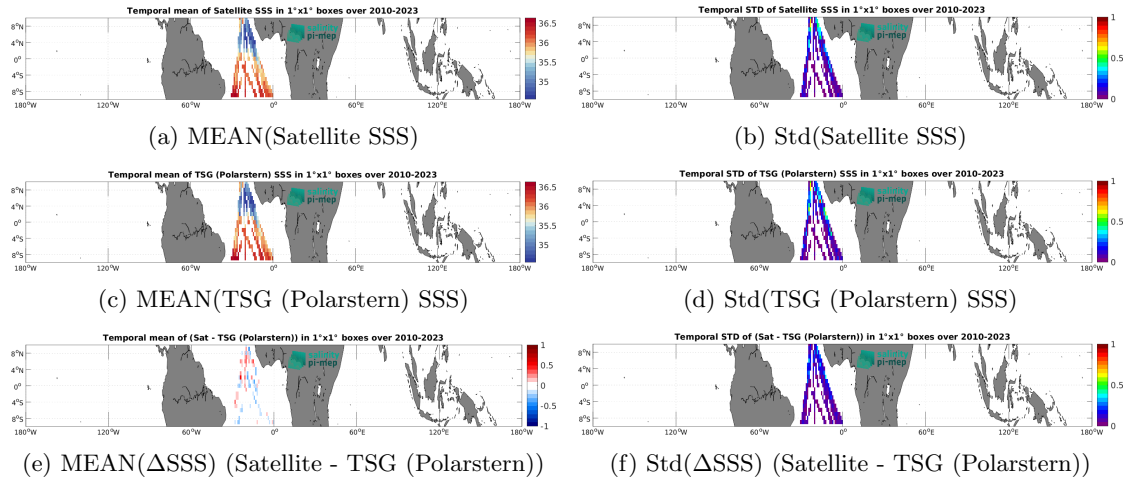
Figure 7: Temporal mean (left) and Std (right) of SSS from CCI SSS L4 Merged-OI v5.5 - 30-day running (ESA) (top), TSG (Polarstern) (middle), and of \Delta SSS (Satellite - TSG (Polarstern)). Only match-up pairs are used to generate these maps.
