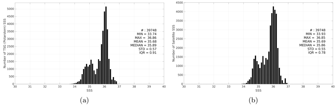
Figure 3: Histograms of SSS from TSG (Polarstern) (a) and CCI SSS L4 Merged-OI v5.5 - 30-day running (ESA) (b) considering all match-up pairs per bins of 0.1 over the Equatorial Ocean 10N-10S Pi-MEP region and for the full satellite product period.
