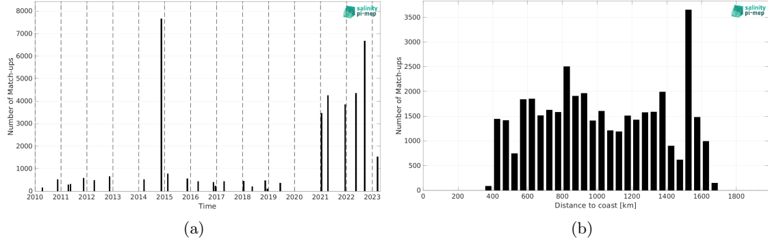
Figure 2: Number of match-ups between TSG (Polarstern) and CCI SSS L4 Merged-OI v5.5 - 30-day running (ESA) SSS as a function of time (a) and as function of the distance to coast (b) over the Equatorial Ocean 10N-10S Pi-MEP region and for the full satellite product period.
