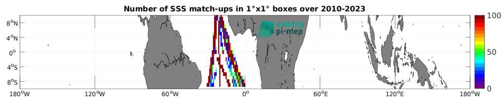
Figure 5: Number of SSS match-ups between TSG (Polarstern) SSS and the CCI SSS L4 Merged-OI v5.5 - 30-day running (ESA) SSS product for the Equatorial Ocean 10N-10S Pi-MEP region over 1^\circ \times 1^\circ boxes and for the full satellite product period.
