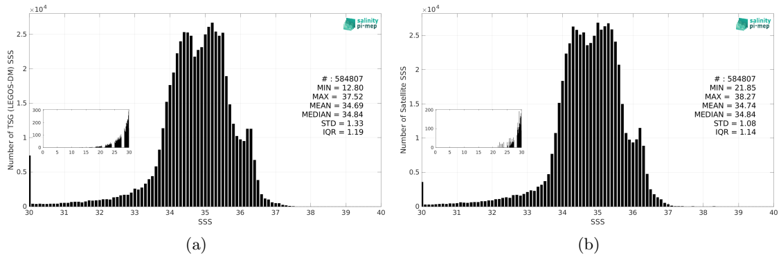
Figure 3: Histograms of SSS from TSG (LEGOS-DM) (a) and CCI SSS L4 Merged-OI v5.5 - 30-day running (ESA) (b) considering all match-up pairs per bins of 0.1 over the Equatorial Ocean 10N-10S Pi-MEP region and for the full satellite product period.
