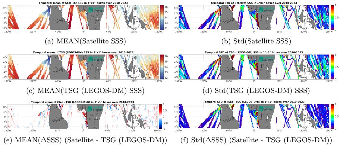
Figure 7: Temporal mean (left) and Std (right) of SSS from CCI SSS L4 Merged-OI v5.5 - 30-day running (ESA) (top), TSG (LEGOS-DM) (middle), and of \Delta SSS (Satellite - TSG (LEGOS-DM)). Only match-up pairs are used to generate these maps.
