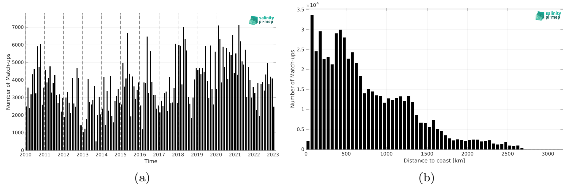
Figure 2: Number of match-ups between TSG (LEGOS-DM) and CCI SSS L4 Merged-OI v5.5 - 30-day running (ESA) SSS as a function of time (a) and as function of the distance to coast (b) over the Equatorial Ocean 10N-10S Pi-MEP region and for the full satellite product period.
