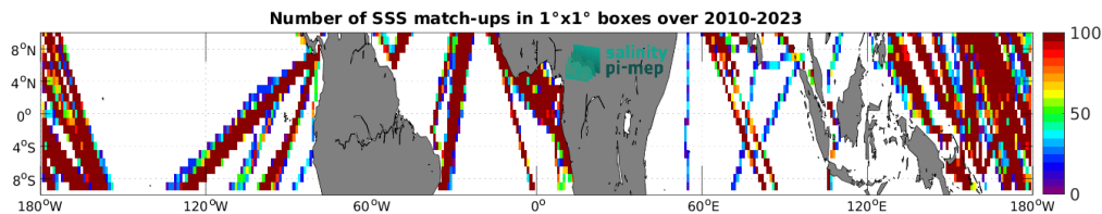
Figure 5: Number of SSS match-ups between TSG (LEGOS-DM) SSS and the CCI SSS L4 Merged-OI v5.5 - 30-day running (ESA) SSS product for the Equatorial Ocean 10N-10S Pi-MEP region over 1^\circ \times 1^\circ boxes and for the full satellite product period.
