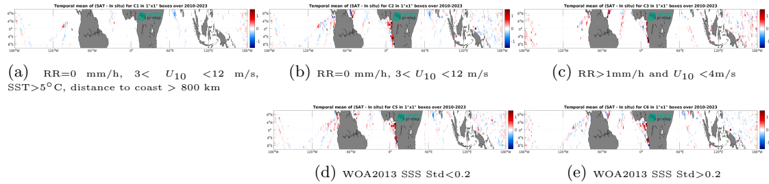
Figure 14: Temporal mean gridded over spatial boxes of size 1^\circ \times 1^\circ of \Delta\text{SSS} (CCI SSS L4 Merged-OI v5.5 - 30-day running (ESA) - TSG (LEGOS-DM)) for 5 different subdatasets corresponding to: RR=0 mm/h, 3 < U_{10} < 12 m/s, SST>5°C, distance to coast > 800 km (a), RR=0 mm/h, 3 < U_{10} < 12 m/s (b), RR>1mm/h and U_{10} < 4 m/s (c), WOA2013 SSS Std<0.2 (d), WOA2013 SSS Std>0.2 (e).
