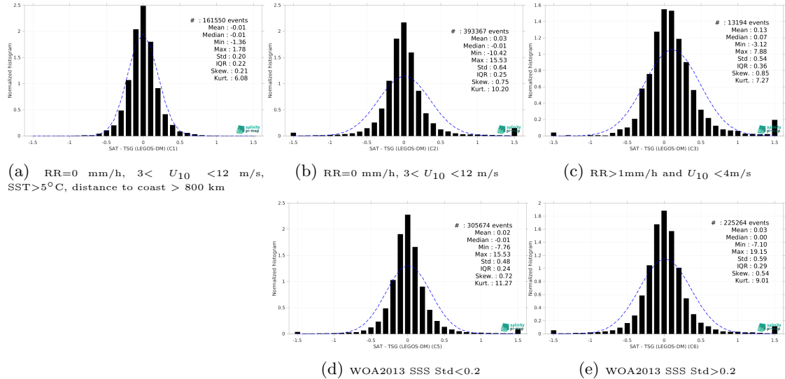
Figure 15: Normalized histogram of \Delta\text{SSS} (CCI SSS L4 Merged-OI v5.5 - 30-day running (ESA) - TSG (LEGOS-DM)) for 5 different subdatasets corresponding to: RR=0 mm/h, 3 < U_{10} < 12 m/s, SST>5°C, distance to coast > 800 km (a), RR=0 mm/h, 3 < U_{10} < 12 m/s (b), RR>1mm/h and U_{10} < 4 m/s (c), WOA2013 SSS Std<0.2 (d), WOA2013 SSS Std>0.2 (e).
