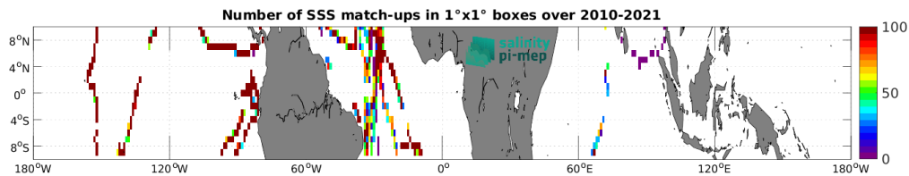
Figure 5: Number of SSS match-ups between TSG (GOSUD-Sailing-ship) SSS and the CCI SSS L4 Merged-OI v5.5 - 30-day running (ESA) SSS product for the Equatorial Ocean 10N-10S Pi-MEP region over 1^\circ \times 1^\circ boxes and for the full satellite product period.
