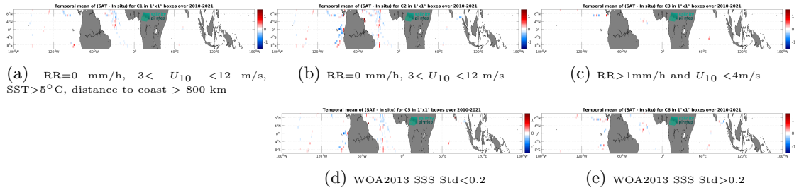
Figure 14: Temporal mean gridded over spatial boxes of size 1^\circ \times 1^\circ of \Delta SSS (CCI SSS L4 Merged-OI v5.5 - 30-day running (ESA) - TSG (GOSUD-Sailing-ship)) for 5 different subdatasets corresponding to:RR=0 mm/h, 3 < U_{10} < 12 m/s, SST >5^\circ\text{C} , distance to coast > 800 km (a), RR=0 mm/h, 3 < U_{10} < 12 m/s (b), RR >1 mm/h and U_{10} < 4 m/s (c), WOA2013 SSS Std <0.2 (d), WOA2013 SSS Std >0.2 (e).
