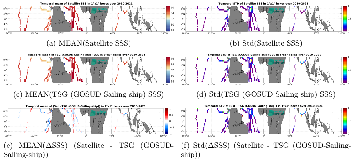
Figure 7: Temporal mean (left) and Std (right) of SSS from CCI SSS L4 Merged-OI v5.5 - 30-day running (ESA) (top), TSG (GOSUD-Sailing-ship) (middle), and of \Delta SSS (Satellite - TSG (GOSUD-Sailing-ship)). Only match-up pairs are used to generate these maps.
