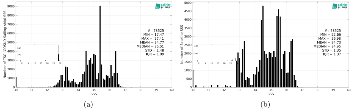
Figure 3: Histograms of SSS from TSG (GOSUD-Sailing-ship) (a) and CCI SSS L4 Merged-OI v5.5 - 30-day running (ESA) (b) considering all match-up pairs per bins of 0.1 over the Equatorial Ocean 10N-10S Pi-MEP region and for the full satellite product period.
