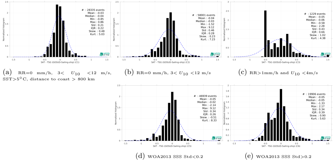
Figure 15: Normalized histogram of \Delta SSS (CCI SSS L4 Merged-OI v5.5 - 30-day running (ESA) - TSG (GOSUD-Sailing-ship)) for 5 different subdatasets corresponding to: RR=0 mm/h, 3 < U_{10} < 12 m/s, SST >5^\circ\text{C} , distance to coast > 800 km (a), RR=0 mm/h, 3 < U_{10} < 12 m/s (b), RR >1 mm/h and U_{10} < 4 m/s (c), WOA2013 SSS Std <0.2 (d), WOA2013 SSS Std >0.2 (e).
