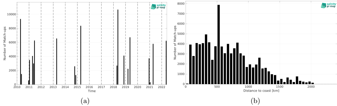
Figure 2: Number of match-ups between TSG (CSIC-UTM) and CCI SSS L4 Merged-OI v5.5 - 30-day running (ESA) SSS as a function of time (a) and as function of the distance to coast (b) over the Equatorial Ocean 10N-10S Pi-MEP region and for the full satellite product period.
