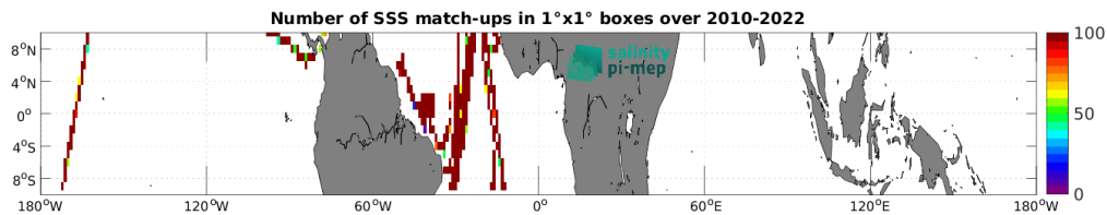
Figure 5: Number of SSS match-ups between TSG (CSIC-UTM) SSS and the CCI SSS L4 Merged-OI v5.5 - 30-day running (ESA) SSS product for the Equatorial Ocean 10N-10S Pi-MEP region over 1^\circ \times 1^\circ boxes and for the full satellite product period.
