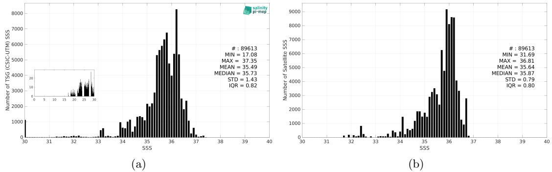
Figure 3: Histograms of SSS from TSG (CSIC-UTM) (a) and CCI SSS L4 Merged-OI v5.5 - 30-day running (ESA) (b) considering all match-up pairs per bins of 0.1 over the Equatorial Ocean 10N-10S Pi-MEP region and for the full satellite product period.
