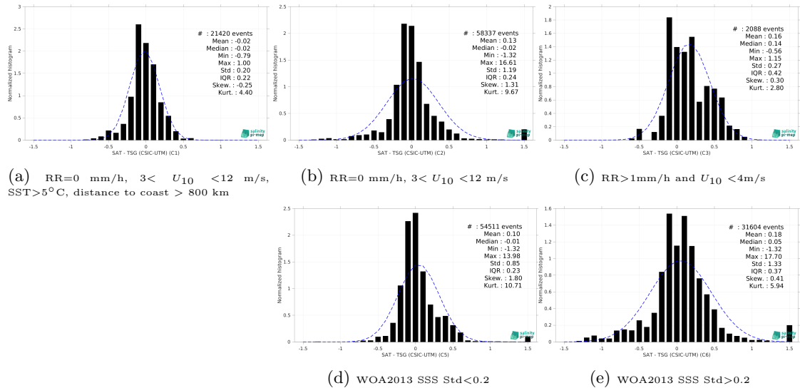
Figure 15: Normalized histogram of \Delta\text{SSS} (CCI SSS L4 Merged-OI v5.5 - 30-day running (ESA) - TSG (CSIC-UTM)) for 5 different subdatasets corresponding to: RR=0 mm/h, 3 < U_{10} < 12 m/s, SST>5°C, distance to coast > 800 km (a), RR=0 mm/h, 3 < U_{10} < 12 m/s (b), RR>1mm/h and U_{10} < 4 m/s (c), WOA2013 SSS Std<0.2 (d), WOA2013 SSS Std>0.2 (e).
