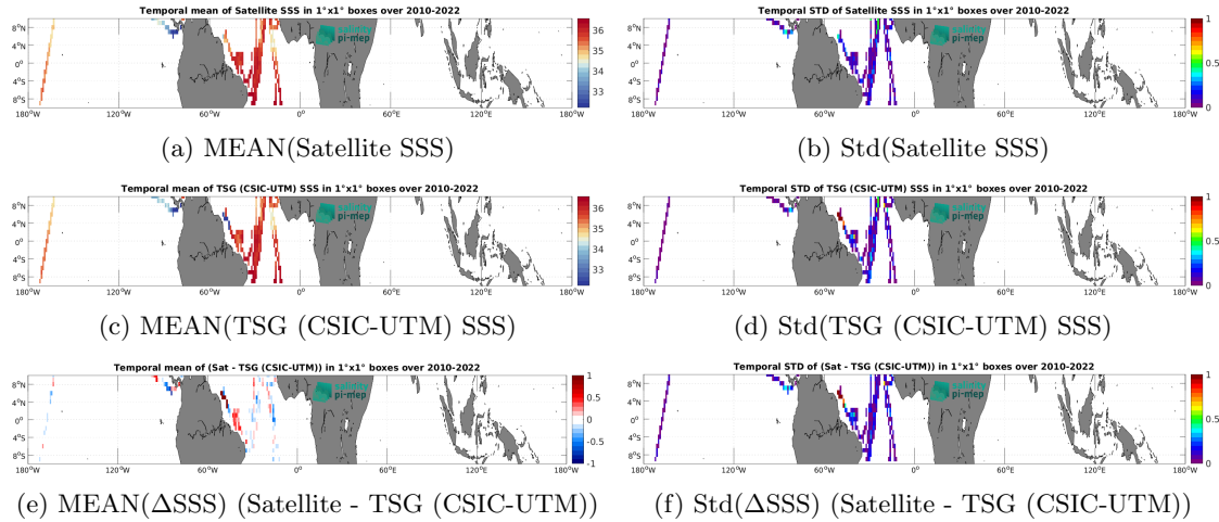
Figure 7: Temporal mean (left) and Std (right) of SSS from CCI SSS L4 Merged-OI v5.5 - 30-day running (ESA) (top), TSG (CSIC-UTM) (middle), and of \Delta SSS (Satellite - TSG (CSIC-UTM)). Only match-up pairs are used to generate these maps.
