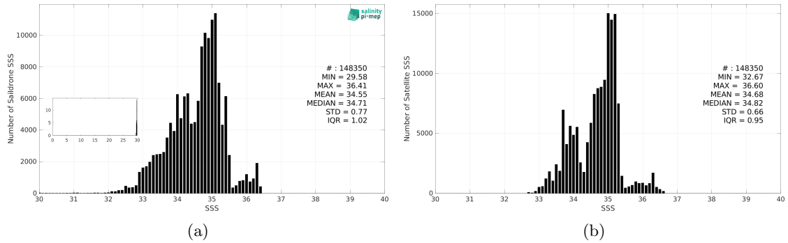
Figure 3: Histograms of SSS from Saildrone (a) and CCI SSS L4 Merged-OI v5.5 - 30-day running (ESA) (b) considering all match-up pairs per bins of 0.1 over the Equatorial Ocean 10N-10S Pi-MEP region and for the full satellite product period.
