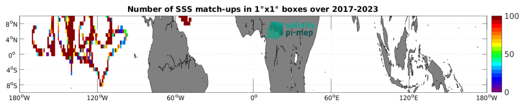
Figure 5: Number of SSS match-ups between Saildrone SSS and the CCI SSS L4 Merged-OI v5.5 - 30-day running (ESA) SSS product for the Equatorial Ocean 10N-10S Pi-MEP region over 1^\circ \times 1^\circ boxes and for the full satellite product period.
