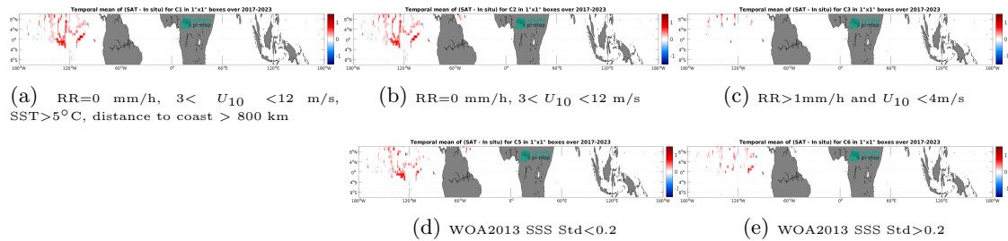
Figure 14: Temporal mean gridded over spatial boxes of size 1^\circ \times 1^\circ of \Delta SSS (CCI SSS L4 Merged-OI v5.5 - 30-day running (ESA) - Saildrone) for 5 different subdatasets corresponding to: RR=0 mm/h, 3 < U_{10} < 12 m/s, SST>5°C, distance to coast > 800 km (a), RR=0 mm/h, 3 < U_{10} < 12 m/s (b), RR>1mm/h and U_{10} < 4 m/s (c), WOA2013 SSS Std<0.2 (d), WOA2013 SSS Std>0.2 (e).
