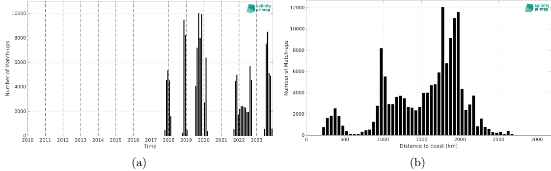
Figure 2: Number of match-ups between Saildrone and CCI SSS L4 Merged-OI v5.5 - 30-day running (ESA) SSS as a function of time (a) and as function of the distance to coast (b) over the Equatorial Ocean 10N-10S Pi-MEP region and for the full satellite product period.
