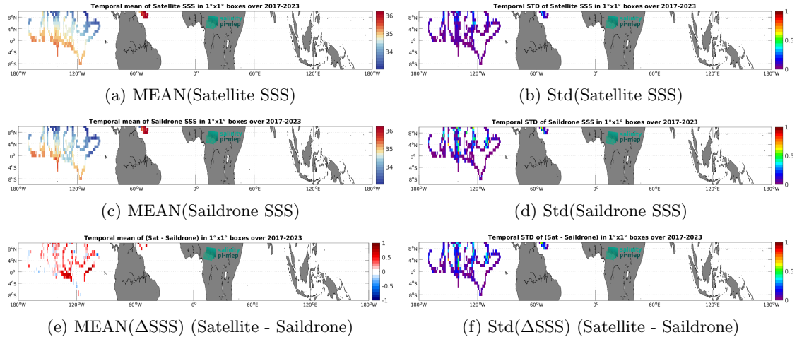
Figure 7: Temporal mean (left) and Std (right) of SSS from CCI SSS L4 Merged-OI v5.5 - 30-day running (ESA) (top), Saildrone (middle), and of \Delta SSS (Satellite - Saildrone). Only match-up pairs are used to generate these maps.
