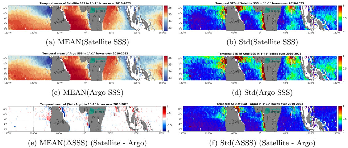
Figure 7: Temporal mean (left) and Std (right) of SSS from CCI SSS L4 Merged-OI v5.5 - 30-day running (ESA) (top), Argo (middle), and of \Delta SSS (Satellite - Argo). Only match-up pairs are used to generate these maps.
