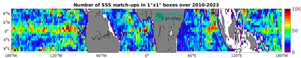
Figure 5: Number of SSS match-ups between Argo SSS and the CCI SSS L4 Merged-OI v5.5 - 30-day running (ESA) SSS product for the Equatorial Ocean 10N-10S Pi-MEP region over 1^\circ \times 1^\circ boxes and for the full satellite product period.
