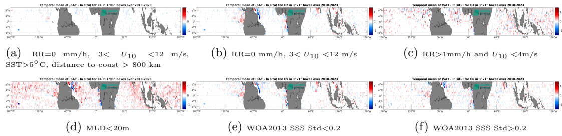
Figure 14: Temporal mean gridded over spatial boxes of size 1^\circ \times 1^\circ of \Delta SSS (CCI SSS L4 Merged-OI v5.5 - 30-day running (ESA) - Argo) for 6 different subdatasets corresponding to:RR=0 mm/h, 3 < U_{10} < 12 m/s, SST >5^\circ\text{C} , distance to coast > 800 km (a), RR=0 mm/h, 3 < U_{10} < 12 m/s (b), RR >1 mm/h and U_{10} < 4 m/s (c),MLD <20 m (d),WOA2013 SSS Std <0.2 (e),WOA2013 SSS Std >0.2 (f).
