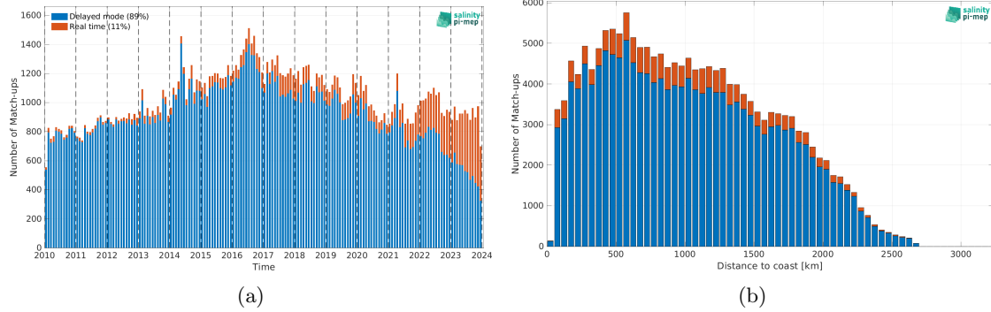
Figure 2: Number of match-ups between Argo and CCI SSS L4 Merged-OI v5.5 - 30-day running (ESA) SSS as a function of time (a) and as function of the distance to coast (b) over the Equatorial Ocean 10N-10S Pi-MEP region and for the full satellite product period.
