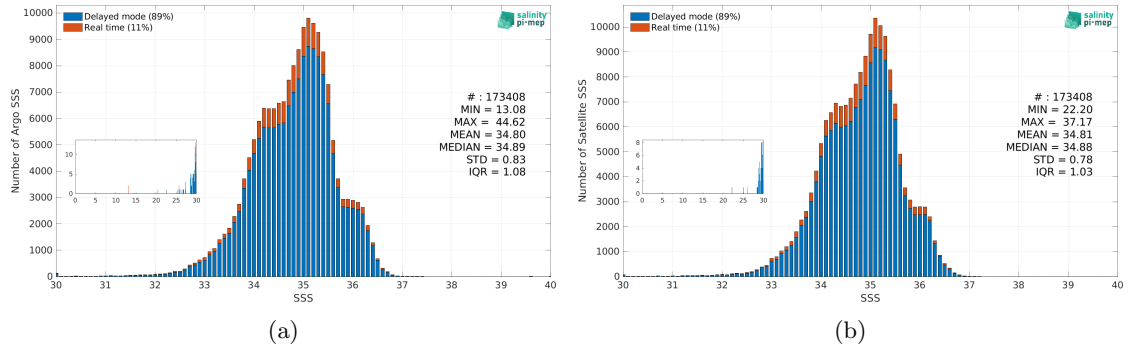
Figure 3: Histograms of SSS from Argo (a) and CCI SSS L4 Merged-OI v5.5 - 30-day running (ESA) (b) considering all match-up pairs per bins of 0.1 over the Equatorial Ocean 10N-10S Pi-MEP region and for the full satellite product period.
