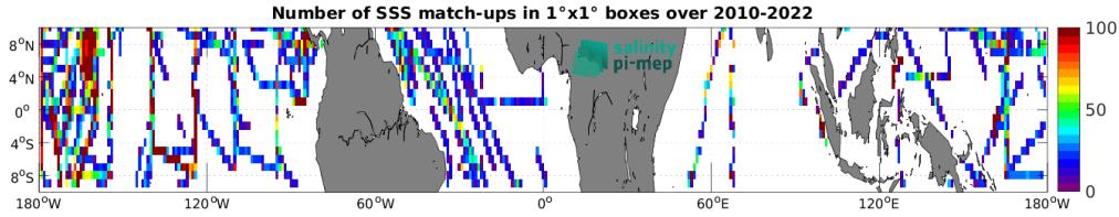
Figure 5: Number of SSS match-ups between TSG (SAMOS) SSS and the CCI SSS L4 Merged-OI v4.41 - 7-day running (ESA) SSS product for the Equatorial Ocean 10N-10S Pi-MEP region over 1^\circ \times 1^\circ boxes and for the full satellite product period.
