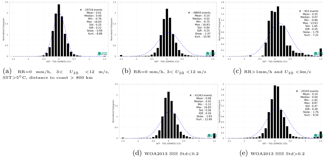
Figure 15: Normalized histogram of \Delta\text{SSS} (CCI SSS L4 Merged-OI v4.41 - 7-day running (ESA) - TSG (SAMOS)) for 5 different subdatasets corresponding to: RR=0 mm/h, 3 < U_{10} < 12 m/s, SST> 5^\circ\text{C} , distance to coast > 800 km (a), RR=0 mm/h, 3 < U_{10} < 12 m/s (b), RR>1mm/h and U_{10} < 4 m/s (c), WOA2013 SSS Std<0.2 (d), WOA2013 SSS Std>0.2 (e).
