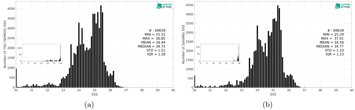
Figure 3: Histograms of SSS from TSG (SAMOS) (a) and CCI SSS L4 Merged-OI v4.41 - 7-day running (ESA) (b) considering all match-up pairs per bins of 0.1 over the Equatorial Ocean 10N-10S Pi-MEP region and for the full satellite product period.
