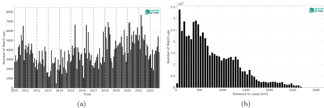
Figure 2: Number of match-ups between TSG (LEGOS-DM) and CCI SSS L4 Merged-OI v4.41 - 7-day running (ESA) SSS as a function of time (a) and as function of the distance to coast (b) over the Equatorial Ocean 10N-10S Pi-MEP region and for the full satellite product period.
