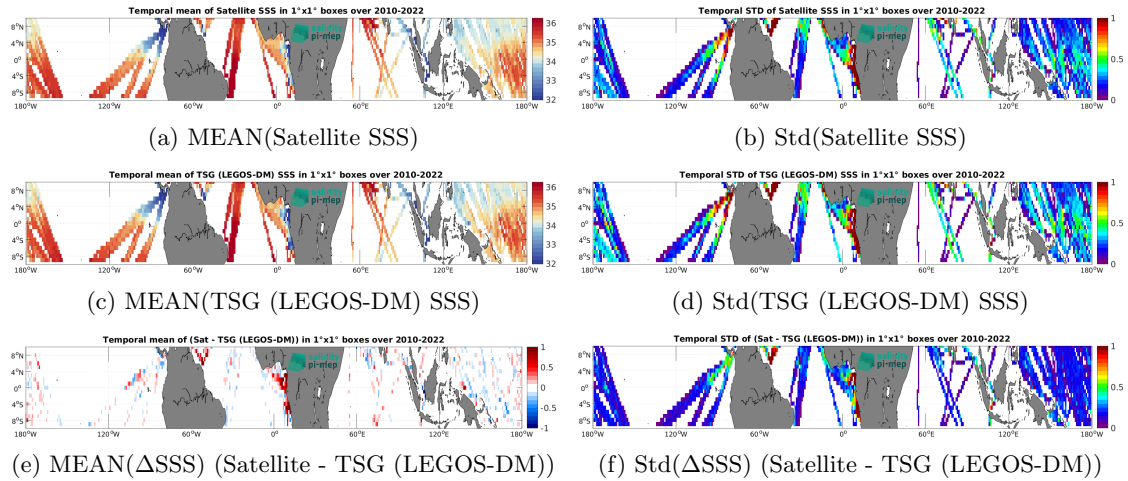
Figure 7: Temporal mean (left) and Std (right) of SSS from CCI SSS L4 Merged-OI v4.41 - 7-day running (ESA) (top), TSG (LEGOS-DM) in situ dataset (middle), and of \Delta SSS (Satellite - TSG (LEGOS-DM)). Only match-up pairs are used to generate these maps.
