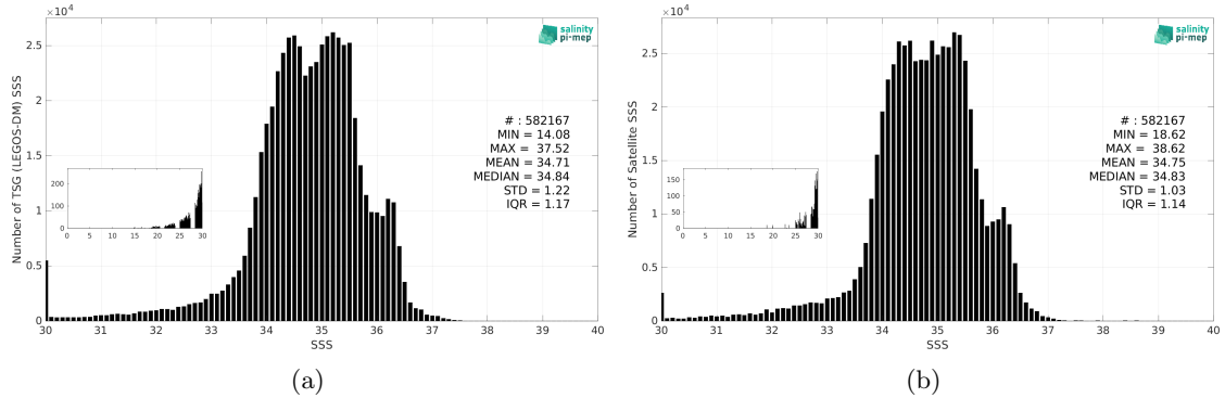
Figure 3: Histograms of SSS from TSG (LEGOS-DM) (a) and CCI SSS L4 Merged-OI v4.41 - 7-day running (ESA) (b) considering all match-up pairs per bins of 0.1 over the Equatorial Ocean 10N-10S Pi-MEP region and for the full satellite product period.
