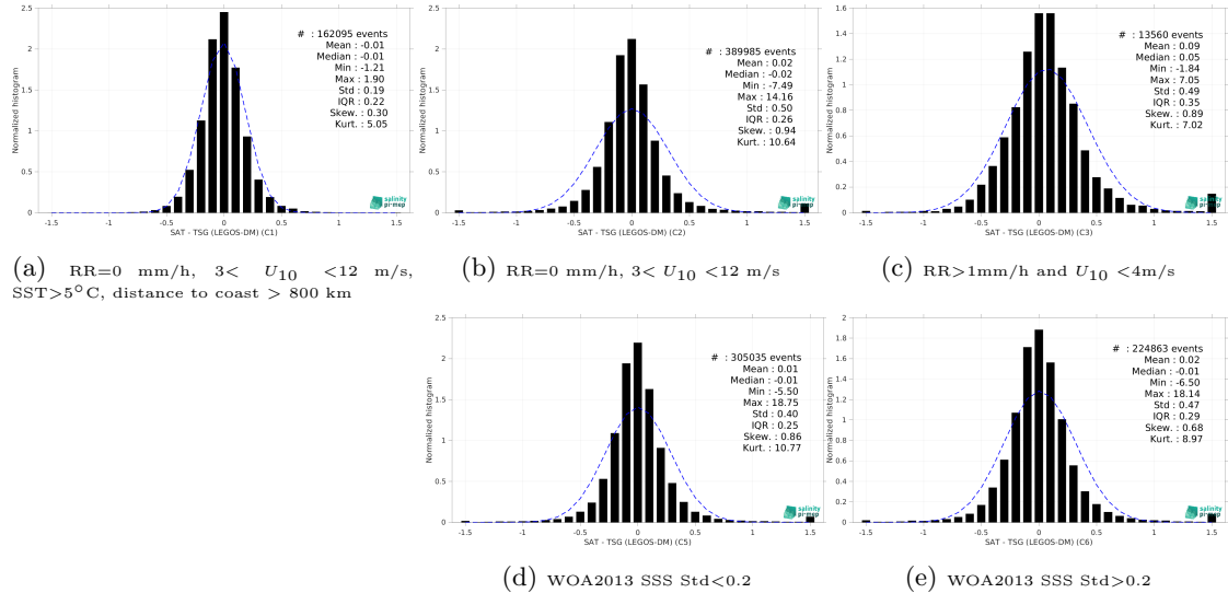
Figure 15: Normalized histogram of \Delta SSS (CCI SSS L4 Merged-OI v4.41 - 7-day running (ESA) - TSG (LEGOS-DM)) for 5 different subdatasets corresponding to: RR=0 mm/h, 3 < U_{10} < 12 m/s, SST>5°C, distance to coast > 800 km (a), RR=0 mm/h, 3 < U_{10} < 12 m/s (b), RR>1mm/h and U_{10} < 4 m/s (c), WOA2013 SSS Std<0.2 (d), WOA2013 SSS Std>0.2 (e).
