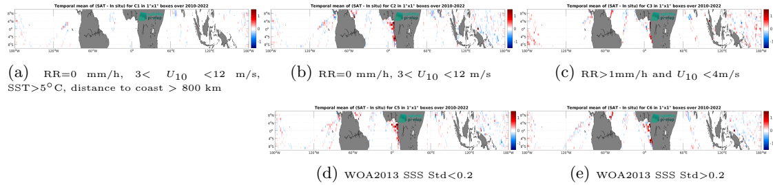
Figure 14: Temporal mean gridded over spatial boxes of size 1^\circ \times 1^\circ of \Delta SSS (CCI SSS L4 Merged-OI v4.41 - 7-day running (ESA) - TSG (LEGOS-DM)) for 5 different subdatasets corresponding to: RR=0 mm/h, 3 < U_{10} < 12 m/s, SST>5°C, distance to coast > 800 km (a), RR=0 mm/h, 3 < U_{10} < 12 m/s (b), RR>1mm/h and U_{10} < 4 m/s (c), WOA2013 SSS Std<0.2 (d), WOA2013 SSS Std>0.2 (e).
