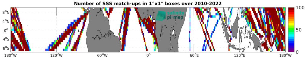
Figure 5: Number of SSS match-ups between TSG (LEGOS-DM) SSS and the CCI SSS L4 Merged-OI v4.41 - 7-day running (ESA) SSS product for the Equatorial Ocean 10N-10S Pi-MEP region over 1^\circ \times 1^\circ boxes and for the full satellite product period.
