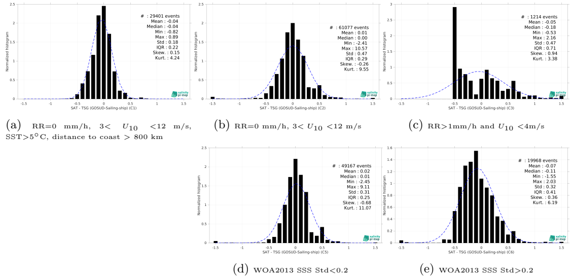
Figure 15: Normalized histogram of \Delta SSS (CCI SSS L4 Merged-OI v4.41 - 7-day running (ESA) - TSG (GOSUD-Sailing-ship)) for 5 different subdatasets corresponding to: RR=0 mm/h, 3 < U_{10} < 12 m/s, SST>5°C, distance to coast > 800 km (a), RR=0 mm/h, 3 < U_{10} < 12 m/s (b), RR>1mm/h and U_{10} < 4 m/s (c), WOA2013 SSS Std<0.2 (d), WOA2013 SSS Std>0.2 (e).
