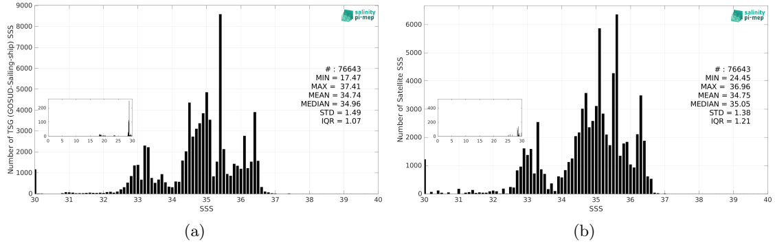
Figure 3: Histograms of SSS from TSG (GOSUD-Sailing-ship) (a) and CCI SSS L4 Merged-OI v4.41 - 7-day running (ESA) (b) considering all match-up pairs per bins of 0.1 over the Equatorial Ocean 10N-10S Pi-MEP region and for the full satellite product period.
