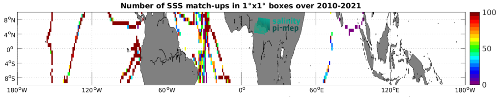
Figure 5: Number of SSS match-ups between TSG (GOSUD-Sailing-ship) SSS and the CCI SSS L4 Merged-OI v4.41 - 7-day running (ESA) SSS product for the Equatorial Ocean 10N-10S Pi-MEP region over 1^\circ \times 1^\circ boxes and for the full satellite product period.
