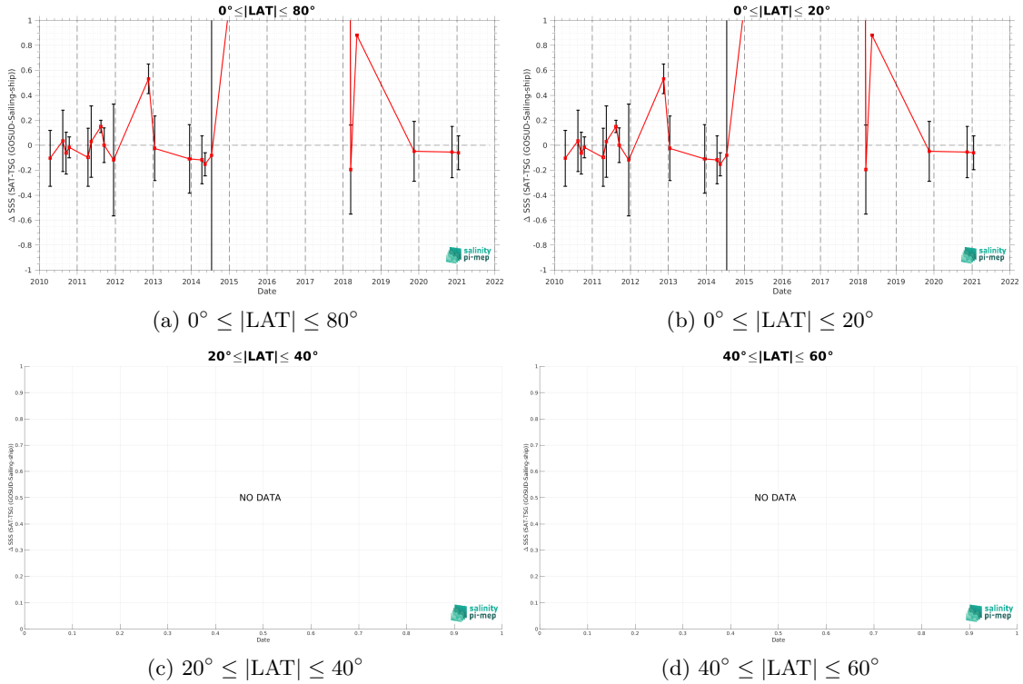
Figure 11: Monthly median (red curves) of \Delta SSS (Satellite - in situ ) between CCI SSS L4 Merged-OI v4.41 - 7-day running (ESA) and TSG (GOSUD-Sailing-ship) SSS as function of time for all the collected Pi-MEP match-up pairs estimated over the Equatorial Ocean 10N-10S Pi-MEP region and for the full satellite product period are shown for different latitude bands: (a) 80°S-80°N, (b) 20°S-20°N, (c) 40°S-20°S and 20°N-40°N and (d) 60°S-40°S and 40°N-60°N.
