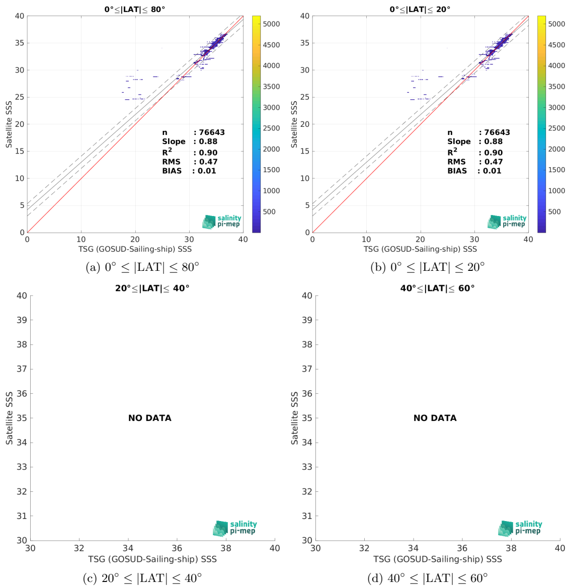
Figure 10: Contour maps of the concentration of CCI SSS L4 Merged-OI v4.41 - 7-day running (ESA) SSS (y-axis) versus TSG (GOSUD-Sailing-ship) SSS (x-axis) at match-up pairs for different latitude bands. For each plot, the red line shows x=y . The black thin and dashed lines indicate a linear fit through the data cloud and the \pm 95\% confidence levels, respectively. The number match-up pairs n , the slope and R^2 coefficient of the linear fit, the root mean square (RMS) and the mean bias between satellite and in situ data are indicated for each latitude band in each plots.
