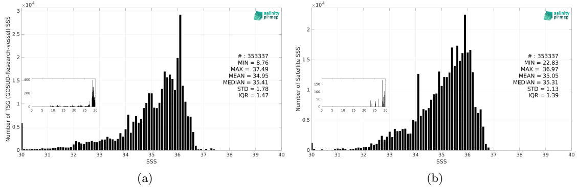
Figure 3: Histograms of SSS from TSG (GOSUD-Research-vessel) (a) and CCI SSS L4 Merged-OI v4.41 - 7-day running (ESA) (b) considering all match-up pairs per bins of 0.1 over the Equatorial Ocean 10N-10S Pi-MEP region and for the full satellite product period.
