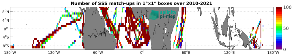
Figure 5: Number of SSS match-ups between TSG (GOSUD-Research-vessel) SSS and the CCI SSS L4 Merged-OI v4.41 - 7-day running (ESA) SSS product for the Equatorial Ocean 10N-10S Pi-MEP region over 1^\circ \times 1^\circ boxes and for the full satellite product period.
