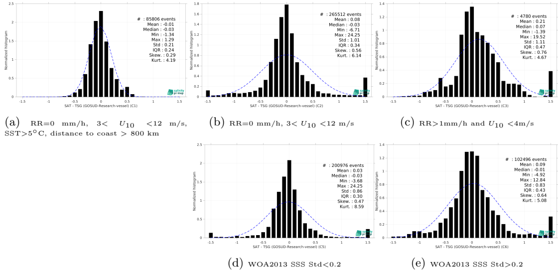
Figure 15: Normalized histogram of \Delta\text{SSS} (CCI SSS L4 Merged-OI v4.41 - 7-day running (ESA) - TSG (GOSUD-Research-vessel)) for 5 different subdatasets corresponding to: RR=0 mm/h, 3 < U_{10} < 12 m/s, SST>5°C, distance to coast > 800 km (a), RR=0 mm/h, 3 < U_{10} < 12 m/s (b), RR>1mm/h and U_{10} < 4 m/s (c), WOA2013 SSS Std<0.2 (d), WOA2013 SSS Std>0.2 (e).
