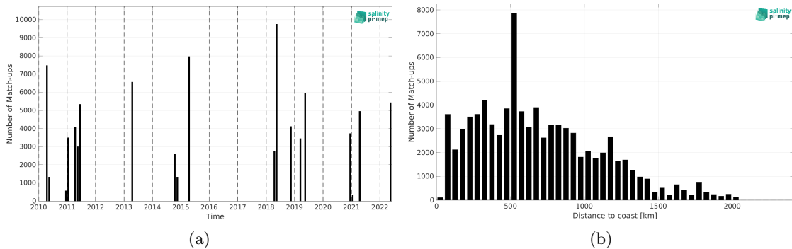
Figure 2: Number of match-ups between TSG (CSIC-UTM) and CCI SSS L4 Merged-OI v4.41 - 7-day running (ESA) SSS as a function of time (a) and as function of the distance to coast (b) over the Equatorial Ocean 10N-10S Pi-MEP region and for the full satellite product period.
