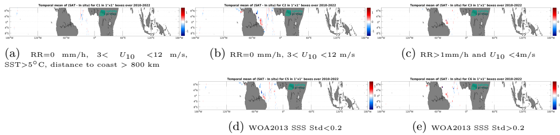
Figure 14: Temporal mean gridded over spatial boxes of size 1^\circ \times 1^\circ of \Delta SSS (CCI SSS L4 Merged-OI v4.41 - 7-day running (ESA) - TSG (CSIC-UTM)) for 5 different subdatasets corresponding to: RR=0 mm/h, 3 < U_{10} < 12 m/s, SST>5°C, distance to coast > 800 km (a), RR=0 mm/h, 3 < U_{10} < 12 m/s (b), RR>1mm/h and U_{10} < 4 m/s (c), WOA2013 SSS Std<0.2 (d), WOA2013 SSS Std>0.2 (e).
