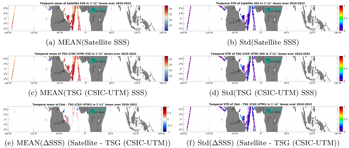
Figure 7: Temporal mean (left) and Std (right) of SSS from CCI SSS L4 Merged-OI v4.41 - 7-day running (ESA) (top), TSG (CSIC-UTM) ( in situ ) (middle), and of \Delta SSS (Satellite - TSG (CSIC-UTM)). Only match-up pairs are used to generate these maps.
