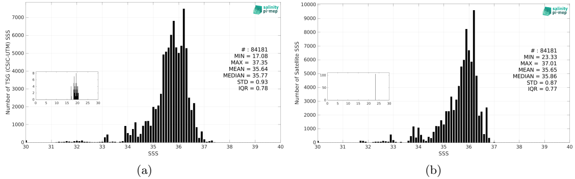
Figure 3: Histograms of SSS from TSG (CSIC-UTM) (a) and CCI SSS L4 Merged-OI v4.41 - 7-day running (ESA) (b) considering all match-up pairs per bins of 0.1 over the Equatorial Ocean 10N-10S Pi-MEP region and for the full satellite product period.
