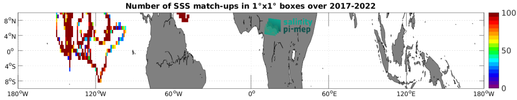
Figure 5: Number of SSS match-ups between Saildrone SSS and the CCI SSS L4 Merged-OI v4.41 - 7-day running (ESA) SSS product for the Equatorial Ocean 10N-10S Pi-MEP region over 1^\circ \times 1^\circ boxes and for the full satellite product period.
