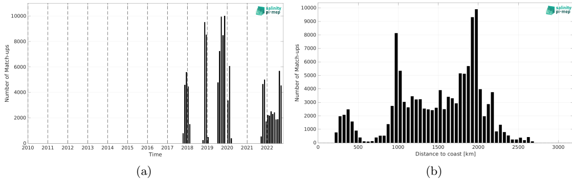
Figure 2: Number of match-ups between Saildrone and CCI SSS L4 Merged-OI v4.41 - 7-day running (ESA) SSS as a function of time (a) and as function of the distance to coast (b) over the Equatorial Ocean 10N-10S Pi-MEP region and for the full satellite product period.
