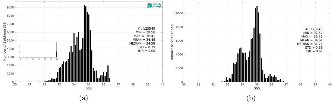
Figure 3: Histograms of SSS from Saildrone (a) and CCI SSS L4 Merged-OI v4.41 - 7-day running (ESA) (b) considering all match-up pairs per bins of 0.1 over the Equatorial Ocean 10N-10S Pi-MEP region and for the full satellite product period.
