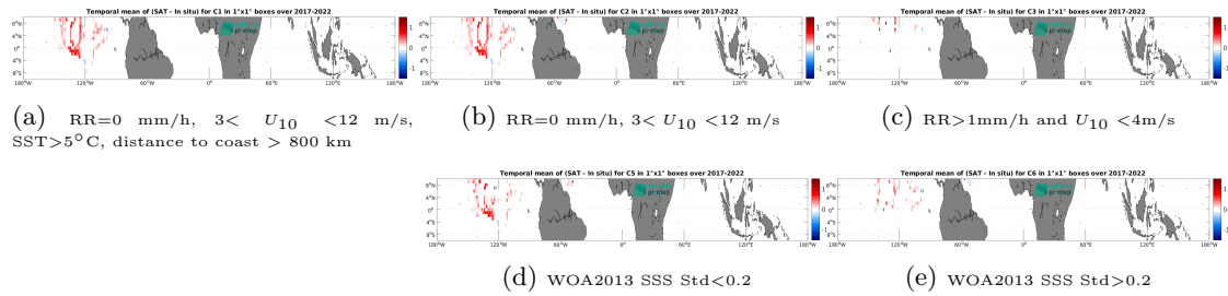
Figure 14: Temporal mean gridded over spatial boxes of size 1^\circ \times 1^\circ of \Delta SSS (CCI SSS L4 Merged-OI v4.41 - 7-day running (ESA) - Saildrone) for 5 different subdatasets corresponding to:RR=0 mm/h, 3 < U_{10} < 12 m/s, SST>5°C, distance to coast > 800 km (a), RR=0 mm/h, 3 < U_{10} < 12 m/s (b), RR>1mm/h and U_{10} < 4 m/s (c), WOA2013 SSS Std<0.2 (d), WOA2013 SSS Std>0.2 (e).
