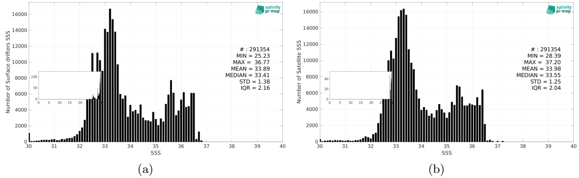
Figure 3: Histograms of SSS from Surface drifters (a) and CCI SSS L4 Merged-OI v4.41 - 7-day running (ESA) (b) considering all match-up pairs per bins of 0.1 over the Equatorial Ocean 10N-10S Pi-MEP region and for the full satellite product period.
