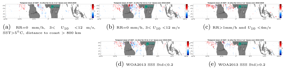
Figure 13: Temporal mean gridded over spatial boxes of size 1^\circ \times 1^\circ of \Delta SSS (CCI SSS L4 Merged-OI v4.41 - 7-day running (ESA) - Surface drifters) for 5 different subdatasets corresponding to: RR=0 mm/h, 3 < U_{10} < 12 m/s, SST >5^\circ C, distance to coast > 800 km (a), RR=0 mm/h, 3 < U_{10} < 12 m/s (b), RR >1 mm/h and U_{10} < 4 m/s (c), WOA2013 SSS Std <0.2 (d), WOA2013 SSS Std >0.2 (e).
