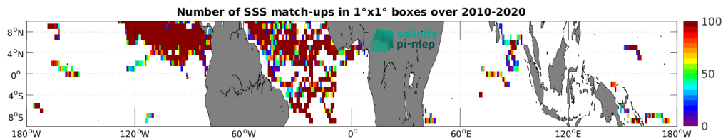
Figure 4: Number of SSS match-ups between Surface drifters SSS and the CCI SSS L4 Merged-OI v4.41 - 7-day running (ESA) SSS product for the Equatorial Ocean 10N-10S Pi-MEP region over 1^\circ \times 1^\circ boxes and for the full satellite product period.
