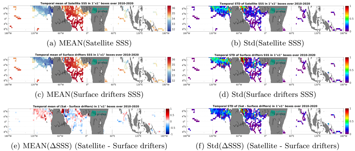
Figure 6: Temporal mean (left) and Std (right) of SSS from CCI SSS L4 Merged-OI v4.41 - 7-day running (ESA) (top), Surface drifters (middle), and of \Delta SSS (Satellite - Surface drifters). Only match-up pairs are used to generate these maps.
