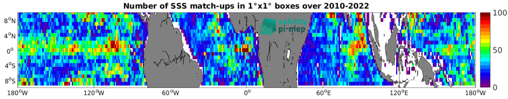
Figure 5: Number of SSS match-ups between Argo SSS and the CCI SSS L4 Merged-OI v4.41 - 7-day running (ESA) SSS product for the Equatorial Ocean 10N-10S Pi-MEP region over 1^\circ \times 1^\circ boxes and for the full satellite product period.
