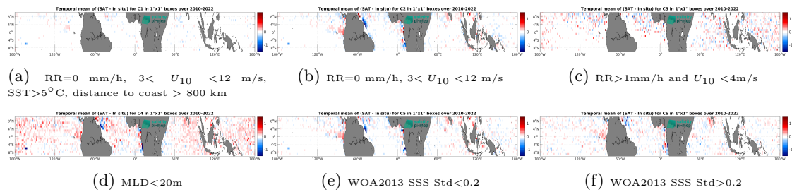
Figure 14: Temporal mean gridded over spatial boxes of size 1^\circ \times 1^\circ of \Delta SSS (CCI SSS L4 Merged-OI v4.41 - 7-day running (ESA) - Argo) for 6 different subdatasets corresponding to:RR=0 mm/h, 3 < U_{10} < 12 m/s, SST >5^\circ C, distance to coast > 800 km (a), RR=0 mm/h, 3 < U_{10} < 12 m/s (b), RR >1 mm/h and U_{10} < 4 m/s (c),MLD <20 m (d),WOA2013 SSS Std <0.2 (e),WOA2013 SSS Std >0.2 (f).
