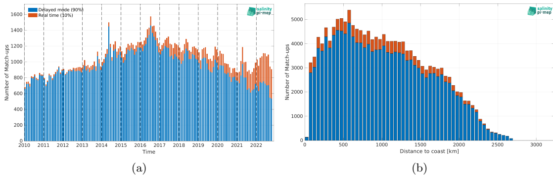
Figure 2: Number of match-ups between Argo and CCI SSS L4 Merged-OI v4.41 - 7-day running (ESA) SSS as a function of time (a) and as function of the distance to coast (b) over the Equatorial Ocean 10N-10S Pi-MEP region and for the full satellite product period.
