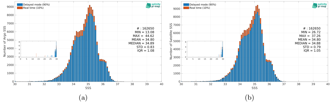
Figure 3: Histograms of SSS from Argo (a) and CCI SSS L4 Merged-OI v4.41 - 7-day running (ESA) (b) considering all match-up pairs per bins of 0.1 over the Equatorial Ocean 10N-10S Pi-MEP region and for the full satellite product period.
