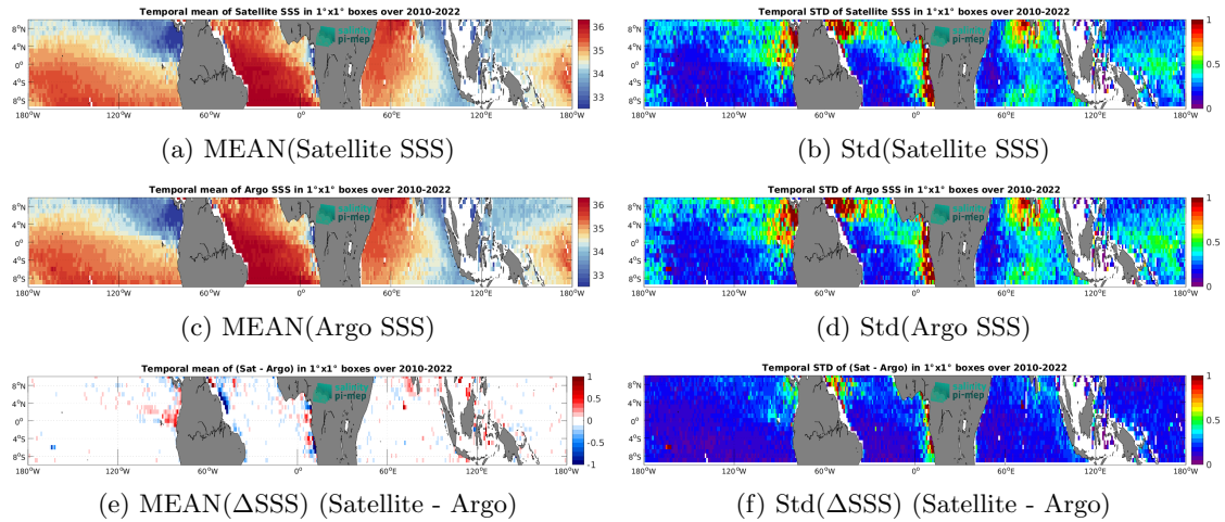
Figure 7: Temporal mean (left) and Std (right) of SSS from CCI SSS L4 Merged-OI v4.41 - 7-day running (ESA) (top), Argo (middle), and of \Delta SSS (Satellite - Argo). Only match-up pairs are used to generate these maps.
