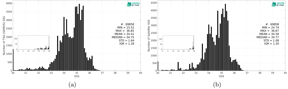
Figure 3: Histograms of SSS from TSG (SAMOS) (a) and CCI SSS L4 Merged-OI v4.41 - 30-day running (ESA) (b) considering all match-up pairs per bins of 0.1 over the Equatorial Ocean 10N-10S Pi-MEP region and for the full satellite product period.
