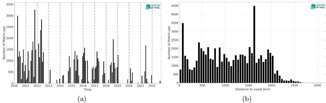
Figure 2: Number of match-ups between TSG (SAMOS) and CCI SSS L4 Merged-OI v4.41 - 30-day running (ESA) SSS as a function of time (a) and as function of the distance to coast (b) over the Equatorial Ocean 10N-10S Pi-MEP region and for the full satellite product period.
