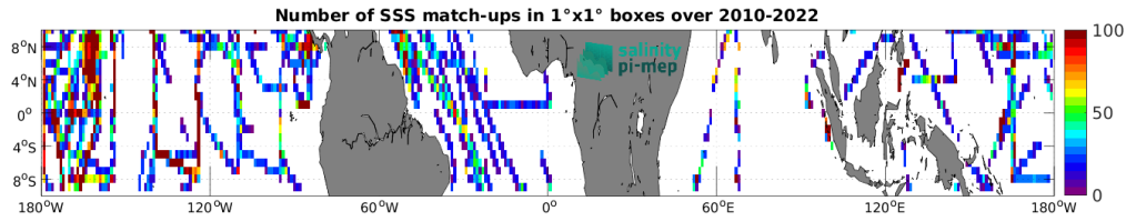
Figure 5: Number of SSS match-ups between TSG (SAMOS) SSS and the CCI SSS L4 Merged-OI v4.41 - 30-day running (ESA) SSS product for the Equatorial Ocean 10N-10S Pi-MEP region over 1^\circ \times 1^\circ boxes and for the full satellite product period.
