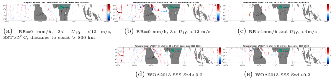
Figure 14: Temporal mean gridded over spatial boxes of size 1^\circ \times 1^\circ of \Delta\text{SSS} (CCI SSS L4 Merged-OI v4.41 - 30-day running (ESA) - TSG (SAMOS)) for 5 different subdatasets corresponding to: RR=0 mm/h, 3 < U_{10} < 12 m/s, SST>5°C, distance to coast > 800 km (a), RR=0 mm/h, 3 < U_{10} < 12 m/s (b), RR>1mm/h and U_{10} < 4 m/s (c), WOA2013 SSS Std<0.2 (d), WOA2013 SSS Std>0.2 (e).
