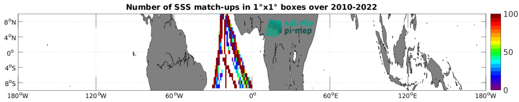
Figure 5: Number of SSS match-ups between TSG (Polarstern) SSS and the CCI SSS L4 Merged-OI v4.41 - 30-day running (ESA) SSS product for the Equatorial Ocean 10N-10S Pi-MEP region over 1^\circ \times 1^\circ boxes and for the full satellite product period.
