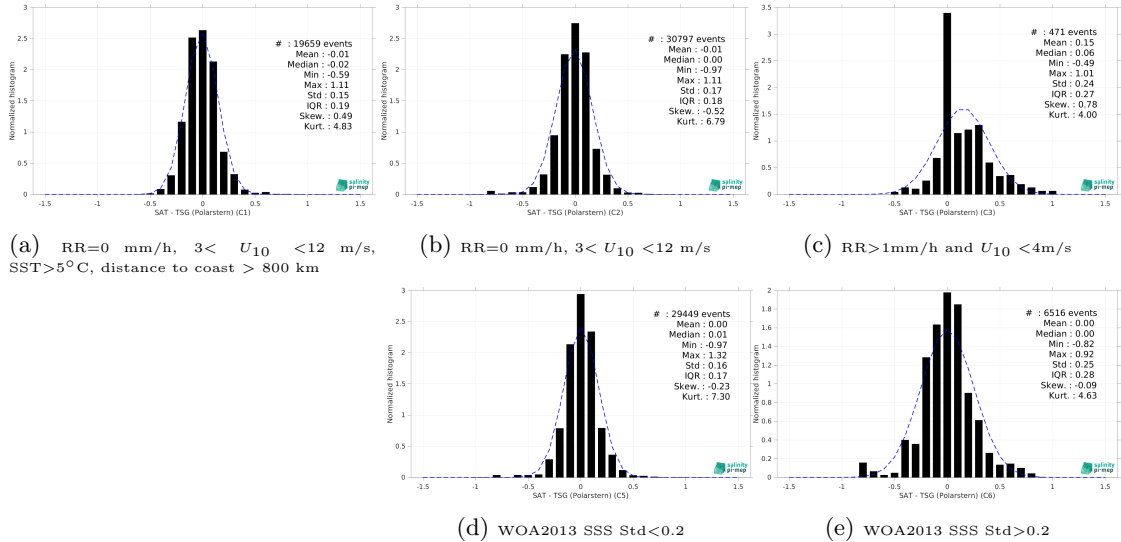
Figure 15: Normalized histogram of \Delta SSS (CCI SSS L4 Merged-OI v4.41 - 30-day running (ESA) - TSG (Polarstern)) for 5 different subdatasets corresponding to: RR=0 mm/h, 3 < U_{10} < 12 m/s, SST>5°C, distance to coast > 800 km (a), RR=0 mm/h, 3 < U_{10} < 12 m/s (b), RR>1mm/h and U_{10} < 4 m/s (c), WOA2013 SSS Std<0.2 (d), WOA2013 SSS Std>0.2 (e).
