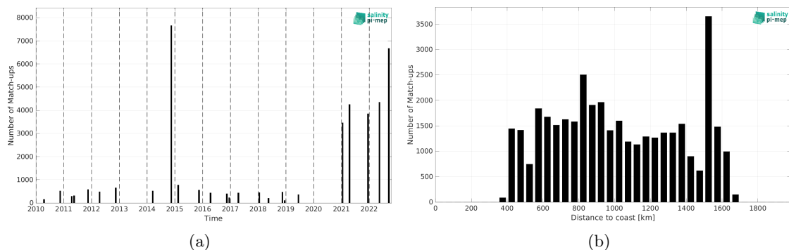
Figure 2: Number of match-ups between TSG (Polarstern) and CCI SSS L4 Merged-OI v4.41 - 30-day running (ESA) SSS as a function of time (a) and as function of the distance to coast (b) over the Equatorial Ocean 10N-10S Pi-MEP region and for the full satellite product period.
