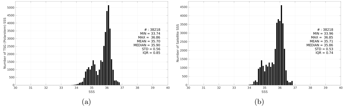
Figure 3: Histograms of SSS from TSG (Polarstern) (a) and CCI SSS L4 Merged-OI v4.41 - 30-day running (ESA) (b) considering all match-up pairs per bins of 0.1 over the Equatorial Ocean 10N-10S Pi-MEP region and for the full satellite product period.
