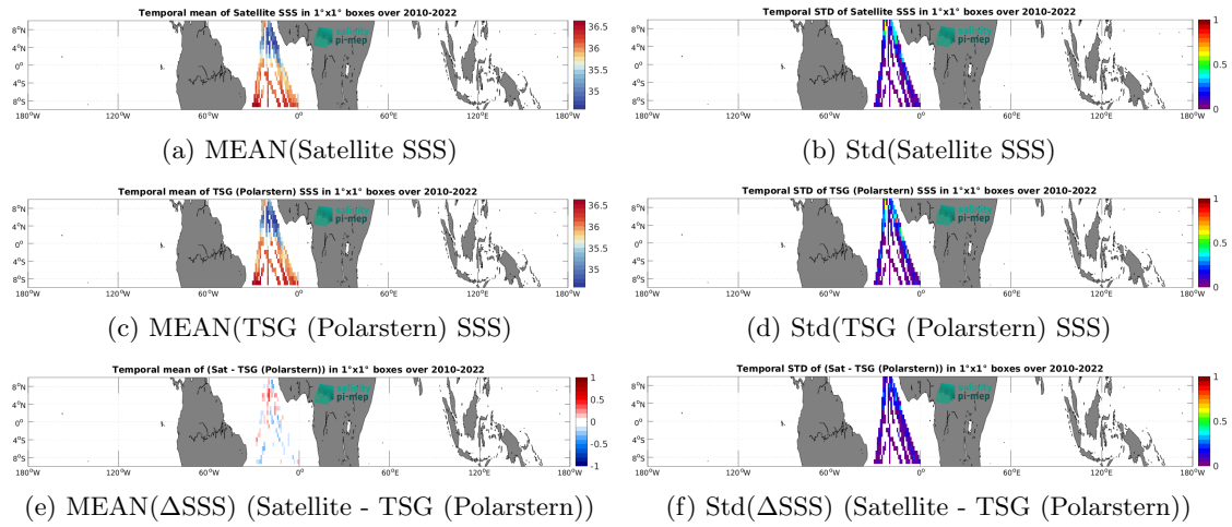
Figure 7: Temporal mean (left) and Std (right) of SSS from CCI SSS L4 Merged-OI v4.41 - 30-day running (ESA) (top), TSG (Polarstern) (middle), and of \Delta SSS (Satellite - TSG (Polarstern)). Only match-up pairs are used to generate these maps.
