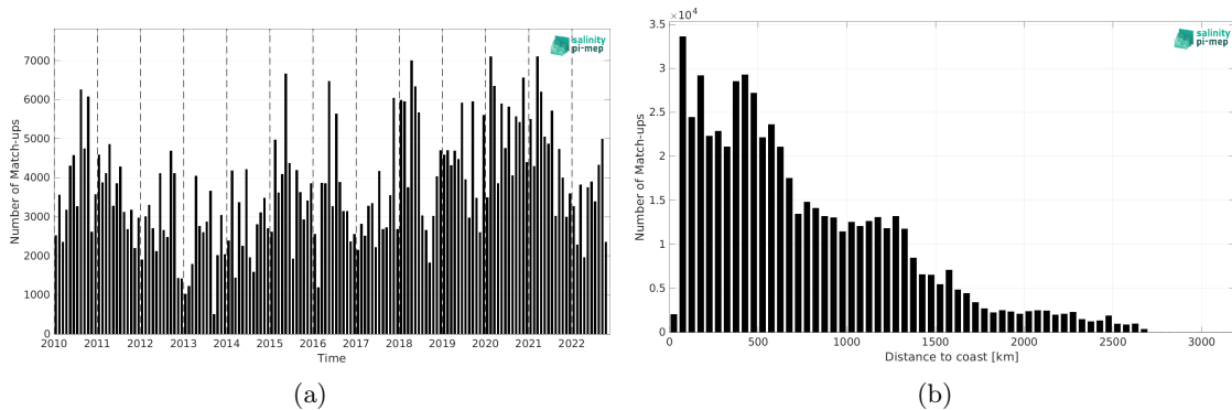
Figure 2: Number of match-ups between TSG (LEGOS-DM) and CCI SSS L4 Merged-OI v4.41 - 30-day running (ESA) SSS as a function of time (a) and as function of the distance to coast (b) over the Equatorial Ocean 10N-10S Pi-MEP region and for the full satellite product period.
