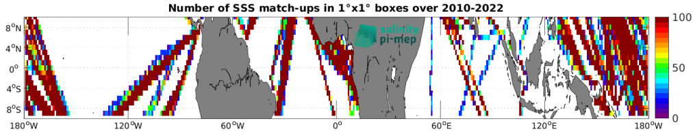
Figure 5: Number of SSS match-ups between TSG (LEGOS-DM) SSS and the CCI SSS L4 Merged-OI v4.41 - 30-day running (ESA) SSS product for the Equatorial Ocean 10N-10S Pi-MEP region over 1^\circ \times 1^\circ boxes and for the full satellite product period.
