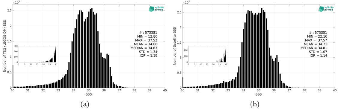
Figure 3: Histograms of SSS from TSG (LEGOS-DM) (a) and CCI SSS L4 Merged-OI v4.41 - 30-day running (ESA) (b) considering all match-up pairs per bins of 0.1 over the Equatorial Ocean 10N-10S Pi-MEP region and for the full satellite product period.
