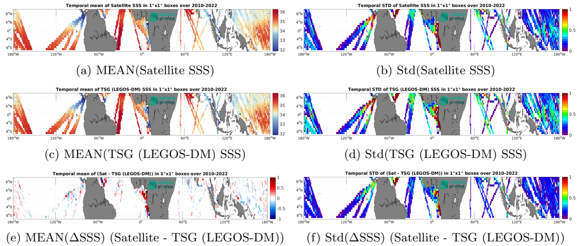
Figure 7: Temporal mean (left) and Std (right) of SSS from CCI SSS L4 Merged-OI v4.41 - 30-day running (ESA) (top), TSG (LEGOS-DM) (middle), and of \Delta SSS (Satellite - TSG (LEGOS-DM)). Only match-up pairs are used to generate these maps.
