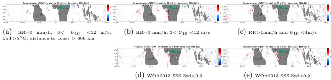
Figure 14: Temporal mean gridded over spatial boxes of size 1^\circ \times 1^\circ of \Delta SSS (CCI SSS L4 Merged-OI v4.41 - 30-day running (ESA) - TSG (LEGOS-DM)) for 5 different subdatasets corresponding to: RR=0 mm/h, 3 < U_{10} < 12 m/s, SST>5°C, distance to coast > 800 km (a), RR=0 mm/h, 3 < U_{10} < 12 m/s (b), RR>1mm/h and U_{10} < 4 m/s (c), WOA2013 SSS Std<0.2 (d), WOA2013 SSS Std>0.2 (e).
