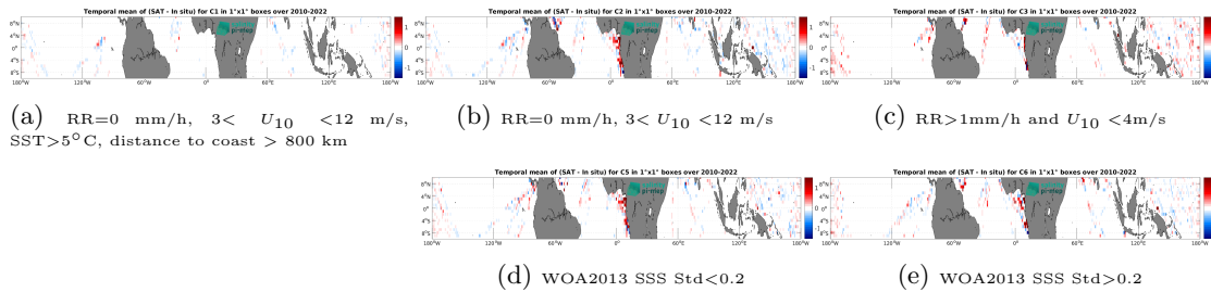
Figure 14: Temporal mean gridded over spatial boxes of size 1^\circ \times 1^\circ of \Delta\text{SSS} (CCI SSS L4 Merged-OI v4.41 - 30-day running (ESA) - TSG (LEGOS-DM)) for 5 different subdatasets corresponding to: RR=0 mm/h, 3 < U_{10} < 12 m/s, SST>5°C, distance to coast > 800 km (a), RR=0 mm/h, 3 < U_{10} < 12 m/s (b), RR>1mm/h and U_{10} < 4 m/s (c), WOA2013 SSS Std<0.2 (d), WOA2013 SSS Std>0.2 (e).
