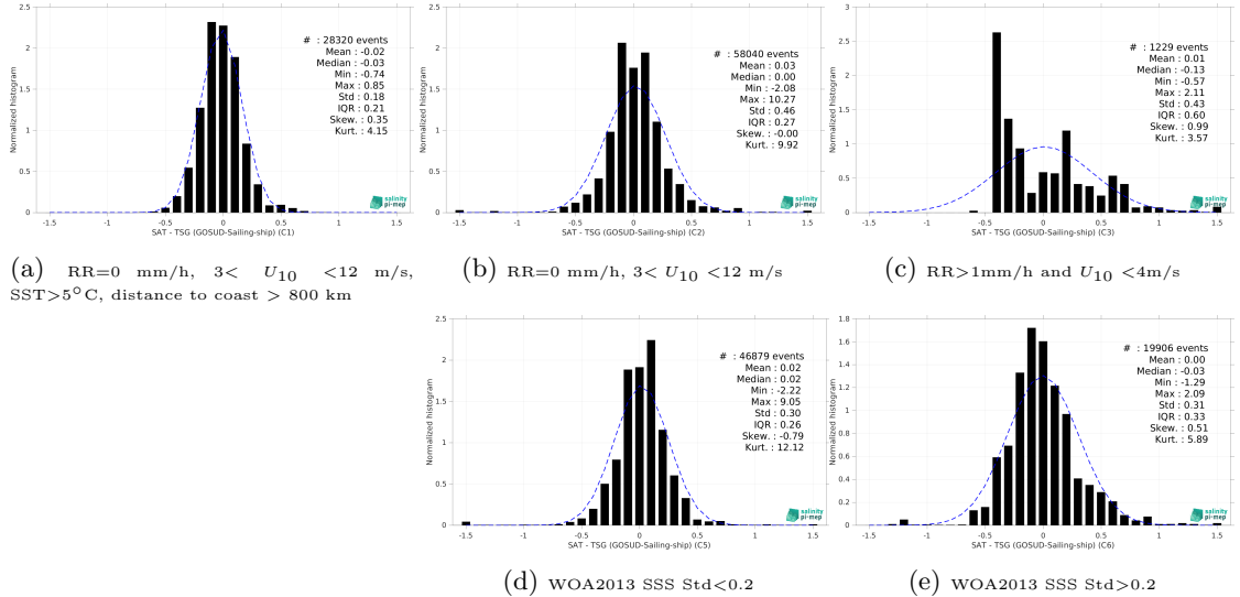
Figure 15: Normalized histogram of \Delta\text{SSS} (CCI SSS L4 Merged-OI v4.41 - 30-day running (ESA) - TSG (GOSUD-Sailing-ship)) for 5 different subdatasets corresponding to: RR=0 mm/h, 3 < U_{10} < 12 m/s, SST>5°C, distance to coast > 800 km (a), RR=0 mm/h, 3 < U_{10} < 12 m/s (b), RR>1mm/h and U_{10} < 4 m/s (c), WOA2013 SSS Std<0.2 (d), WOA2013 SSS Std>0.2 (e).
