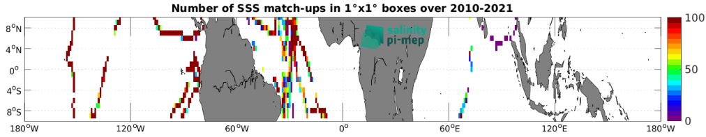
Figure 5: Number of SSS match-ups between TSG (GOSUD-Sailing-ship) SSS and the CCI SSS L4 Merged-OI v4.41 - 30-day running (ESA) SSS product for the Equatorial Ocean 10N-10S Pi-MEP region over 1^\circ \times 1^\circ boxes and for the full satellite product period.
