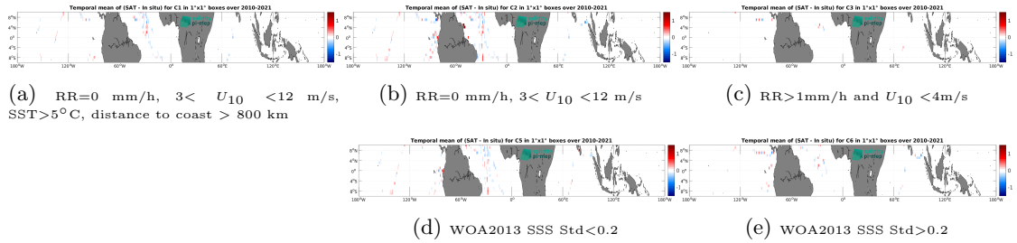
Figure 14: Temporal mean gridded over spatial boxes of size 1^\circ \times 1^\circ of \Delta\text{SSS} (CCI SSS L4 Merged-OI v4.41 - 30-day running (ESA) - TSG (GOSUD-Sailing-ship)) for 5 different subdatasets corresponding to:RR=0 mm/h, 3 < U_{10} < 12 m/s, SST>5°C, distance to coast > 800 km (a), RR=0 mm/h, 3 < U_{10} < 12 m/s (b), RR>1mm/h and U_{10} < 4 m/s (c), WOA2013 SSS Std<0.2 (d), WOA2013 SSS Std>0.2 (e).
