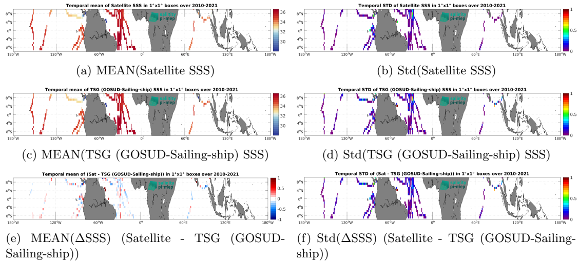
Figure 7: Temporal mean (left) and Std (right) of SSS from CCI SSS L4 Merged-OI v4.41 - 30-day running (ESA) (top), TSG (GOSUD-Sailing-ship) (middle), and of \Delta SSS (Satellite - TSG (GOSUD-Sailing-ship)). Only match-up pairs are used to generate these maps.
