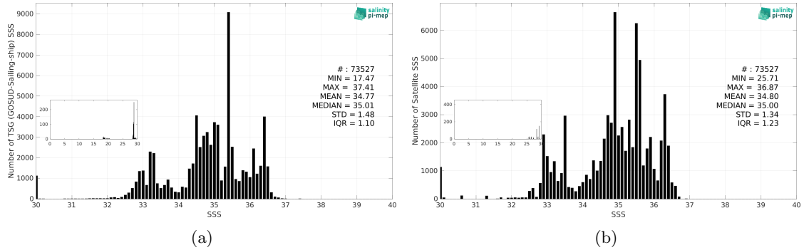
Figure 3: Histograms of SSS from TSG (GOSUD-Sailing-ship) (a) and CCI SSS L4 Merged-OI v4.41 - 30-day running (ESA) (b) considering all match-up pairs per bins of 0.1 over the Equatorial Ocean 10N-10S Pi-MEP region and for the full satellite product period.
