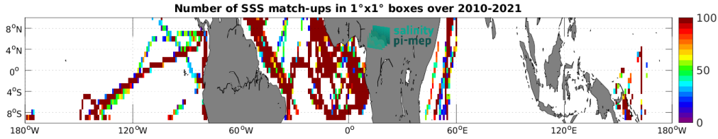
Figure 5: Number of SSS match-ups between TSG (GOSUD-Research-vessel) SSS and the CCI SSS L4 Merged-OI v4.41 - 30-day running (ESA) SSS product for the Equatorial Ocean 10N-10S Pi-MEP region over 1^\circ \times 1^\circ boxes and for the full satellite product period.
