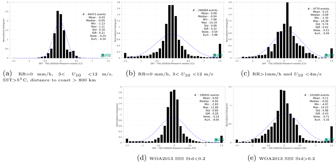
Figure 15: Normalized histogram of \Delta\text{SSS} (CCI SSS L4 Merged-OI v4.41 - 30-day running (ESA) - TSG (GOSUD-Research-vessel)) for 5 different subdatasets corresponding to: RR=0 mm/h, 3 < U_{10} < 12 m/s, SST>5°C, distance to coast > 800 km (a), RR=0 mm/h, 3 < U_{10} < 12 m/s (b), RR>1mm/h and U_{10} < 4 m/s (c), WOA2013 SSS Std<0.2 (d), WOA2013 SSS Std>0.2 (e).
