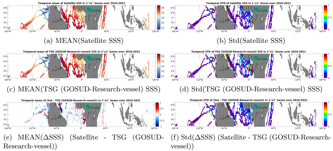
Figure 7: Temporal mean (left) and Std (right) of SSS from CCI SSS L4 Merged-OI v4.41 - 30-day running (ESA) (top), TSG (GOSUD-Research-vessel) (middle), and of \Delta SSS (Satellite - TSG (GOSUD-Research-vessel)). Only match-up pairs are used to generate these maps.
