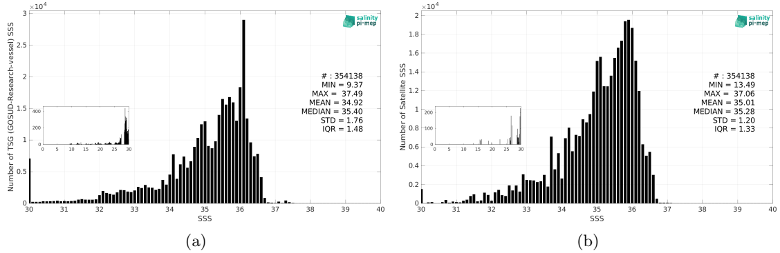
Figure 3: Histograms of SSS from TSG (GOSUD-Research-vessel) (a) and CCI SSS L4 Merged-OI v4.41 - 30-day running (ESA) (b) considering all match-up pairs per bins of 0.1 over the Equatorial Ocean 10N-10S Pi-MEP region and for the full satellite product period.
