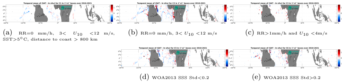
Figure 14: Temporal mean gridded over spatial boxes of size 1^\circ \times 1^\circ of \Delta\text{SSS} (CCI SSS L4 Merged-OI v4.41 - 30-day running (ESA) - TSG (GOSUD-Research-vessel)) for 5 different subdatasets corresponding to:RR=0 mm/h, 3 < U_{10} < 12 m/s, SST>5°C, distance to coast > 800 km (a), RR=0 mm/h, 3 < U_{10} < 12 m/s (b), RR>1mm/h and U_{10} < 4 m/s (c), WOA2013 SSS Std<0.2 (d), WOA2013 SSS Std>0.2 (e).
