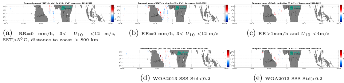
Figure 14: Temporal mean gridded over spatial boxes of size 1^\circ \times 1^\circ of \Delta\text{SSS} (CCI SSS L4 Merged-OI v4.41 - 30-day running (ESA) - TSG (CSIC-UTM)) for 5 different subdatasets corresponding to: RR=0 mm/h, 3 < U_{10} < 12 m/s, SST>5°C, distance to coast > 800 km (a), RR=0 mm/h, 3 < U_{10} < 12 m/s (b), RR>1mm/h and U_{10} < 4 m/s (c), WOA2013 SSS Std<0.2 (d), WOA2013 SSS Std>0.2 (e).
