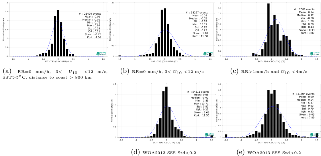
Figure 15: Normalized histogram of \Delta\text{SSS} (CCI SSS L4 Merged-OI v4.41 - 30-day running (ESA) - TSG (CSIC-UTM)) for 5 different subdatasets corresponding to: RR=0 mm/h, 3 < U_{10} < 12 m/s, SST>5°C, distance to coast > 800 km (a), RR=0 mm/h, 3 < U_{10} < 12 m/s (b), RR>1mm/h and U_{10} < 4 m/s (c), WOA2013 SSS Std<0.2 (d), WOA2013 SSS Std>0.2 (e).
