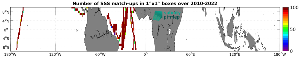
Figure 5: Number of SSS match-ups between TSG (CSIC-UTM) SSS and the CCI SSS L4 Merged-OI v4.41 - 30-day running (ESA) SSS product for the Equatorial Ocean 10N-10S Pi-MEP region over 1^\circ \times 1^\circ boxes and for the full satellite product period.
