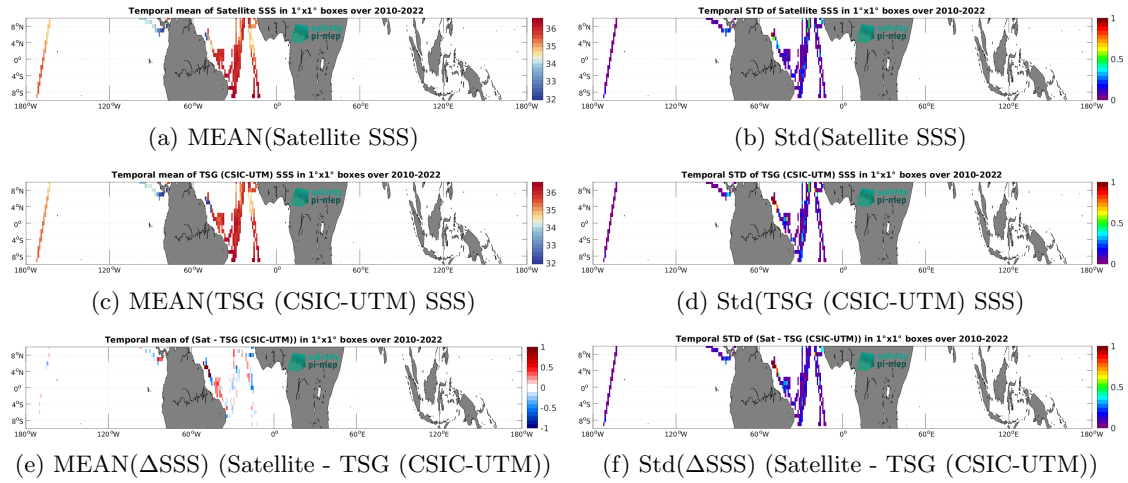
Figure 7: Temporal mean (left) and Std (right) of SSS from CCI SSS L4 Merged-OI v4.41 - 30-day running (ESA) (top), TSG (CSIC-UTM) (middle), and of \Delta SSS (Satellite - TSG (CSIC-UTM)). Only match-up pairs are used to generate these maps.
