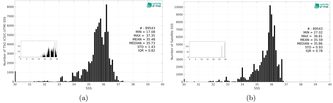
Figure 3: Histograms of SSS from TSG (CSIC-UTM) (a) and CCI SSS L4 Merged-OI v4.41 - 30-day running (ESA) (b) considering all match-up pairs per bins of 0.1 over the Equatorial Ocean 10N-10S Pi-MEP region and for the full satellite product period.
