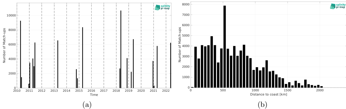
Figure 2: Number of match-ups between TSG (CSIC-UTM) and CCI SSS L4 Merged-OI v4.41 - 30-day running (ESA) SSS as a function of time (a) and as function of the distance to coast (b) over the Equatorial Ocean 10N-10S Pi-MEP region and for the full satellite product period.
