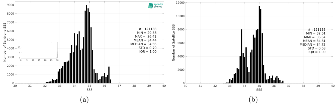
Figure 3: Histograms of SSS from Saildrone (a) and CCI SSS L4 Merged-OI v4.41 - 30-day running (ESA) (b) considering all match-up pairs per bins of 0.1 over the Equatorial Ocean 10N-10S Pi-MEP region and for the full satellite product period.
