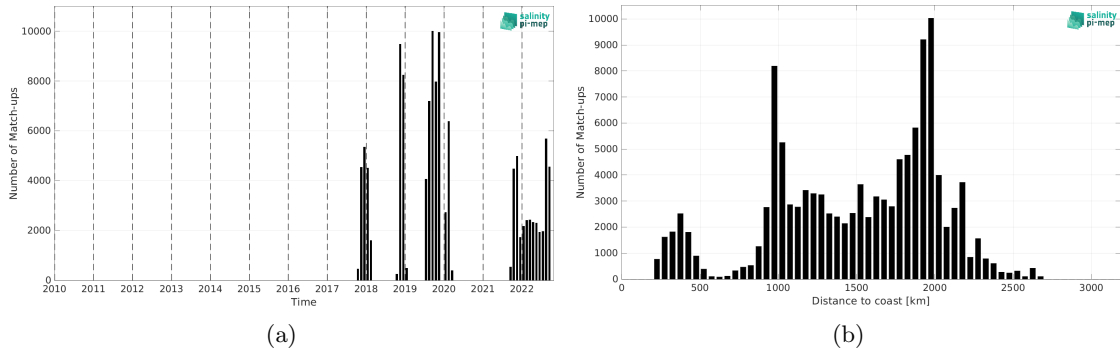
Figure 2: Number of match-ups between Saildrone and CCI SSS L4 Merged-OI v4.41 - 30-day running (ESA) SSS as a function of time (a) and as function of the distance to coast (b) over the Equatorial Ocean 10N-10S Pi-MEP region and for the full satellite product period.
