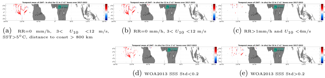
Figure 14: Temporal mean gridded over spatial boxes of size 1^\circ \times 1^\circ of \Delta SSS (CCI SSS L4 Merged-OI v4.41 - 30-day running (ESA) - Saildrone) for 5 different subdatasets corresponding to: RR=0 mm/h, 3 < U_{10} < 12 m/s, SST>5°C, distance to coast > 800 km (a), RR=0 mm/h, 3 < U_{10} < 12 m/s (b), RR>1mm/h and U_{10} < 4 m/s (c), WOA2013 SSS Std<0.2 (d), WOA2013 SSS Std>0.2 (e).
