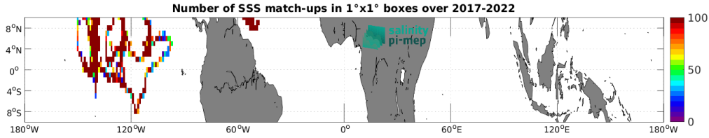
Figure 5: Number of SSS match-ups between Saildrone SSS and the CCI SSS L4 Merged-OI v4.41 - 30-day running (ESA) SSS product for the Equatorial Ocean 10N-10S Pi-MEP region over 1^\circ \times 1^\circ boxes and for the full satellite product period.
