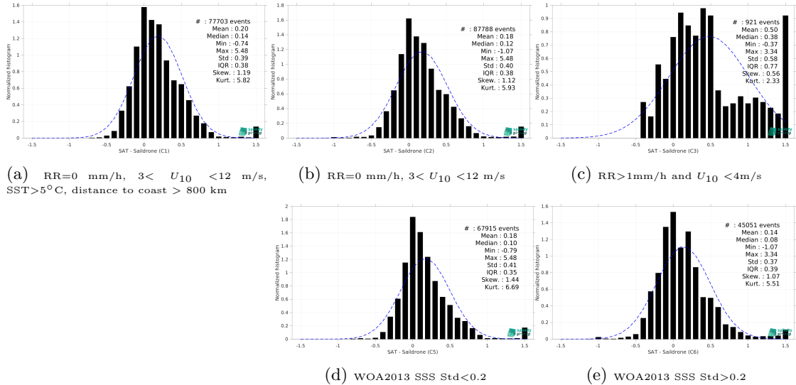
Figure 15: Normalized histogram of \Delta SSS (CCI SSS L4 Merged-OI v4.41 - 30-day running (ESA) - Saildrone) for 5 different subdatasets corresponding to: RR=0 mm/h, 3 < U_{10} < 12 m/s, SST>5°C, distance to coast > 800 km (a), RR=0 mm/h, 3 < U_{10} < 12 m/s (b), RR>1mm/h and U_{10} < 4 m/s (c), WOA2013 SSS Std<0.2 (d), WOA2013 SSS Std>0.2 (e).
