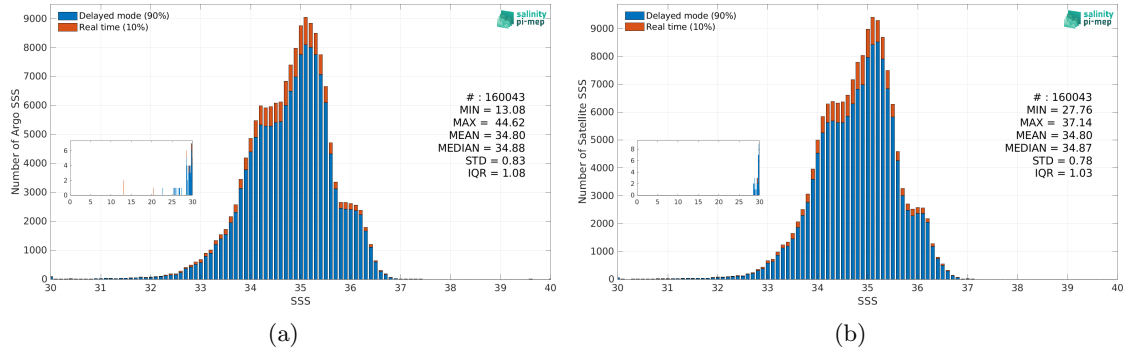
Figure 3: Histograms of SSS from Argo (a) and CCI SSS L4 Merged-OI v4.41 - 30-day running (ESA) (b) considering all match-up pairs per bins of 0.1 over the Equatorial Ocean 10N-10S Pi-MEP region and for the full satellite product period.
