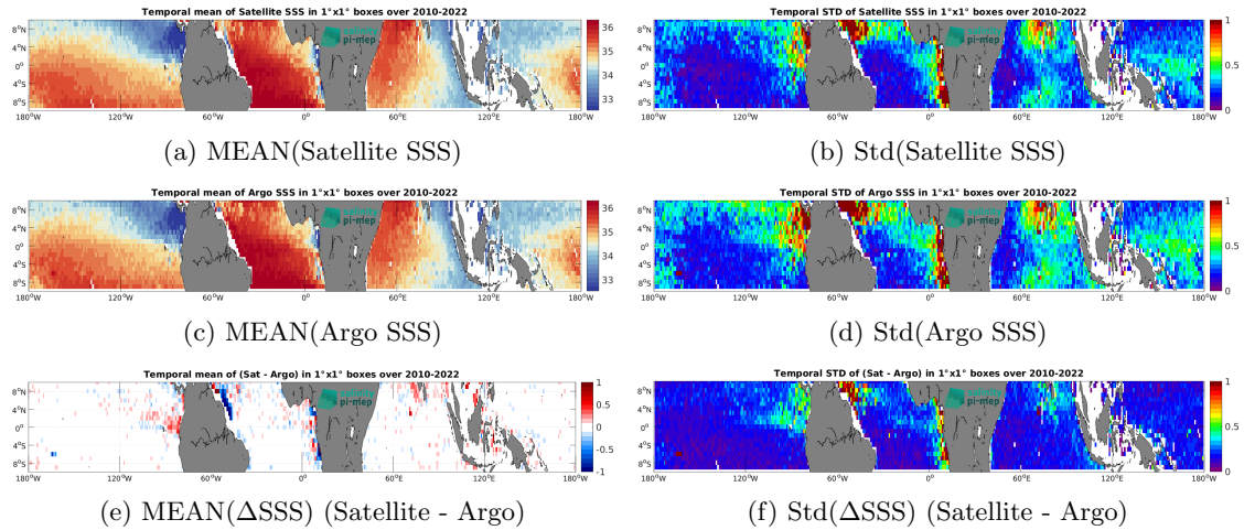
Figure 7: Temporal mean (left) and Std (right) of SSS from CCI SSS L4 Merged-OI v4.41 - 30-day running (ESA) (top), Argo (middle), and of \Delta SSS (Satellite - Argo). Only match-up pairs are used to generate these maps.
