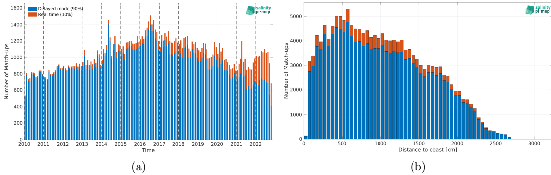
Figure 2: Number of match-ups between Argo and CCI SSS L4 Merged-OI v4.41 - 30-day running (ESA) SSS as a function of time (a) and as function of the distance to coast (b) over the Equatorial Ocean 10N-10S Pi-MEP region and for the full satellite product period.
