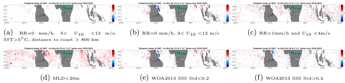
Figure 14: Temporal mean gridded over spatial boxes of size 1^\circ \times 1^\circ of \Delta SSS (CCI SSS L4 Merged-OI v4.41 - 30-day running (ESA) - Argo) for 6 different subdatasets corresponding to:RR=0 mm/h, 3 < U_{10} < 12 m/s, SST >5^\circ C, distance to coast > 800 km (a), RR=0 mm/h, 3 < U_{10} < 12 m/s (b), RR >1 mm/h and U_{10} < 4 m/s (c),MLD <20 m (d),WOA2013 SSS Std <0.2 (e),WOA2013 SSS Std >0.2 (f).
