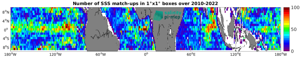
Figure 5: Number of SSS match-ups between Argo SSS and the CCI SSS L4 Merged-OI v4.41 - 30-day running (ESA) SSS product for the Equatorial Ocean 10N-10S Pi-MEP region over 1^\circ \times 1^\circ boxes and for the full satellite product period.
