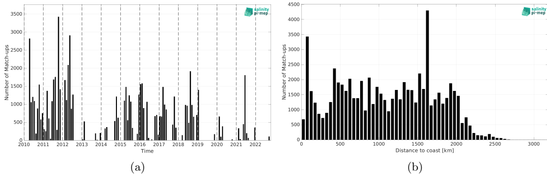
Figure 1: Number of match-ups between TSG (SAMOS) and CCI SSS L4 Merged-OI v4.4 - 7-day running (ESA) SSS as a function of time (a) and as function of the distance to coast (b) over the Equatorial Ocean 10N-10S Pi-MEP region and for the full satellite product period.
