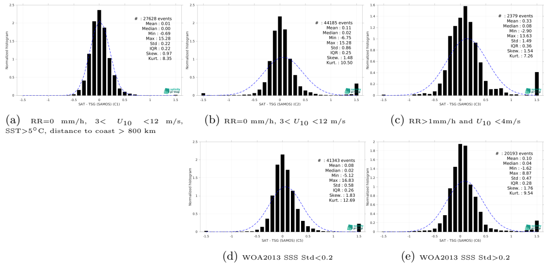
Figure 13: Normalized histogram of \Delta SSS (CCI SSS L4 Merged-OI v4.4 - 7-day running (ESA) - TSG (SAMOS)) for 5 different subdatasets corresponding to: RR=0 mm/h, 3 < U_{10} < 12 m/s, SST >5^\circ\text{C} , distance to coast > 800 km (a), RR=0 mm/h, 3 < U_{10} < 12 m/s (b), RR >1 mm/h and U_{10} < 4 m/s (c), WOA2013 SSS Std <0.2 (d), WOA2013 SSS Std >0.2 (e).
