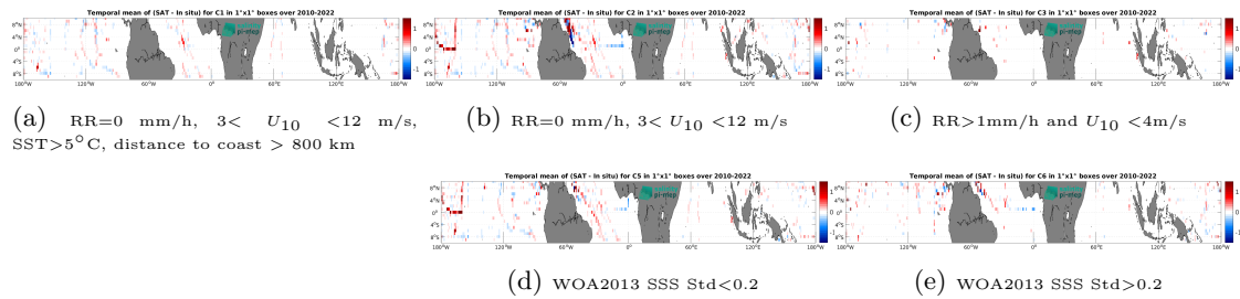
Figure 12: Temporal mean gridded over spatial boxes of size 1^\circ \times 1^\circ of \Delta SSS (CCI SSS L4 Merged-OI v4.4 - 7-day running (ESA) - TSG (SAMOS)) for 5 different subdatasets corresponding to: RR=0 mm/h, 3 < U_{10} < 12 m/s, SST >5^\circ\text{C} , distance to coast > 800 km (a), RR=0 mm/h, 3 < U_{10} < 12 m/s (b), RR >1 mm/h and U_{10} < 4 m/s (c), WOA2013 SSS Std <0.2 (d), WOA2013 SSS Std >0.2 (e).
