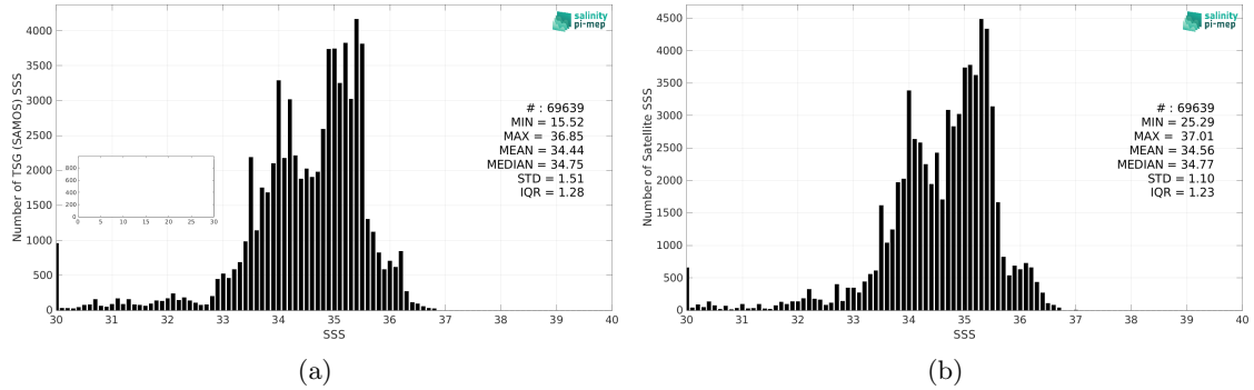
Figure 2: Histograms of SSS from TSG (SAMOS) (a) and CCI SSS L4 Merged-OI v4.4 - 7-day running (ESA) (b) considering all match-up pairs per bins of 0.1 over the Equatorial Ocean 10N-10S Pi-MEP region and for the full satellite product period.
