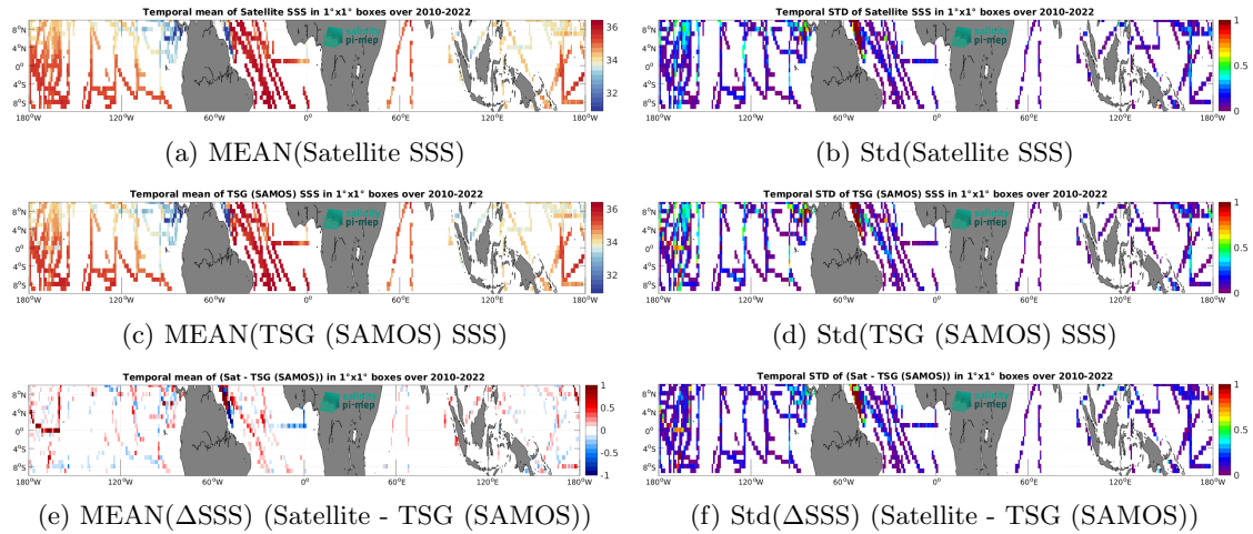
Figure 6: Temporal mean (left) and Std (right) of SSS from CCI SSS L4 Merged-OI v4.4 - 7-day running (ESA) (top), TSG (SAMOS) in situ dataset (middle), and of \Delta SSS (Satellite - TSG (SAMOS)). Only match-up pairs are used to generate these maps.
