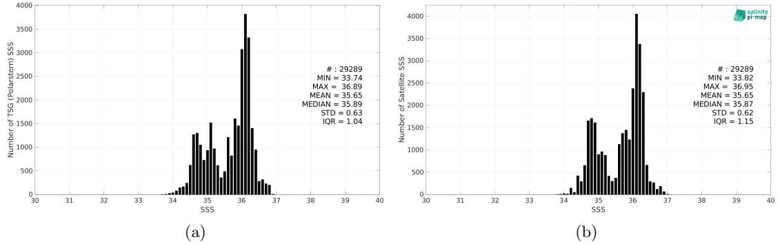
Figure 2: Histograms of SSS from TSG (Polarstern) (a) and CCI SSS L4 Merged-OI v4.4 - 7-day running (ESA) (b) considering all match-up pairs per bins of 0.1 over the Equatorial Ocean 10N-10S Pi-MEP region and for the full satellite product period.
