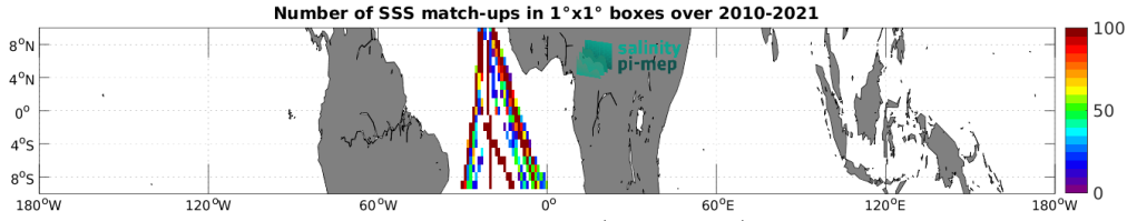
Figure 4: Number of SSS match-ups between TSG (Polarstern) SSS and the CCI SSS L4 Merged-OI v4.4 - 7-day running (ESA) SSS product for the Equatorial Ocean 10N-10S Pi-MEP region over 1^\circ \times 1^\circ boxes and for the full satellite product period.
