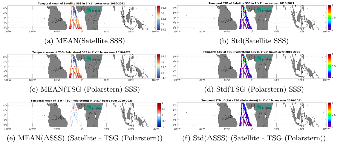
Figure 6: Temporal mean (left) and Std (right) of SSS from CCI SSS L4 Merged-OI v4.4 - 7-day running (ESA) (top), TSG (Polarstern) (middle), and of \Delta SSS (Satellite - TSG (Polarstern)). Only match-up pairs are used to generate these maps.
