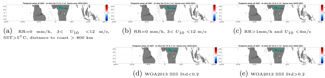
Figure 12: Temporal mean gridded over spatial boxes of size 1^\circ \times 1^\circ of \Delta SSS (CCI SSS L4 Merged-OI v4.4 - 7-day running (ESA) - TSG (Polarstern)) for 5 different subdatasets corresponding to: RR=0 mm/h, 3 < U_{10} < 12 m/s, SST >5^\circ C, distance to coast > 800 km (a), RR=0 mm/h, 3 < U_{10} < 12 m/s (b), RR >1 mm/h and U_{10} < 4 m/s (c), WOA2013 SSS Std <0.2 (d), WOA2013 SSS Std >0.2 (e).
