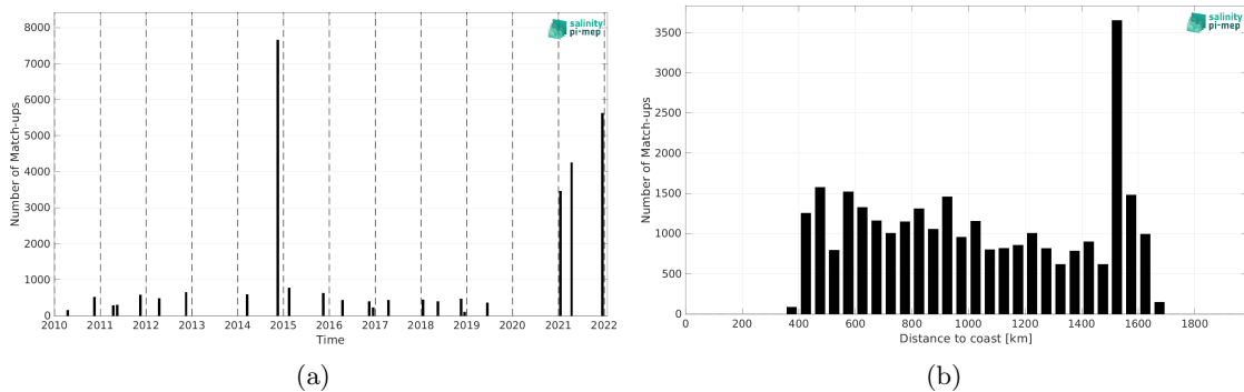
Figure 1: Number of match-ups between TSG (Polarstern) and CCI SSS L4 Merged-OI v4.4 - 7-day running (ESA) SSS as a function of time (a) and as function of the distance to coast (b) over the Equatorial Ocean 10N-10S Pi-MEP region and for the full satellite product period.
