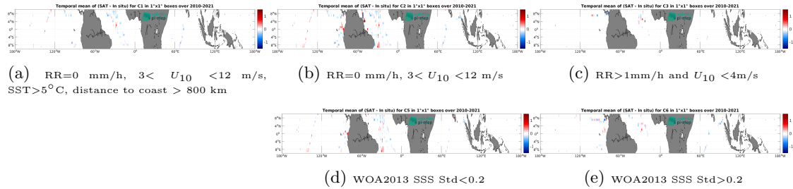
Figure 12: Temporal mean gridded over spatial boxes of size 1^{\circ}\times 1^{\circ} of \Delta SSS (CCI SSS L4 Merged-OI v4.4 - 7-day running (ESA) - TSG (GOSUD-Sailing-ship)) for 5 different subdatasets corresponding to:RR=0 mm/h, 3 < U_{10} < 12 m/s, SST >5^{\circ}\text{C} , distance to coast > 800 km (a), RR=0 mm/h, 3 < U_{10} < 12 m/s (b), RR >1 mm/h and U_{10} < 4 m/s (c), WOA2013 SSS Std <0.2 (d), WOA2013 SSS Std >0.2 (e).
