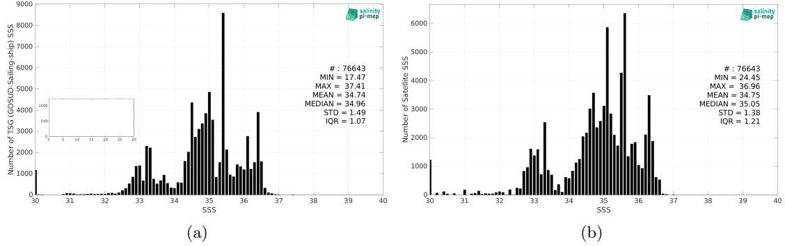
Figure 2: Histograms of SSS from TSG (GOSUD-Sailing-ship) (a) and CCI SSS L4 Merged-OI v4.4 - 7-day running (ESA) (b) considering all match-up pairs per bins of 0.1 over the Equatorial Ocean 10N-10S Pi-MEP region and for the full satellite product period.
