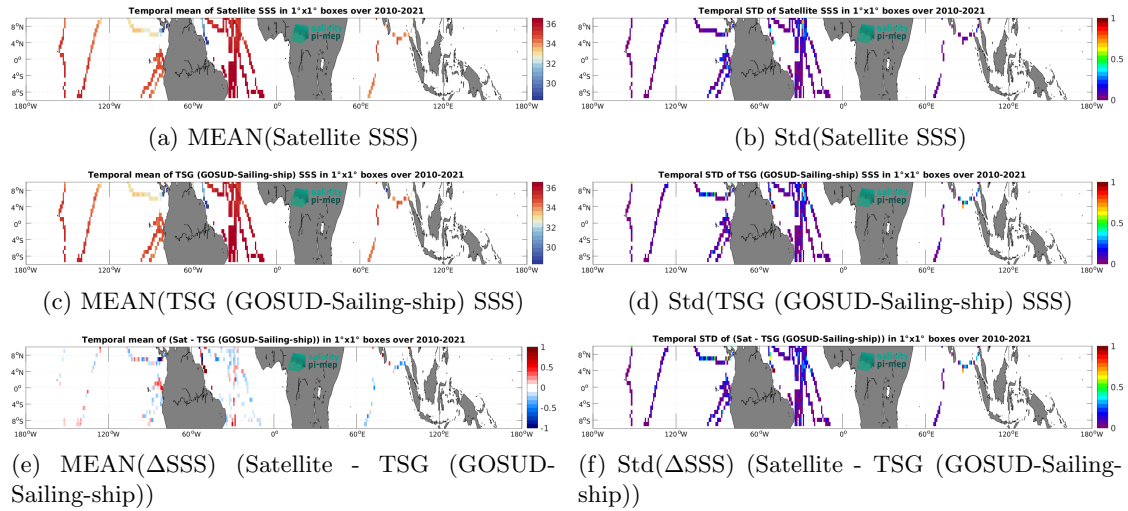
Figure 6: Temporal mean (left) and Std (right) of SSS from CCI SSS L4 Merged-OI v4.4 - 7-day running (ESA) (top), TSG (GOSUD-Sailing-ship) (middle), and of \Delta SSS (Satellite - TSG (GOSUD-Sailing-ship)). Only match-up pairs are used to generate these maps.
