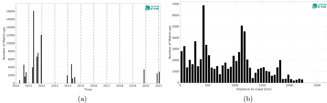
Figure 1: Number of match-ups between TSG (GOSUD-Sailing-ship) and CCI SSS L4 Merged-OI v4.4 - 7-day running (ESA) SSS as a function of time (a) and as function of the distance to coast (b) over the Equatorial Ocean 10N-10S Pi-MEP region and for the full satellite product period.
