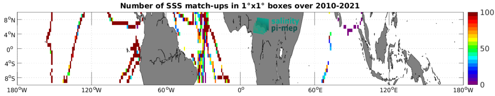
Figure 4: Number of SSS match-ups between TSG (GOSUD-Sailing-ship) SSS and the CCI SSS L4 Merged-OI v4.4 - 7-day running (ESA) SSS product for the Equatorial Ocean 10N-10S Pi-MEP region over 1^\circ \times 1^\circ boxes and for the full satellite product period.
