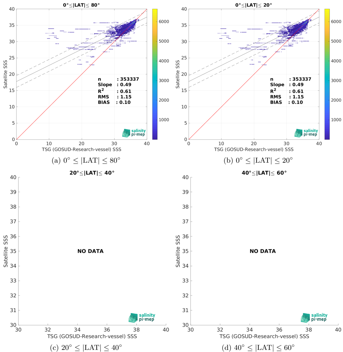
Figure 9: Contour maps of the concentration of CCI SSS L4 Merged-OI v4.4 - 7-day running (ESA) SSS (y-axis) versus TSG (GOSUD-Research-vessel) SSS (x-axis) at match-up pairs for different latitude bands. For each plot, the red line shows x=y . The black thin and dashed lines indicate a linear fit through the data cloud and the \pm 95\% confidence levels, respectively. The number match-up pairs n , the slope and R^2 coefficient of the linear fit, the root mean square (RMS) and the mean bias between satellite and in situ data are indicated for each latitude band in each plots.
