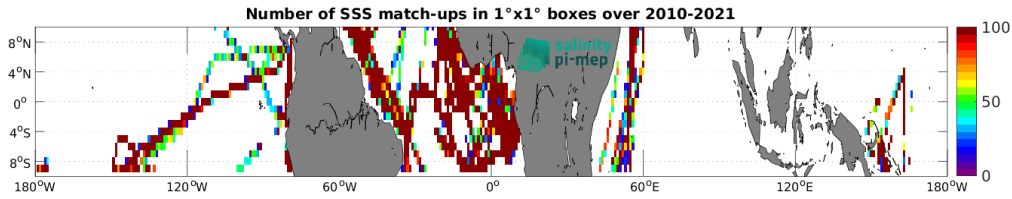
Figure 4: Number of SSS match-ups between TSG (GOSUD-Research-vessel) SSS and the CCI SSS L4 Merged-OI v4.4 - 7-day running (ESA) SSS product for the Equatorial Ocean 10N-10S Pi-MEP region over 1^\circ \times 1^\circ boxes and for the full satellite product period.
