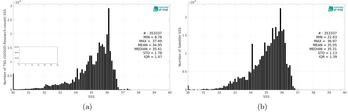
Figure 2: Histograms of SSS from TSG (GOSUD-Research-vessel) (a) and CCI SSS L4 Merged-OI v4.4 - 7-day running (ESA) (b) considering all match-up pairs per bins of 0.1 over the Equatorial Ocean 10N-10S Pi-MEP region and for the full satellite product period.
