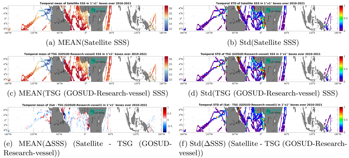
Figure 6: Temporal mean (left) and Std (right) of SSS from CCI SSS L4 Merged-OI v4.4 - 7-day running (ESA) (top), TSG (GOSUD-Research-vessel) (middle), and of \Delta SSS (Satellite - TSG (GOSUD-Research-vessel)). Only match-up pairs are used to generate these maps.
