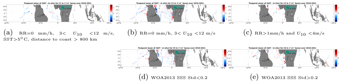
Figure 12: Temporal mean gridded over spatial boxes of size 1^\circ \times 1^\circ of \Delta SSS (CCI SSS L4 Merged-OI v4.4 - 7-day running (ESA) - TSG (GOSUD-Research-vessel)) for 5 different subdatasets corresponding to:RR=0 mm/h, 3 < U_{10} < 12 m/s, SST >5^\circ C, distance to coast > 800 km (a), RR=0 mm/h, 3 < U_{10} < 12 m/s (b), RR >1 mm/h and U_{10} < 4 m/s (c), WOA2013 SSS Std <0.2 (d), WOA2013 SSS Std >0.2 (e).
