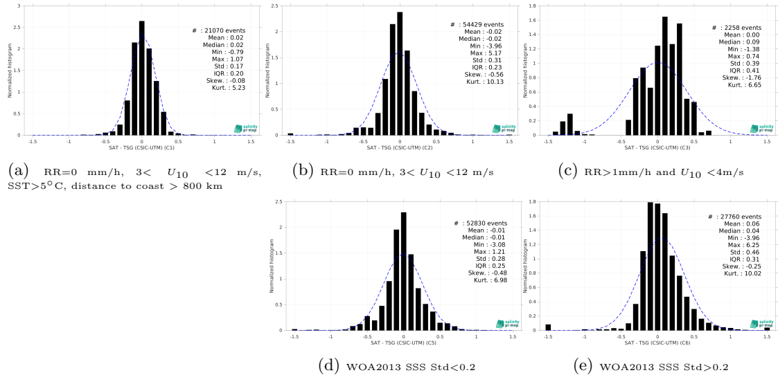
Figure 13: Normalized histogram of \Delta SSS (CCI SSS L4 Merged-OI v4.4 - 7-day running (ESA) - TSG (CSIC-UTM)) for 5 different subdatasets corresponding to: RR=0 mm/h, 3 < U_{10} < 12 m/s, SST >5^\circ C, distance to coast > 800 km (a), RR=0 mm/h, 3 < U_{10} < 12 m/s (b), RR >1 mm/h and U_{10} < 4 m/s (c), WOA2013 SSS Std <0.2 (d), WOA2013 SSS Std >0.2 (e).
