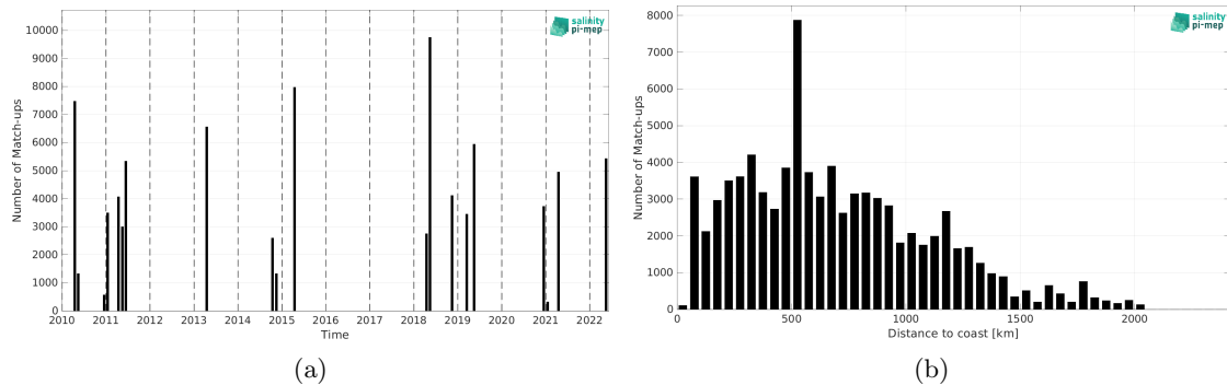
Figure 1: Number of match-ups between TSG (CSIC-UTM) and CCI SSS L4 Merged-OI v4.4 - 7-day running (ESA) SSS as a function of time (a) and as function of the distance to coast (b) over the Equatorial Ocean 10N-10S Pi-MEP region and for the full satellite product period.
