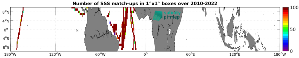
Figure 4: Number of SSS match-ups between TSG (CSIC-UTM) SSS and the CCI SSS L4 Merged-OI v4.4 - 7-day running (ESA) SSS product for the Equatorial Ocean 10N-10S Pi-MEP region over 1^\circ \times 1^\circ boxes and for the full satellite product period.
