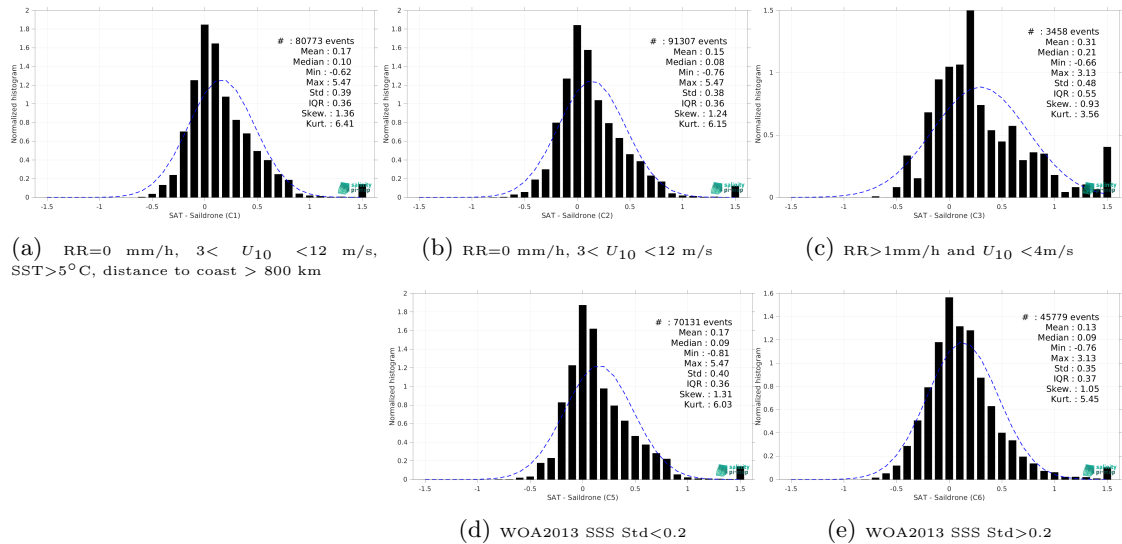
Figure 13: Normalized histogram of \Delta SSS (CCI SSS L4 Merged-OI v4.4 - 7-day running (ESA) - Saildrone) for 5 different subdatasets corresponding to: RR=0 mm/h, 3 < U_{10} < 12 m/s, SST >5^\circ C, distance to coast > 800 km (a), RR=0 mm/h, 3 < U_{10} < 12 m/s (b), RR >1 mm/h and U_{10} < 4 m/s (c), WOA2013 SSS Std <0.2 (d), WOA2013 SSS Std >0.2 (e).
