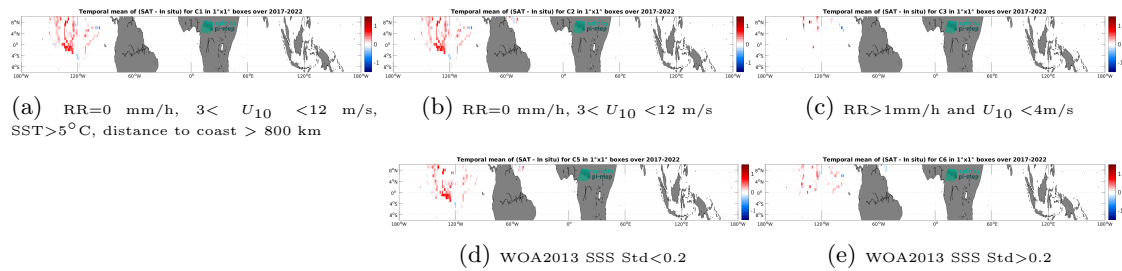
Figure 12: Temporal mean gridded over spatial boxes of size 1^\circ \times 1^\circ of \Delta SSS (CCI SSS L4 Merged-OI v4.4 - 7-day running (ESA) - Saildrone) for 5 different subdatasets corresponding to: RR=0 mm/h, 3 < U_{10} < 12 m/s, SST >5^\circ C, distance to coast > 800 km (a), RR=0 mm/h, 3 < U_{10} < 12 m/s (b), RR >1 mm/h and U_{10} < 4 m/s (c), WOA2013 SSS Std <0.2 (d), WOA2013 SSS Std >0.2 (e).
