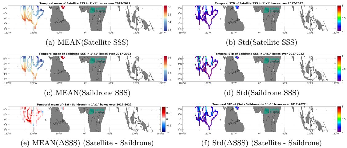
Figure 6: Temporal mean (left) and Std (right) of SSS from CCI SSS L4 Merged-OI v4.4 - 7-day running (ESA) (top), Saildrone (middle), and of \Delta SSS (Satellite - Saildrone). Only match-up pairs are used to generate these maps.
