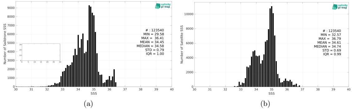
Figure 2: Histograms of SSS from Saildrone (a) and CCI SSS L4 Merged-OI v4.4 - 7-day running (ESA) (b) considering all match-up pairs per bins of 0.1 over the Equatorial Ocean 10N-10S Pi-MEP region and for the full satellite product period.
