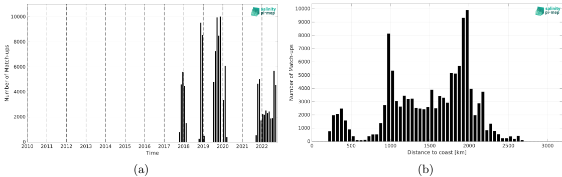
Figure 1: Number of match-ups between Saildrone and CCI SSS L4 Merged-OI v4.4 - 7-day running (ESA) SSS as a function of time (a) and as function of the distance to coast (b) over the Equatorial Ocean 10N-10S Pi-MEP region and for the full satellite product period.
