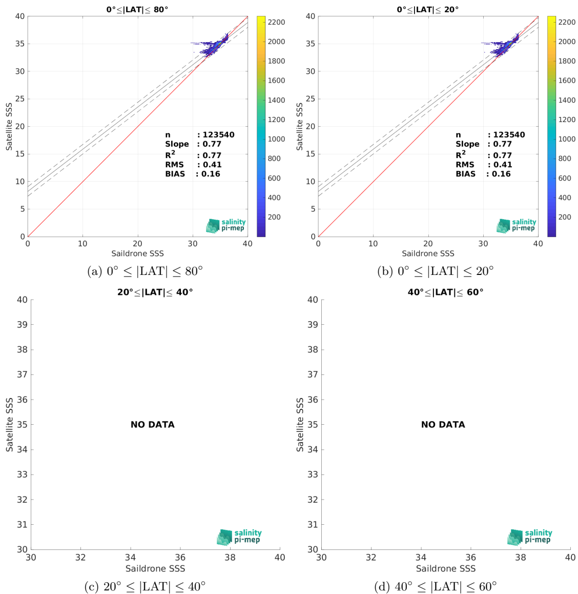
Figure 9: Contour maps of the concentration of CCI SSS L4 Merged-OI v4.4 - 7-day running (ESA) SSS (y-axis) versus Saildrone SSS (x-axis) at match-up pairs for different latitude bands. For each plot, the red line shows x=y . The black thin and dashed lines indicate a linear fit through the data cloud and the \pm 95\% confidence levels, respectively. The number match-up pairs n , the slope and R^2 coefficient of the linear fit, the root mean square (RMS) and the mean bias between satellite and in situ data are indicated for each latitude band in each plots.
