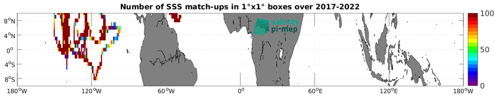
Figure 4: Number of SSS match-ups between Saildrone SSS and the CCI SSS L4 Merged-OI v4.4 - 7-day running (ESA) SSS product for the Equatorial Ocean 10N-10S Pi-MEP region over 1^\circ \times 1^\circ boxes and for the full satellite product period.
