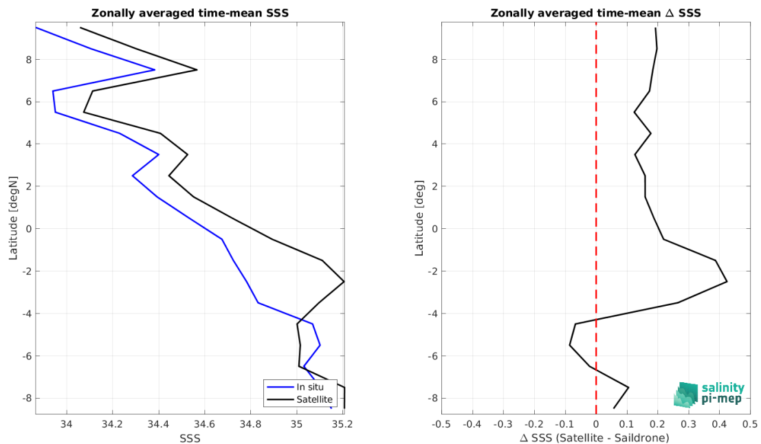
Figure 8: Left panel: Zonal mean SSS from CCI SSS L4 Merged-OI v4.4 - 7-day running (ESA) satellite product (black) and from Sairdrone (blue). Right panel: Zonal mean of \Delta SSS (Satellite - Sairdrone) for all the collected Pi-MEP match-up pairs estimated over the full satellite product period.
