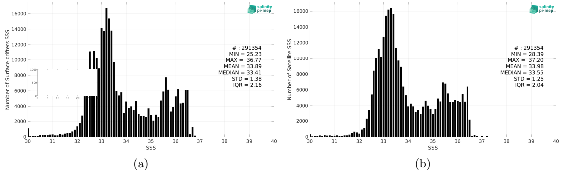
Figure 2: Histograms of SSS from Surface drifters (a) and CCI SSS L4 Merged-OI v4.4 - 7-day running (ESA) (b) considering all match-up pairs per bins of 0.1 over the Equatorial Ocean 10N-10S Pi-MEP region and for the full satellite product period.
