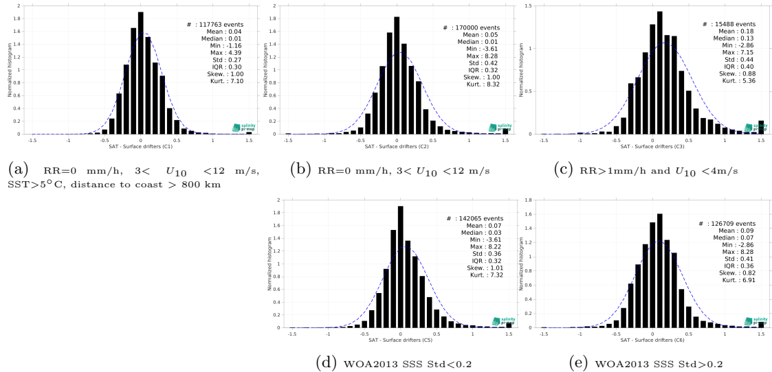
Figure 12: Normalized histogram of \Delta SSS (CCI SSS L4 Merged-OI v4.4 - 7-day running (ESA) - Surface drifters) for 5 different subdatasets corresponding to: RR=0 mm/h, 3 < U_{10} < 12 m/s, SST >5^\circ C, distance to coast > 800 km (a), RR=0 mm/h, 3 < U_{10} < 12 m/s (b), RR >1 mm/h and U_{10} < 4 m/s (c), WOA2013 SSS Std <0.2 (d), WOA2013 SSS Std >0.2 (e).
