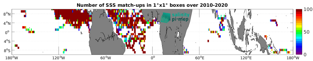
Figure 3: Number of SSS match-ups between Surface drifters SSS and the CCI SSS L4 Merged-OI v4.4 - 7-day running (ESA) SSS product for the Equatorial Ocean 10N-10S Pi-MEP region over 1^\circ \times 1^\circ boxes and for the full satellite product period.
