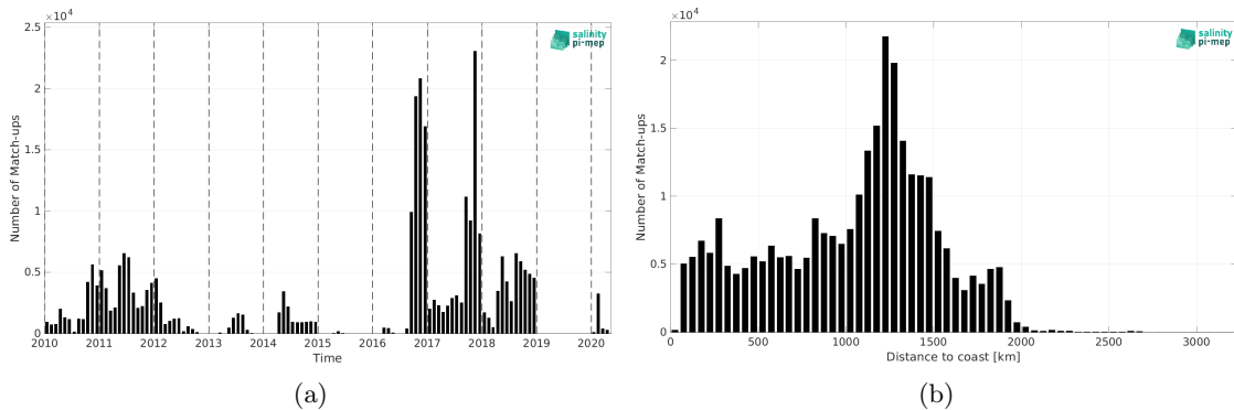
Figure 1: Number of match-ups between Surface drifters and CCI SSS L4 Merged-OI v4.4 - 7-day running (ESA) SSS as a function of time (a) and as function of the distance to coast (b) over the Equatorial Ocean 10N-10S Pi-MEP region and for the full satellite product period.
