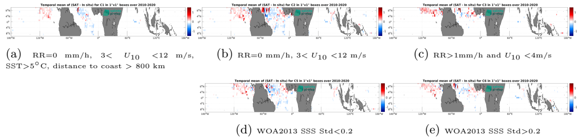
Figure 11: Temporal mean gridded over spatial boxes of size 1^\circ \times 1^\circ of \Delta SSS (CCI SSS L4 Merged-OI v4.4 - 7-day running (ESA) - Surface drifters) for 5 different subdatasets corresponding to: RR=0 mm/h, 3 < U_{10} < 12 m/s, SST >5^\circ C, distance to coast > 800 km (a), RR=0 mm/h, 3 < U_{10} < 12 m/s (b), RR >1 mm/h and U_{10} < 4 m/s (c), WOA2013 SSS Std <0.2 (d), WOA2013 SSS Std >0.2 (e).
