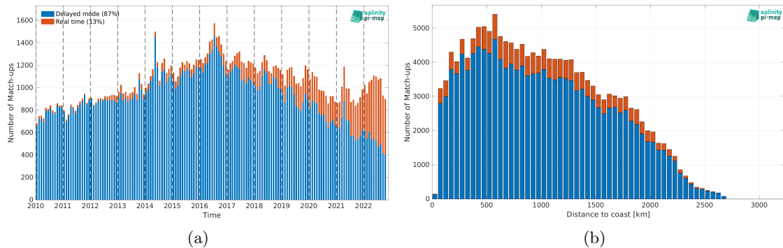
Figure 1: Number of match-ups between Argo and CCI SSS L4 Merged-OI v4.4 - 7-day running (ESA) SSS as a function of time (a) and as function of the distance to coast (b) over the Equatorial Ocean 10N-10S Pi-MEP region and for the full satellite product period.
