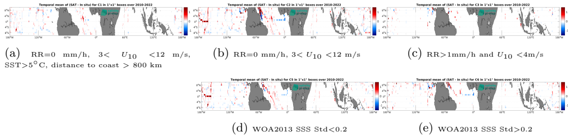
Figure 12: Temporal mean gridded over spatial boxes of size 1^\circ \times 1^\circ of \Delta SSS (CCI SSS L4 Merged-OI v4.4 - 30-day running (ESA) - TSG (SAMOS)) for 5 different subdatasets corresponding to:RR=0 mm/h, 3 < U_{10} < 12 m/s, SST >5^\circ C, distance to coast > 800 km (a), RR=0 mm/h, 3 < U_{10} < 12 m/s (b), RR >1 mm/h and U_{10} < 4 m/s (c), WOA2013 SSS Std <0.2 (d), WOA2013 SSS Std >0.2 (e).
