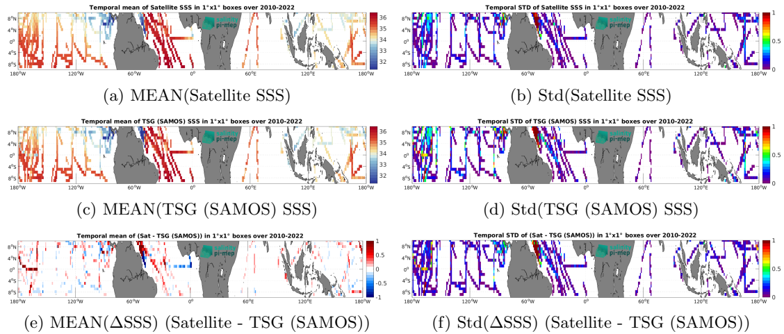
Figure 6: Temporal mean (left) and Std (right) of SSS from CCI SSS L4 Merged-OI v4.4 - 30-day running (ESA) (top), TSG (SAMOS) ( in situ ) dataset (middle), and of \Delta SSS (Satellite - TSG (SAMOS)). Only match-up pairs are used to generate these maps.
