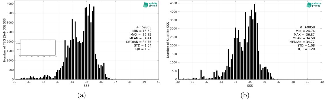
Figure 2: Histograms of SSS from TSG (SAMOS) (a) and CCI SSS L4 Merged-OI v4.4 - 30-day running (ESA) (b) considering all match-up pairs per bins of 0.1 over the Equatorial Ocean 10N-10S Pi-MEP region and for the full satellite product period.
