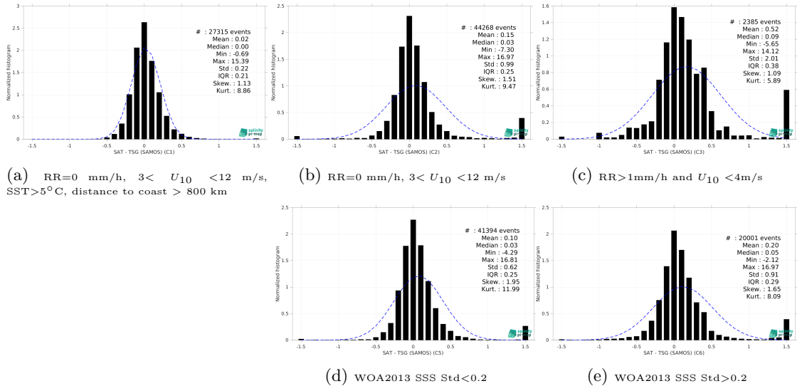
Figure 13: Normalized histogram of \Delta SSS (CCI SSS L4 Merged-OI v4.4 - 30-day running (ESA) - TSG (SAMOS)) for 5 different subdatasets corresponding to: RR=0 mm/h, 3 < U_{10} < 12 m/s, SST >5^\circ C, distance to coast > 800 km (a), RR=0 mm/h, 3 < U_{10} < 12 m/s (b), RR >1 mm/h and U_{10} < 4 m/s (c), WOA2013 SSS Std <0.2 (d), WOA2013 SSS Std >0.2 (e).
