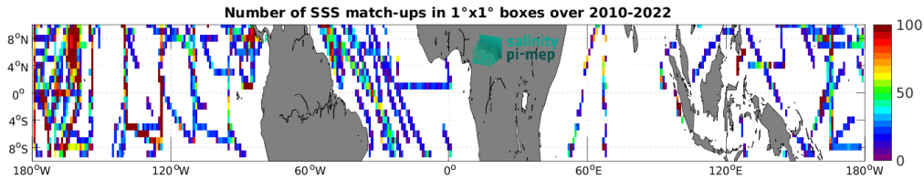
Figure 4: Number of SSS match-ups between TSG (SAMOS) SSS and the CCI SSS L4 Merged-OI v4.4 - 30-day running (ESA) SSS product for the Equatorial Ocean 10N-10S Pi-MEP region over 1^\circ \times 1^\circ boxes and for the full satellite product period.
