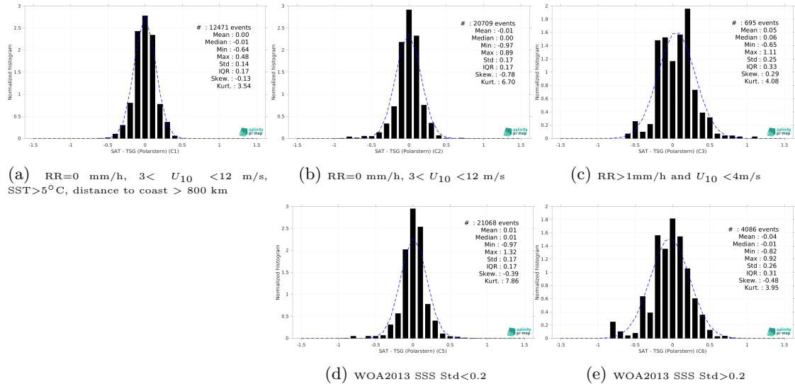
Figure 13: Normalized histogram of \Delta SSS (CCI SSS L4 Merged-OI v4.4 - 30-day running (ESA) - TSG (Polarstern)) for 5 different subdatasets corresponding to: RR=0 mm/h, 3 < U_{10} < 12 m/s, SST >5^\circ C, distance to coast > 800 km (a), RR=0 mm/h, 3 < U_{10} < 12 m/s (b), RR >1 mm/h and U_{10} < 4 m/s (c), WOA2013 SSS Std <0.2 (d), WOA2013 SSS Std >0.2 (e).
