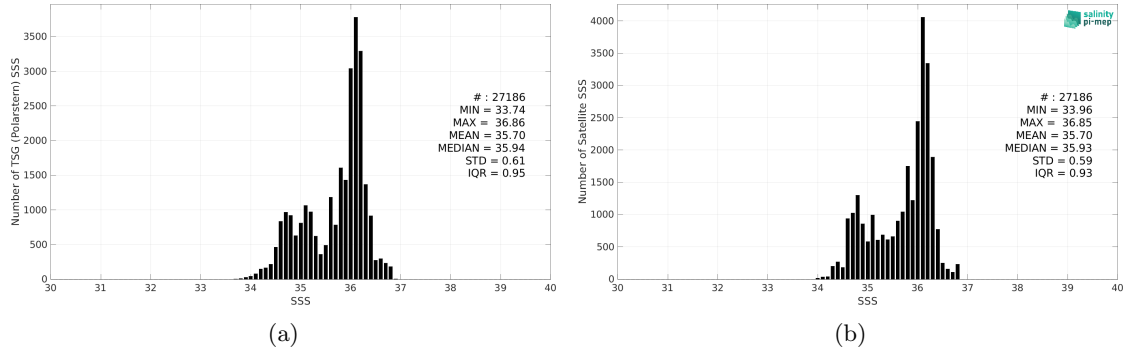
Figure 2: Histograms of SSS from TSG (Polarstern) (a) and CCI SSS L4 Merged-OI v4.4 - 30-day running (ESA) (b) considering all match-up pairs per bins of 0.1 over the Equatorial Ocean 10N-10S Pi-MEP region and for the full satellite product period.
