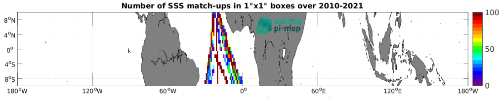
Figure 4: Number of SSS match-ups between TSG (Polarstern) SSS and the CCI SSS L4 Merged-OI v4.4 - 30-day running (ESA) SSS product for the Equatorial Ocean 10N-10S Pi-MEP region over 1^\circ \times 1^\circ boxes and for the full satellite product period.
