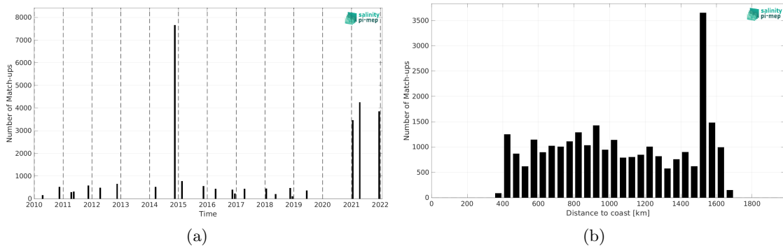
Figure 1: Number of match-ups between TSG (Polarstern) and CCI SSS L4 Merged-OI v4.4 - 30-day running (ESA) SSS as a function of time (a) and as function of the distance to coast (b) over the Equatorial Ocean 10N-10S Pi-MEP region and for the full satellite product period.
