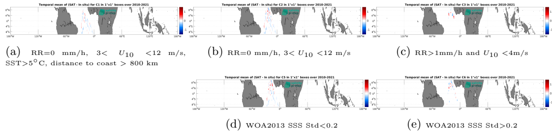
Figure 12: Temporal mean gridded over spatial boxes of size 1^\circ \times 1^\circ of \Delta SSS (CCI SSS L4 Merged-OI v4.4 - 30-day running (ESA) - TSG (Polarstern)) for 5 different subdatasets corresponding to:RR=0 mm/h, 3 < U_{10} < 12 m/s, SST >5^\circ C, distance to coast > 800 km (a), RR=0 mm/h, 3 < U_{10} < 12 m/s (b), RR >1 mm/h and U_{10} < 4 m/s (c), WOA2013 SSS Std <0.2 (d), WOA2013 SSS Std >0.2 (e).
