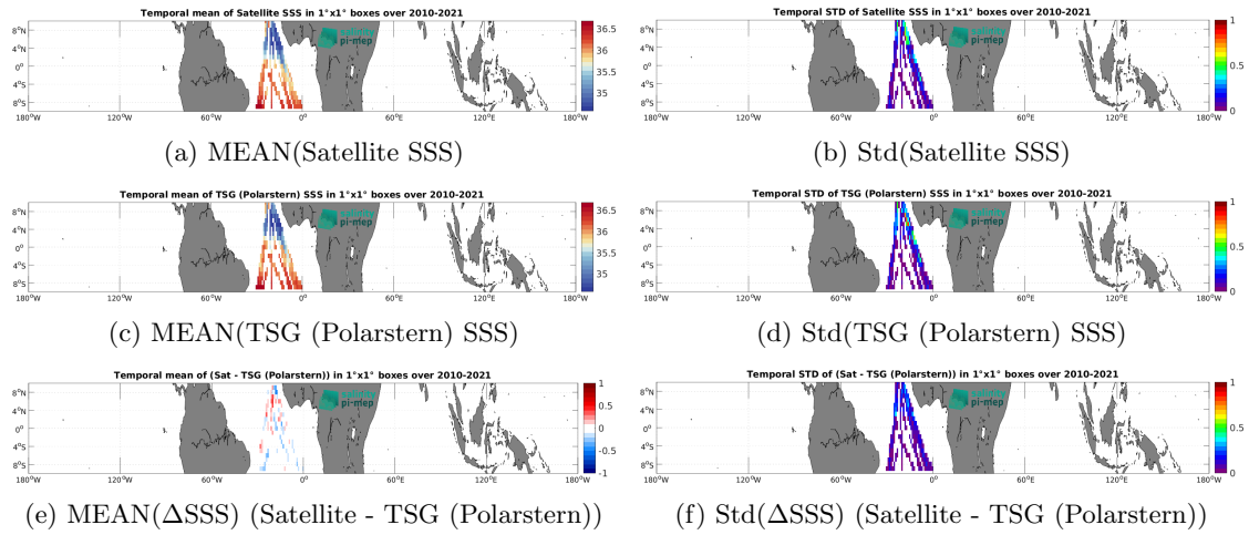
Figure 6: Temporal mean (left) and Std (right) of SSS from CCI SSS L4 Merged-OI v4.4 - 30-day running (ESA) (top), TSG (Polarstern) (middle), and of \Delta SSS (Satellite - TSG (Polarstern)). Only match-up pairs are used to generate these maps.
