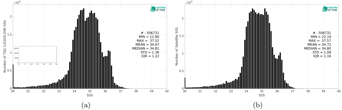
Figure 2: Histograms of SSS from TSG (LEGOS-DM) (a) and CCI SSS L4 Merged-OI v4.4 - 30-day running (ESA) (b) considering all match-up pairs per bins of 0.1 over the Equatorial Ocean 10N-10S Pi-MEP region and for the full satellite product period.
