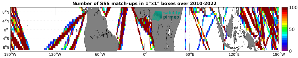
Figure 4: Number of SSS match-ups between TSG (LEGOS-DM) SSS and the CCI SSS L4 Merged-OI v4.4 - 30-day running (ESA) SSS product for the Equatorial Ocean 10N-10S Pi-MEP region over 1^\circ \times 1^\circ boxes and for the full satellite product period.
