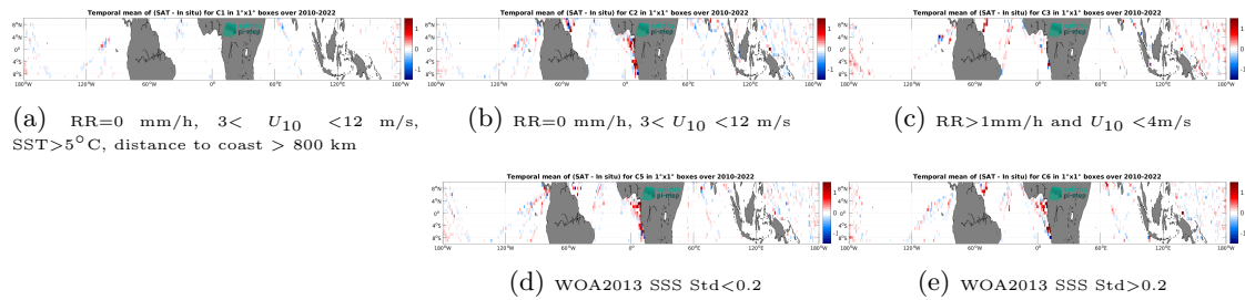
Figure 12: Temporal mean gridded over spatial boxes of size 1^\circ \times 1^\circ of \Delta SSS (CCI SSS L4 Merged-OI v4.4 - 30-day running (ESA) - TSG (LEGOS-DM)) for 5 different subdatasets corresponding to: RR=0 mm/h, 3 < U_{10} < 12 m/s, SST >5^\circ C, distance to coast > 800 km (a), RR=0 mm/h, 3 < U_{10} < 12 m/s (b), RR >1 mm/h and U_{10} < 4 m/s (c), WOA2013 SSS Std <0.2 (d), WOA2013 SSS Std >0.2 (e).
