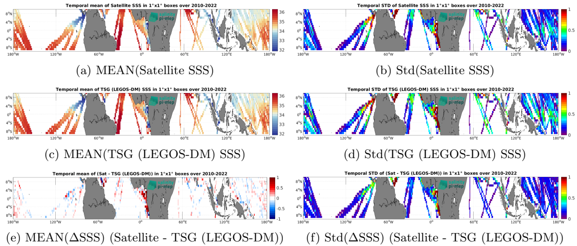
Figure 6: Temporal mean (left) and Std (right) of SSS from CCI SSS L4 Merged-OI v4.4 - 30-day running (ESA) (top), TSG (LEGOS-DM) in situ dataset (middle), and of \Delta SSS (Satellite - TSG (LEGOS-DM)). Only match-up pairs are used to generate these maps.
