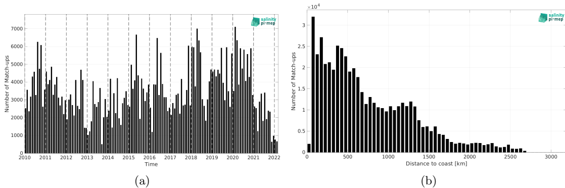
Figure 1: Number of match-ups between TSG (LEGOS-DM) and CCI SSS L4 Merged-OI v4.4 - 30-day running (ESA) SSS as a function of time (a) and as function of the distance to coast (b) over the Equatorial Ocean 10N-10S Pi-MEP region and for the full satellite product period.
