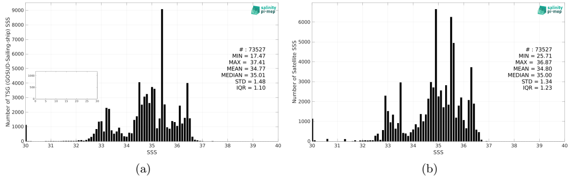
Figure 2: Histograms of SSS from TSG (GOSUD-Sailing-ship) (a) and CCI SSS L4 Merged-OI v4.4 - 30-day running (ESA) (b) considering all match-up pairs per bins of 0.1 over the Equatorial Ocean 10N-10S Pi-MEP region and for the full satellite product period.
