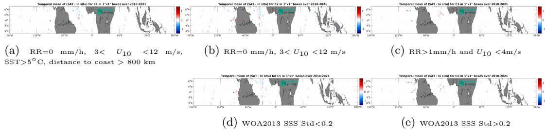
Figure 12: Temporal mean gridded over spatial boxes of size 1^\circ \times 1^\circ of \Delta SSS (CCI SSS L4 Merged-OI v4.4 - 30-day running (ESA) - TSG (GOSUD-Sailing-ship)) for 5 different subdatasets corresponding to: RR=0 mm/h, 3 < U_{10} < 12 m/s, SST > 5^\circ\text{C} , distance to coast > 800 km (a), RR=0 mm/h, 3 < U_{10} < 12 m/s (b), RR > 1 mm/h and U_{10} < 4 m/s (c), WOA2013 SSS Std < 0.2 (d), WOA2013 SSS Std > 0.2 (e).
