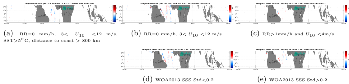
Figure 12: Temporal mean gridded over spatial boxes of size 1^\circ \times 1^\circ of \Delta SSS (CCI SSS L4 Merged-OI v4.4 - 30-day running (ESA) - TSG (CSIC-UTM)) for 5 different subdatasets corresponding to: RR=0 mm/h, 3 < U_{10} < 12 m/s, SST >5^\circ\text{C} , distance to coast > 800 km (a), RR=0 mm/h, 3 < U_{10} < 12 m/s (b), RR >1 mm/h and U_{10} < 4 m/s (c), WOA2013 SSS Std <0.2 (d), WOA2013 SSS Std >0.2 (e).
