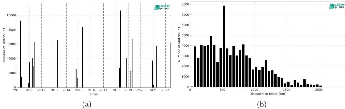
Figure 1: Number of match-ups between TSG (CSIC-UTM) and CCI SSS L4 Merged-OI v4.4 - 30-day running (ESA) SSS as a function of time (a) and as function of the distance to coast (b) over the Equatorial Ocean 10N-10S Pi-MEP region and for the full satellite product period.
