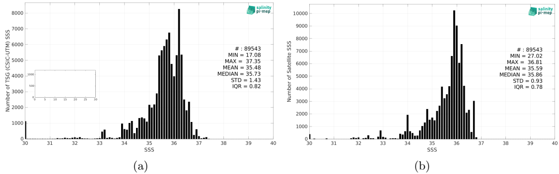
Figure 2: Histograms of SSS from TSG (CSIC-UTM) (a) and CCI SSS L4 Merged-OI v4.4 - 30-day running (ESA) (b) considering all match-up pairs per bins of 0.1 over the Equatorial Ocean 10N-10S Pi-MEP region and for the full satellite product period.
