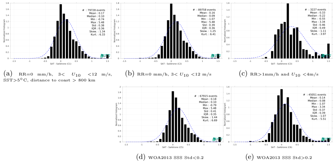
Figure 13: Normalized histogram of \Delta\text{SSS} (CCI SSS L4 Merged-OI v4.4 - 30-day running (ESA) - Saildrone) for 5 different subdatasets corresponding to: RR=0 mm/h, 3 < U_{10} < 12 m/s, SST >5^\circ\text{C} , distance to coast > 800 km (a), RR=0 mm/h, 3 < U_{10} < 12 m/s (b), RR >1 mm/h and U_{10} < 4 m/s (c), WOA2013 SSS Std <0.2 (d), WOA2013 SSS Std >0.2 (e).
