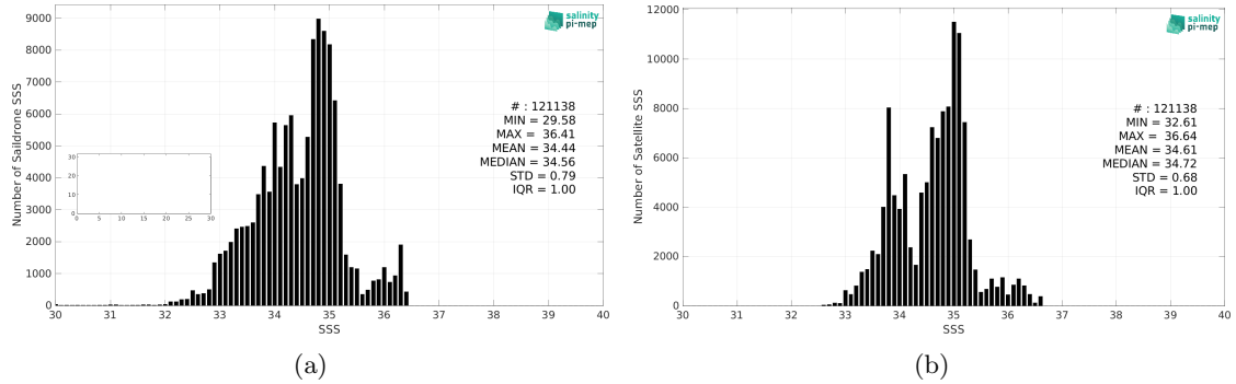
Figure 2: Histograms of SSS from Saildrone (a) and CCI SSS L4 Merged-OI v4.4 - 30-day running (ESA) (b) considering all match-up pairs per bins of 0.1 over the Equatorial Ocean 10N-10S Pi-MEP region and for the full satellite product period.
