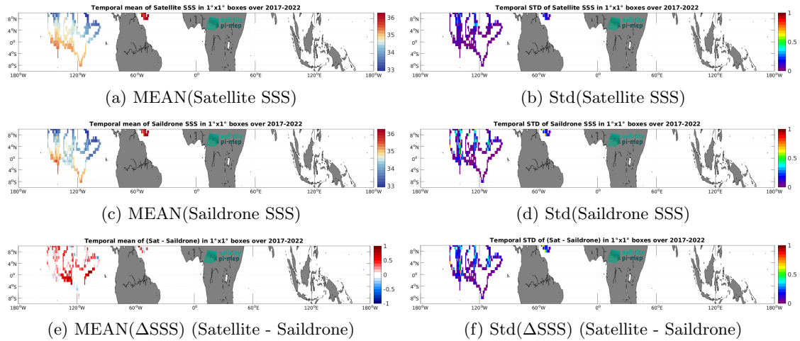
Figure 6: Temporal mean (left) and Std (right) of SSS from CCI SSS L4 Merged-OI v4.4 - 30-day running (ESA) (top), Saildrone (middle), and of \Delta SSS (Satellite - Saildrone). Only match-up pairs are used to generate these maps.
