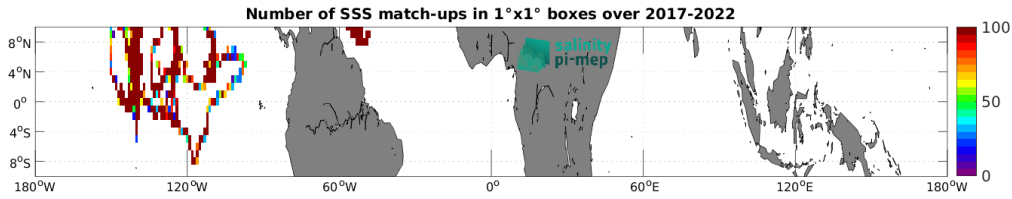
Figure 4: Number of SSS match-ups between Saildrone SSS and the CCI SSS L4 Merged-OI v4.4 - 30-day running (ESA) SSS product for the Equatorial Ocean 10N-10S Pi-MEP region over 1^\circ \times 1^\circ boxes and for the full satellite product period.
