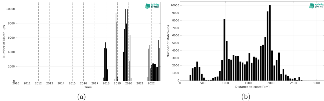
Figure 1: Number of match-ups between Saildrone and CCI SSS L4 Merged-OI v4.4 - 30-day running (ESA) SSS as a function of time (a) and as function of the distance to coast (b) over the Equatorial Ocean 10N-10S Pi-MEP region and for the full satellite product period.
