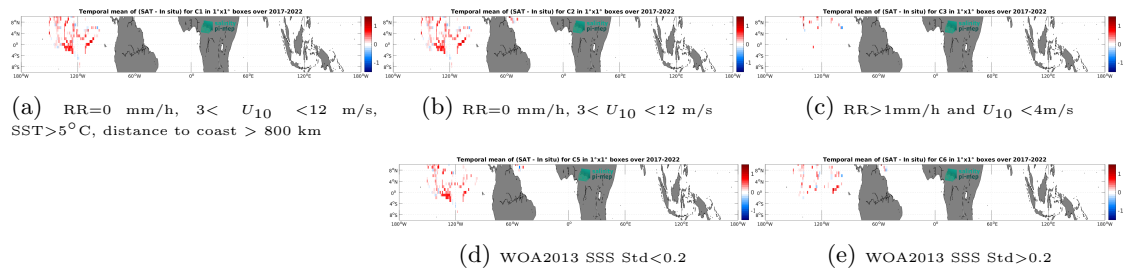
Figure 12: Temporal mean gridded over spatial boxes of size 1^\circ \times 1^\circ of \Delta\text{SSS} (CCI SSS L4 Merged-OI v4.4 - 30-day running (ESA) - Saildrone) for 5 different subdatasets corresponding to:RR=0 mm/h, 3 < U_{10} < 12 m/s, SST >5^\circ\text{C} , distance to coast > 800 km (a), RR=0 mm/h, 3 < U_{10} < 12 m/s (b), RR >1 mm/h and U_{10} < 4 m/s (c), WOA2013 SSS Std <0.2 (d), WOA2013 SSS Std >0.2 (e).
