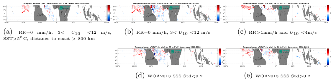
Figure 11: Temporal mean gridded over spatial boxes of size 1^\circ \times 1^\circ of \Delta\text{SSS} (CCI SSS L4 Merged-OI v4.4 - 30-day running (ESA) - Surface drifters) for 5 different subdatasets corresponding to:RR=0 mm/h, 3 < U_{10} < 12 m/s, SST >5^\circ\text{C} , distance to coast > 800 km (a), RR=0 mm/h, 3 < U_{10} < 12 m/s (b), RR >1 mm/h and U_{10} < 4 m/s (c), WOA2013 SSS Std <0.2 (d), WOA2013 SSS Std >0.2 (e).
