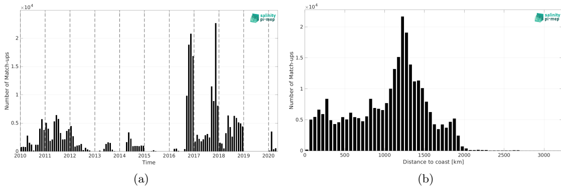
Figure 1: Number of match-ups between Surface drifters and CCI SSS L4 Merged-OI v4.4 - 30-day running (ESA) SSS as a function of time (a) and as function of the distance to coast (b) over the Equatorial Ocean 10N-10S Pi-MEP region and for the full satellite product period.
