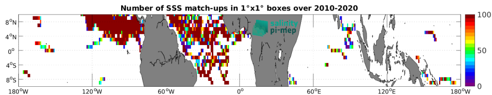
Figure 3: Number of SSS match-ups between Surface drifters SSS and the CCI SSS L4 Merged-OI v4.4 - 30-day running (ESA) SSS product for the Equatorial Ocean 10N-10S Pi-MEP region over 1^\circ \times 1^\circ boxes and for the full satellite product period.
