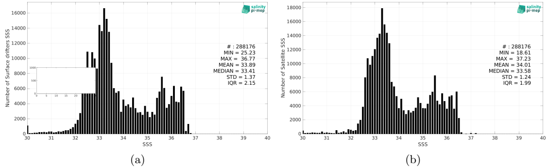
Figure 2: Histograms of SSS from Surface drifters (a) and CCI SSS L4 Merged-OI v4.4 - 30-day running (ESA) (b) considering all match-up pairs per bins of 0.1 over the Equatorial Ocean 10N-10S Pi-MEP region and for the full satellite product period.
