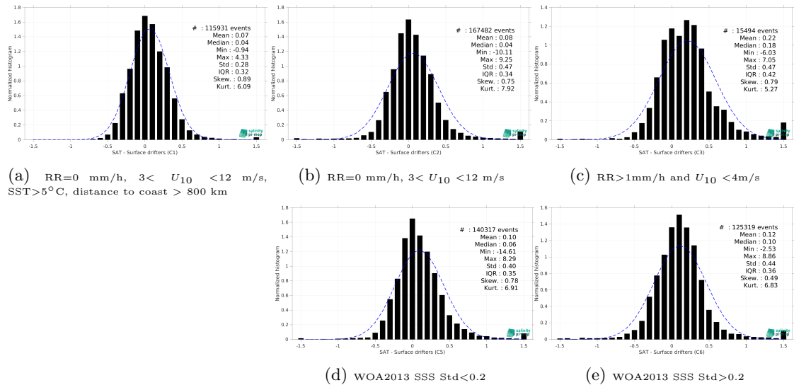
Figure 12: Normalized histogram of \Delta\text{SSS} (CCI SSS L4 Merged-OI v4.4 - 30-day running (ESA) - Surface drifters) for 5 different subdatasets corresponding to: RR=0 mm/h, 3 < U_{10} < 12 m/s, SST >5^\circ\text{C} , distance to coast > 800 km (a), RR=0 mm/h, 3 < U_{10} < 12 m/s (b), RR >1 mm/h and U_{10} < 4 m/s (c), WOA2013 SSS Std <0.2 (d), WOA2013 SSS Std >0.2 (e).
