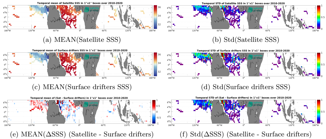
Figure 5: Temporal mean (left) and Std (right) of SSS from CCI SSS L4 Merged-OI v4.4 - 30-day running (ESA) (top), Surface drifters (middle), and of \Delta SSS (Satellite - Surface drifters). Only match-up pairs are used to generate these maps.
