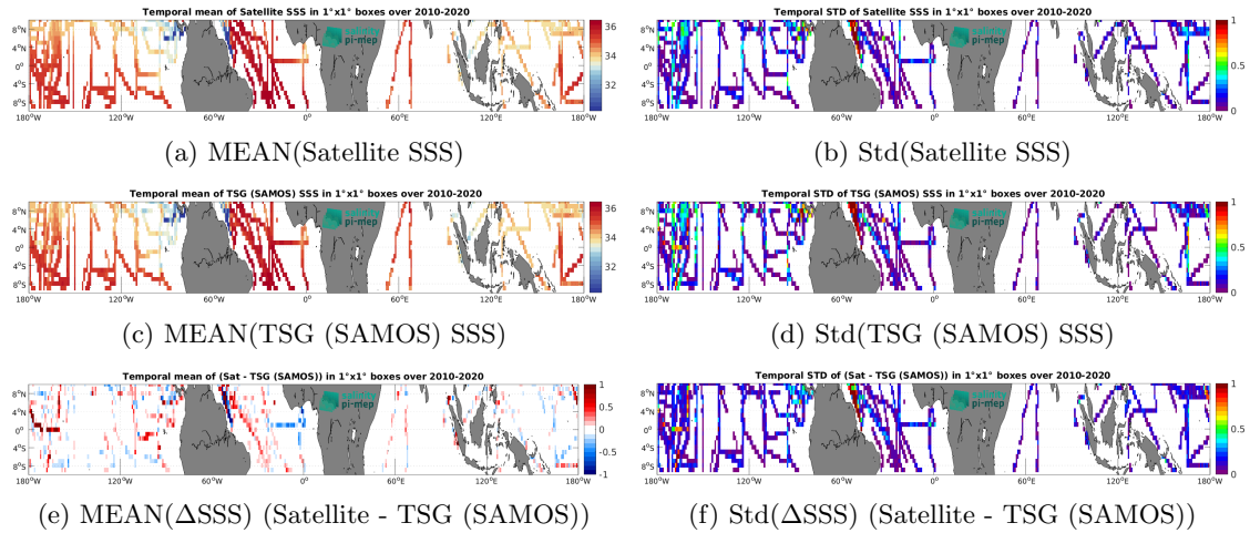
Figure 6: Temporal mean (left) and Std (right) of SSS from CCI SSS L4 Merged-OI v3.2 - 7-day running (ESA) (top), TSG (SAMOS) ( in situ ) dataset (middle), and of \Delta SSS (Satellite - TSG (SAMOS)). Only match-up pairs are used to generate these maps.
