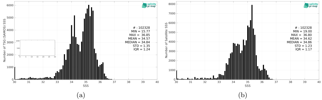
Figure 2: Histograms of SSS from TSG (SAMOS) (a) and CCI SSS L4 Merged-OI v3.2 - 7-day running (ESA) (b) considering all match-up pairs per bins of 0.1 over the Equatorial Ocean 10N-10S Pi-MEP region and for the full satellite product period.
