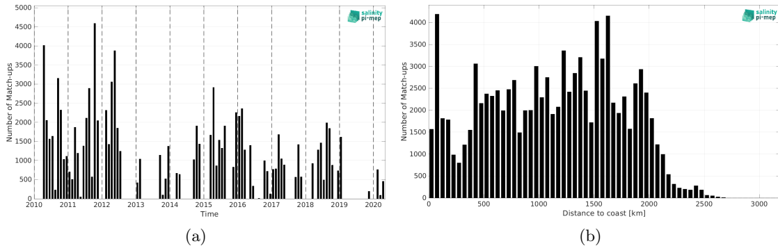
Figure 1: Number of match-ups between TSG (SAMOS) and CCI SSS L4 Merged-OI v3.2 - 7-day running (ESA) SSS as a function of time (a) and as function of the distance to coast (b) over the Equatorial Ocean 10N-10S Pi-MEP region and for the full satellite product period.
