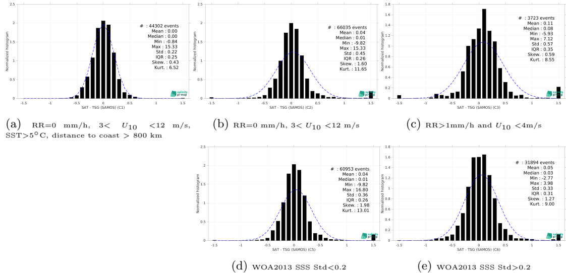
Figure 13: Normalized histogram of \Delta SSS (CCI SSS L4 Merged-OI v3.2 - 7-day running (ESA) - TSG (SAMOS)) for 5 different subdatasets corresponding to: RR=0 mm/h, 3 < U_{10} < 12 m/s, SST >5^\circ\text{C} , distance to coast > 800 km (a), RR=0 mm/h, 3 < U_{10} < 12 m/s (b), RR >1 mm/h and U_{10} < 4 m/s (c), WOA2013 SSS Std <0.2 (d), WOA2013 SSS Std >0.2 (e).
