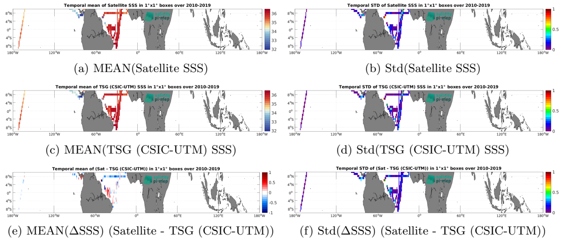
Figure 6: Temporal mean (left) and Std (right) of SSS from CCI SSS L4 Merged-OI v3.2 - 7-day running (ESA) (top), TSG (CSIC-UTM) (middle), and of \Delta SSS (Satellite - TSG (CSIC-UTM)). Only match-up pairs are used to generate these maps.
