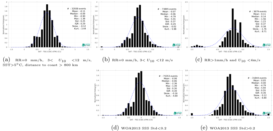
Figure 13: Normalized histogram of \Delta\text{SSS} (CCI SSS L4 Merged-OI v3.2 - 7-day running (ESA) - TSG (CSIC-UTM)) for 5 different subdatasets corresponding to: RR=0 mm/h, 3 < U_{10} < 12 m/s, SST >5^\circ\text{C} , distance to coast > 800 km (a), RR=0 mm/h, 3 < U_{10} < 12 m/s (b), RR >1 mm/h and U_{10} < 4 m/s (c), WOA2013 SSS Std <0.2 (d), WOA2013 SSS Std >0.2 (e).
