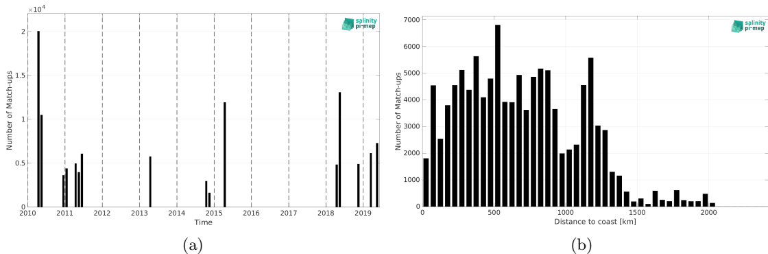
Figure 1: Number of match-ups between TSG (CSIC-UTM) and CCI SSS L4 Merged-OI v3.2 - 7-day running (ESA) SSS as a function of time (a) and as function of the distance to coast (b) over the Equatorial Ocean 10N-10S Pi-MEP region and for the full satellite product period.
