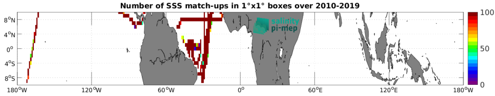
Figure 4: Number of SSS match-ups between TSG (CSIC-UTM) SSS and the CCI SSS L4 Merged-OI v3.2 - 7-day running (ESA) SSS product for the Equatorial Ocean 10N-10S Pi-MEP region over 1^\circ \times 1^\circ boxes and for the full satellite product period.
