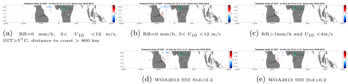
Figure 12: Temporal mean gridded over spatial boxes of size 1^\circ \times 1^\circ of \Delta SSS (CCI SSS L4 Merged-OI v3.2 - 7-day running (ESA) - TSG (CSIC-UTM)) for 5 different subdatasets corresponding to: RR=0 mm/h, 3 < U_{10} < 12 m/s, SST >5^\circ\text{C} , distance to coast > 800 km (a), RR=0 mm/h, 3 < U_{10} < 12 m/s (b), RR >1 mm/h and U_{10} < 4 m/s (c), WOA2013 SSS Std <0.2 (d), WOA2013 SSS Std >0.2 (e).
