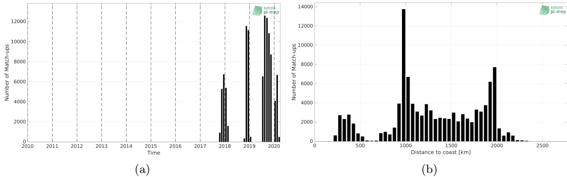
Figure 1: Number of match-ups between Saildrone and CCI SSS L4 Merged-OI v3.2 - 7-day running (ESA) SSS as a function of time (a) and as function of the distance to coast (b) over the Equatorial Ocean 10N-10S Pi-MEP region and for the full satellite product period.
