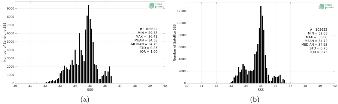
Figure 2: Histograms of SSS from Saildrone (a) and CCI SSS L4 Merged-OI v3.2 - 7-day running (ESA) (b) considering all match-up pairs per bins of 0.1 over the Equatorial Ocean 10N-10S Pi-MEP region and for the full satellite product period.
