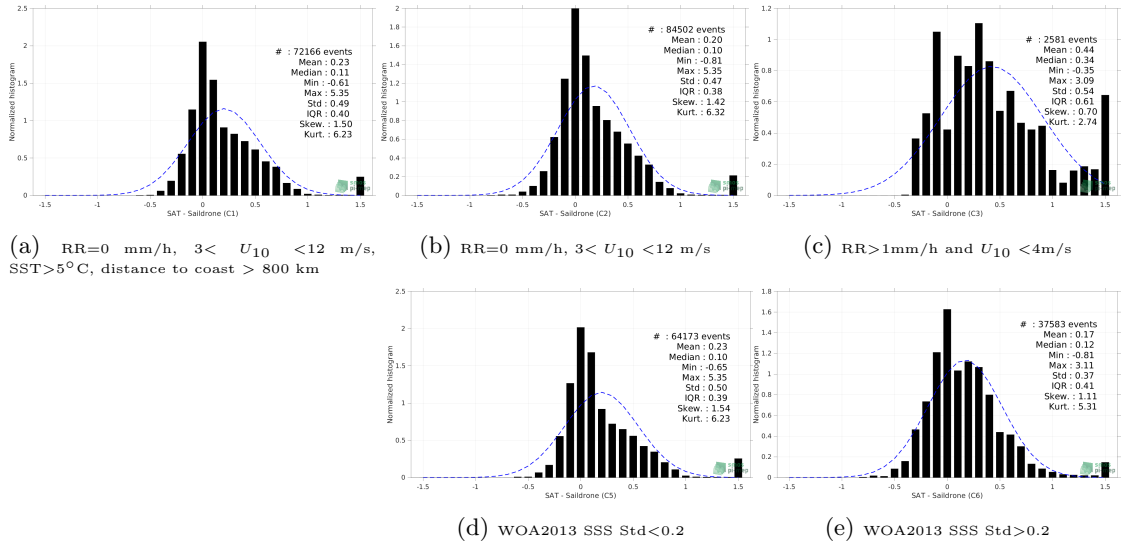
Figure 13: Normalized histogram of \Delta SSS (CCI SSS L4 Merged-OI v3.2 - 7-day running (ESA) - Saildrone) for 5 different subdatasets corresponding to: RR=0 mm/h, 3 < U_{10} < 12 m/s, SST >5^\circ\text{C} , distance to coast > 800 km (a), RR=0 mm/h, 3 < U_{10} < 12 m/s (b), RR >1 mm/h and U_{10} < 4 m/s (c), WOA2013 SSS Std <0.2 (d), WOA2013 SSS Std >0.2 (e).
