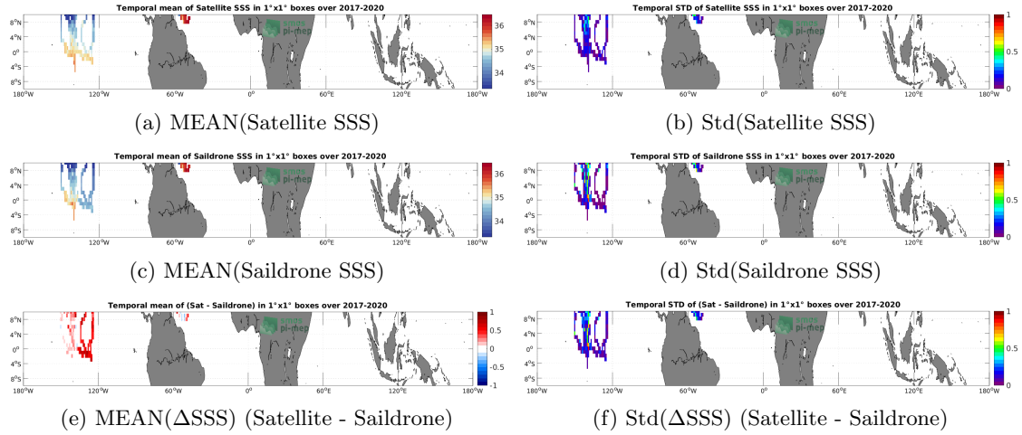
Figure 6: Temporal mean (left) and Std (right) of SSS from CCI SSS L4 Merged-OI v3.2 - 7-day running (ESA) (top), Saildrone (middle), and of \Delta SSS (Satellite - Saildrone). Only match-up pairs are used to generate these maps.
