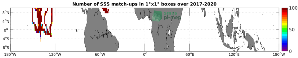
Figure 4: Number of SSS match-ups between Saildrone SSS and the CCI SSS L4 Merged-OI v3.2 - 7-day running (ESA) SSS product for the Equatorial Ocean 10N-10S Pi-MEP region over 1^\circ \times 1^\circ boxes and for the full satellite product period.
