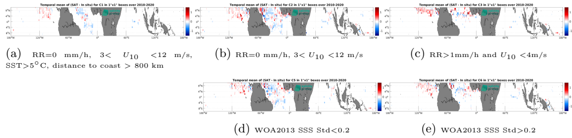
Figure 11: Temporal mean gridded over spatial boxes of size 1^\circ \times 1^\circ of \Delta\text{SSS} (CCI SSS L4 Merged-OI v3.2 - 7-day running (ESA) - Surface drifters) for 5 different subdatasets corresponding to:RR=0 mm/h, 3 < U_{10} < 12 m/s, SST >5^\circ\text{C} , distance to coast > 800 km (a), RR=0 mm/h, 3 < U_{10} < 12 m/s (b), RR >1 mm/h and U_{10} < 4 m/s (c), WOA2013 SSS Std <0.2 (d), WOA2013 SSS Std >0.2 (e).
